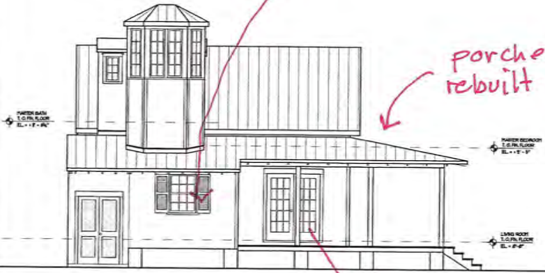
EXISTING SIDE ELEVATION SCALE 1/4" = 1'-0"
