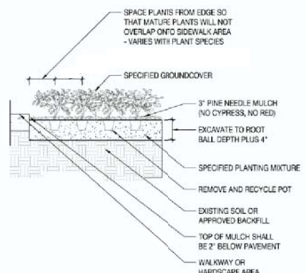
5 GROUND COVER PLANTING DETAIL
