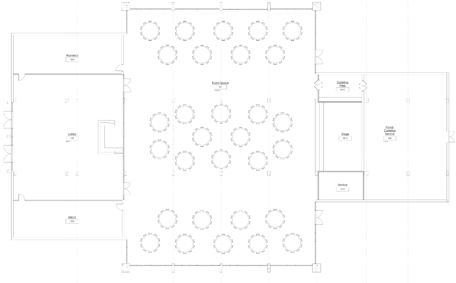
ARCHITECTURAL FIRST FLOOR PLAN 1/8" = 1'-0"
