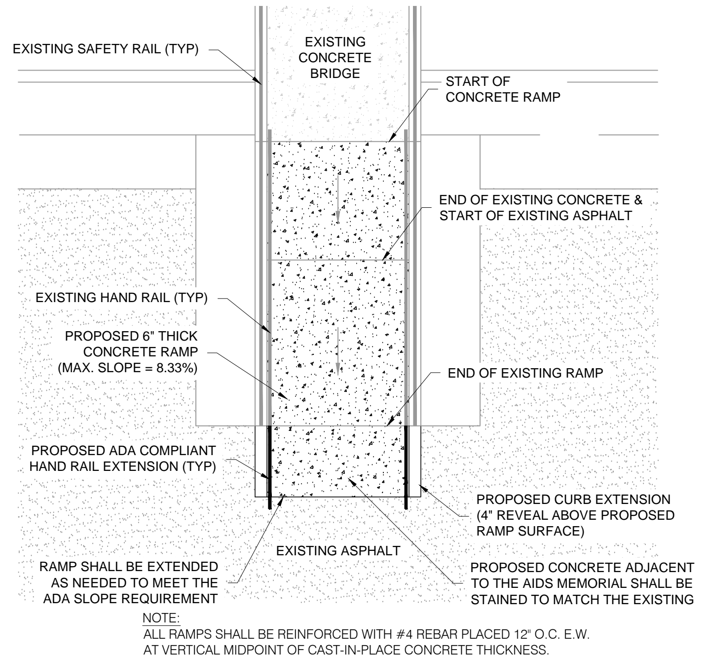
TYPICAL RAMP LAYOUT NTS
