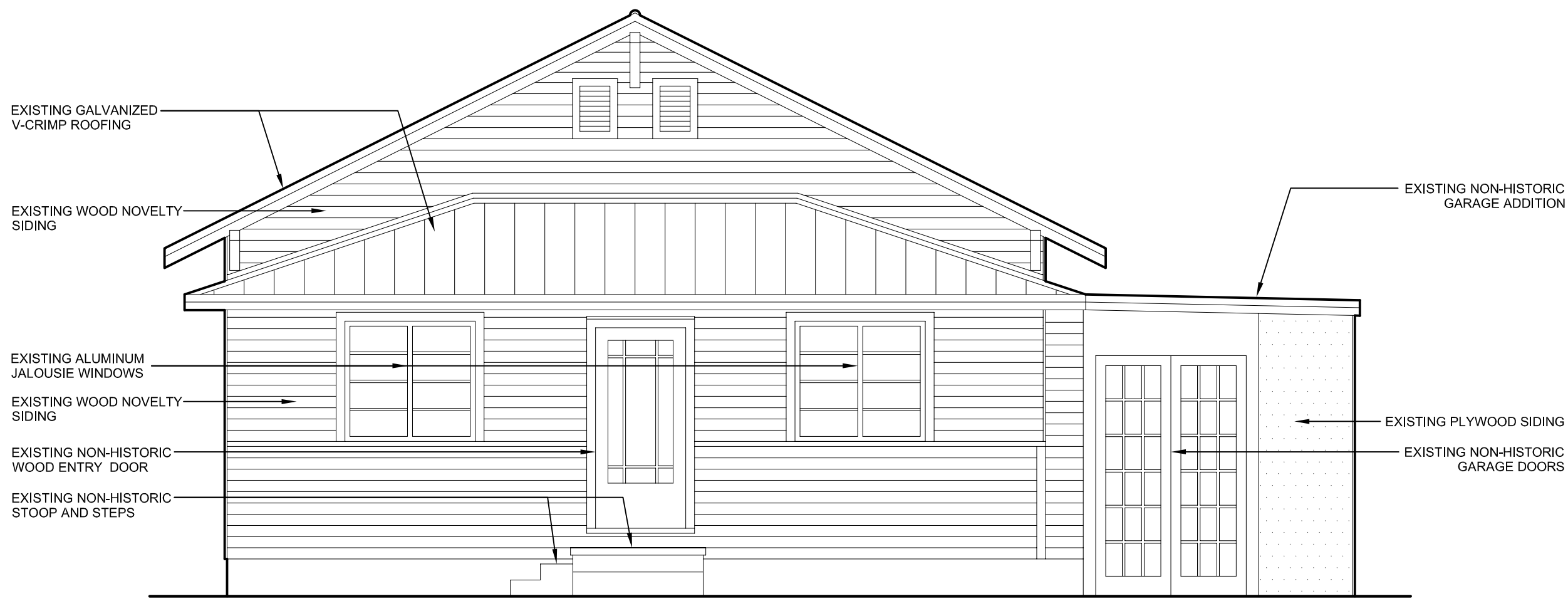
STREET (NORTH) ELEVATION
