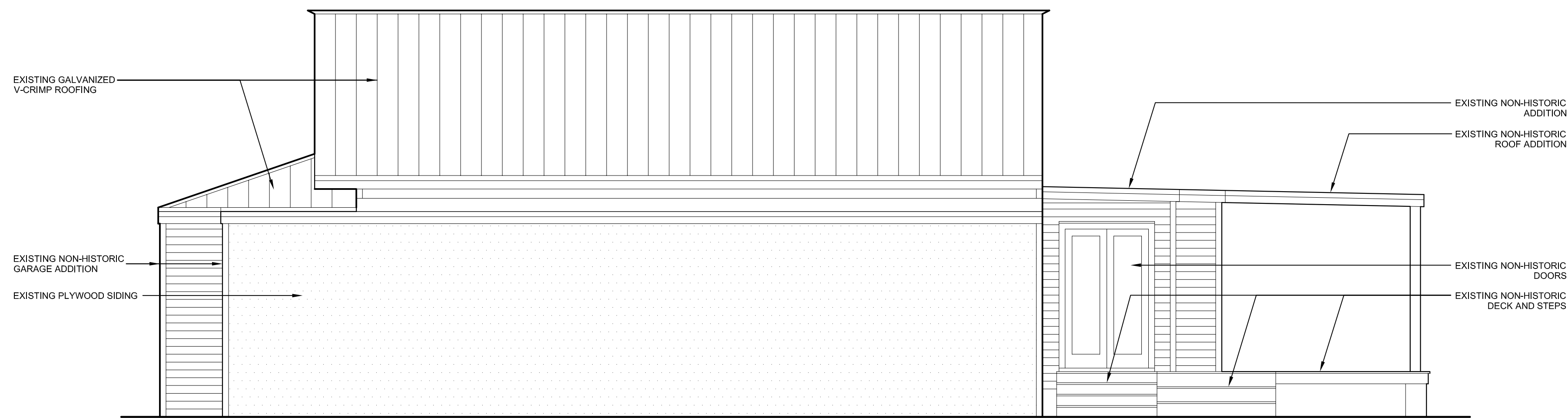
WEST ELEVATION
