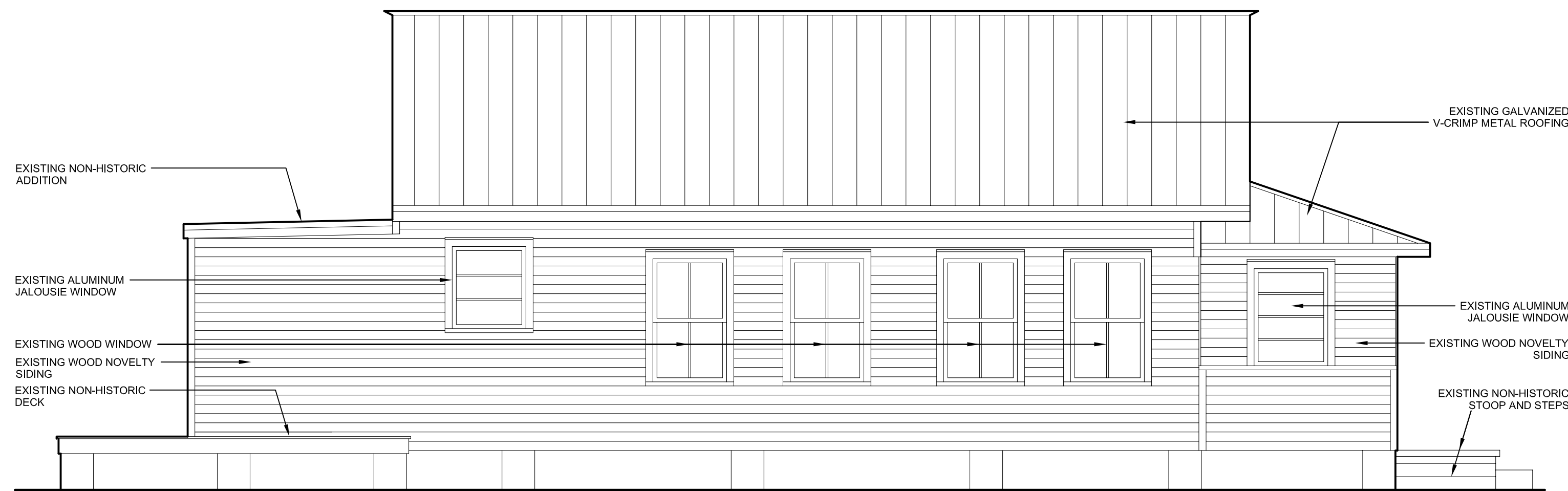
EAST ELEVATION
