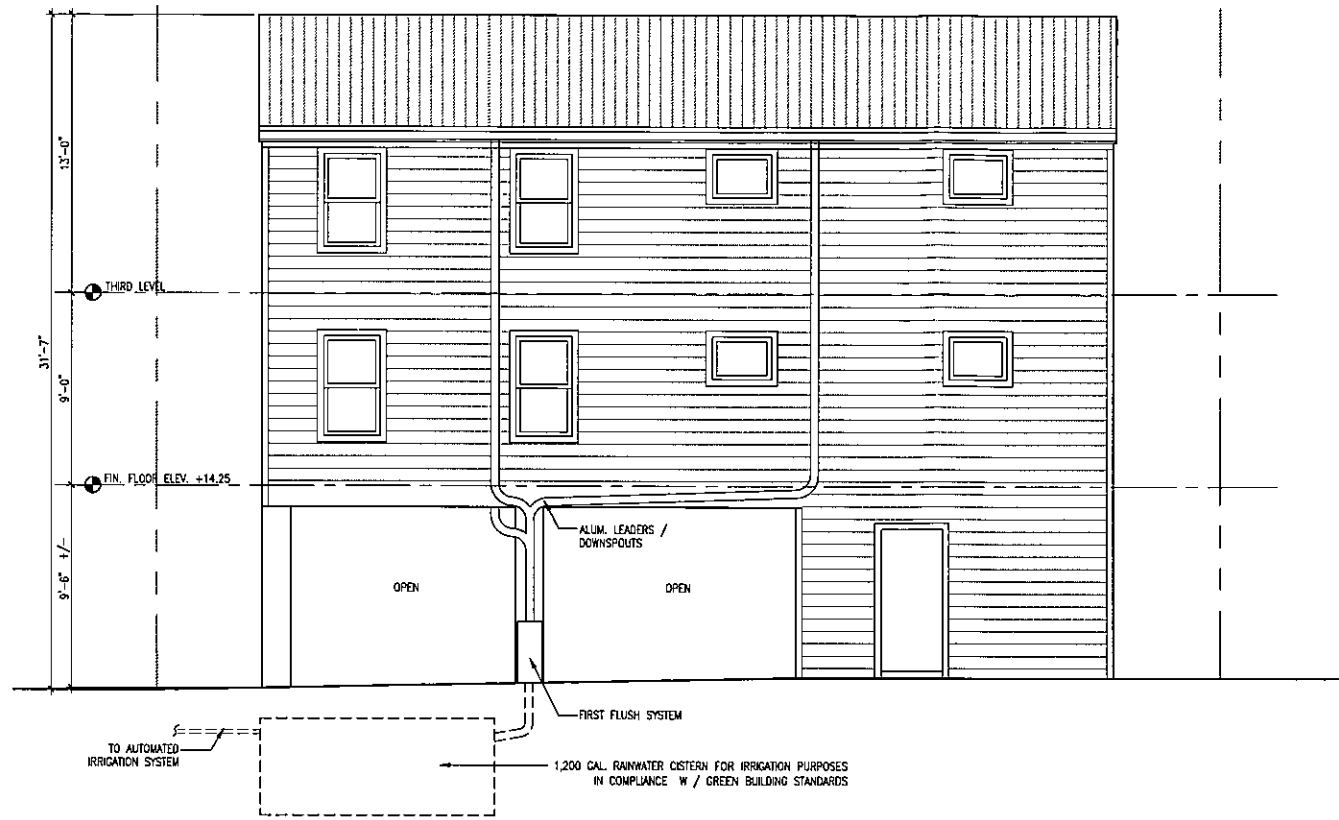
2 A3.1 WEST ELEVATION SCALE: 1/4"=1'-0"
