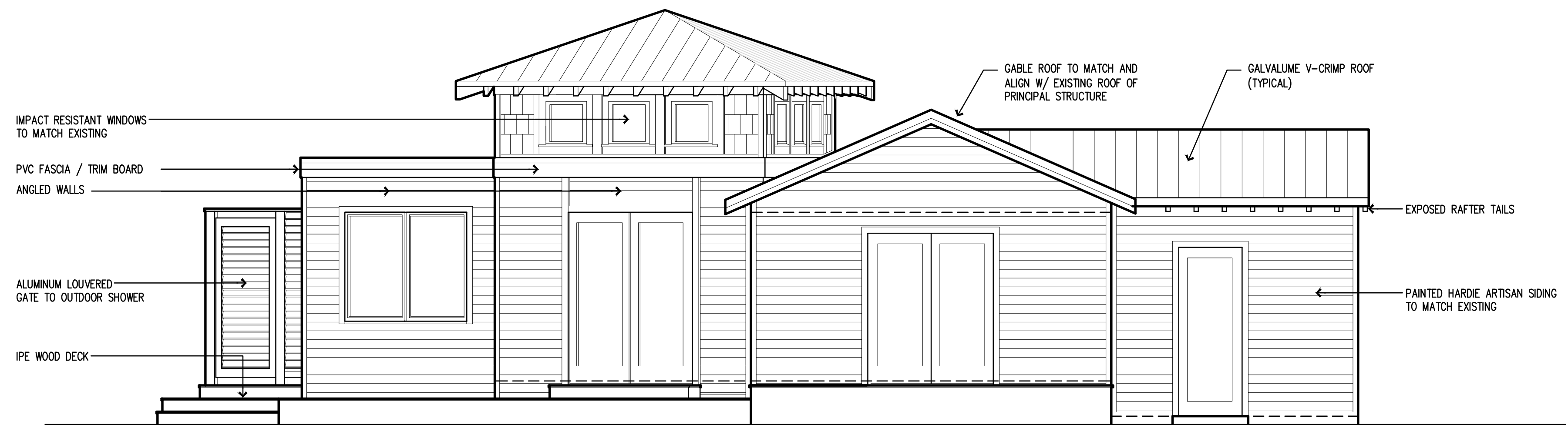
SOUTH SIDE ELEVATION 1/4"=1'-0"
