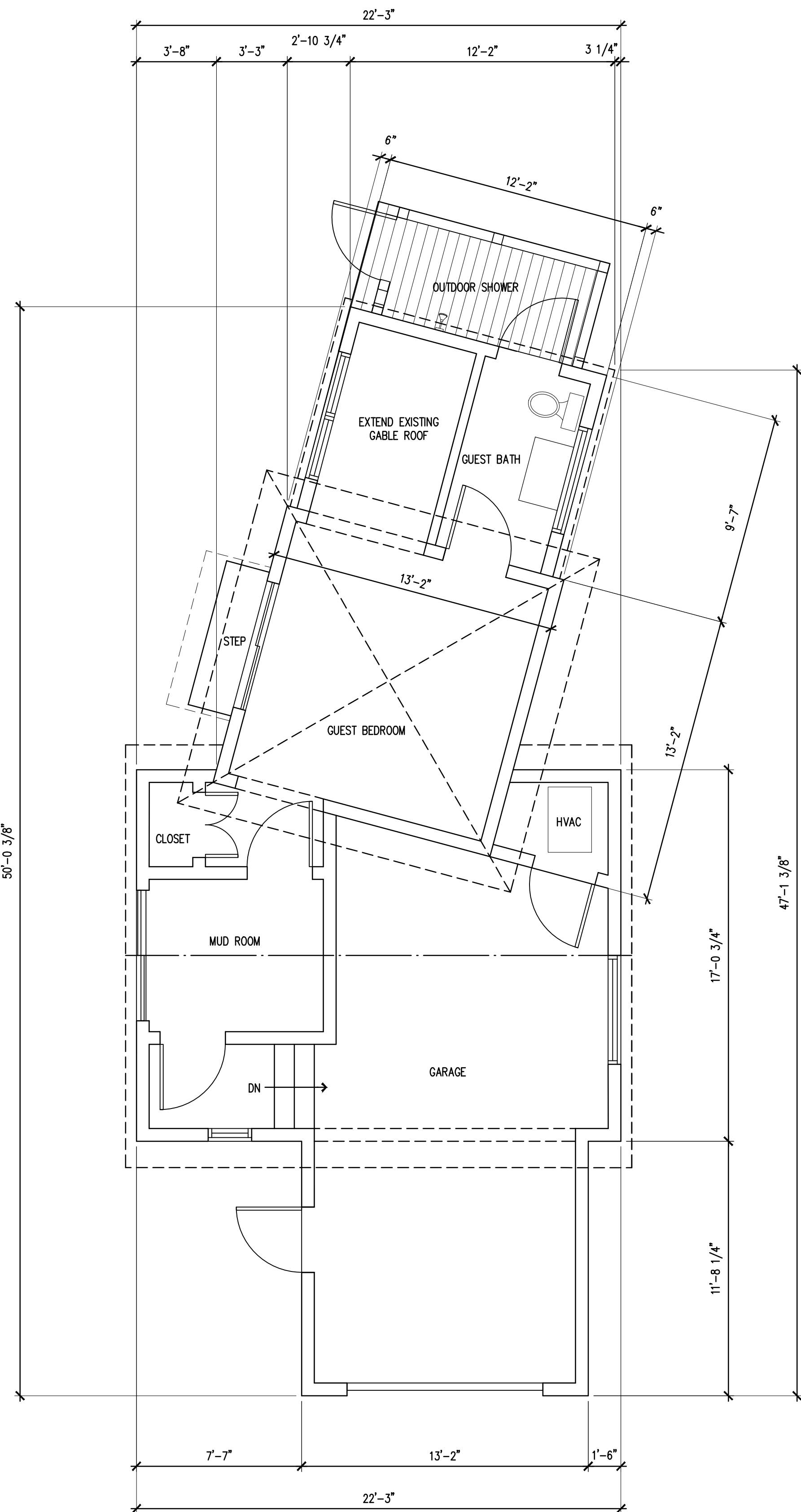
ENLARGED FLOOR PLAN 1/4"=1'-0"
