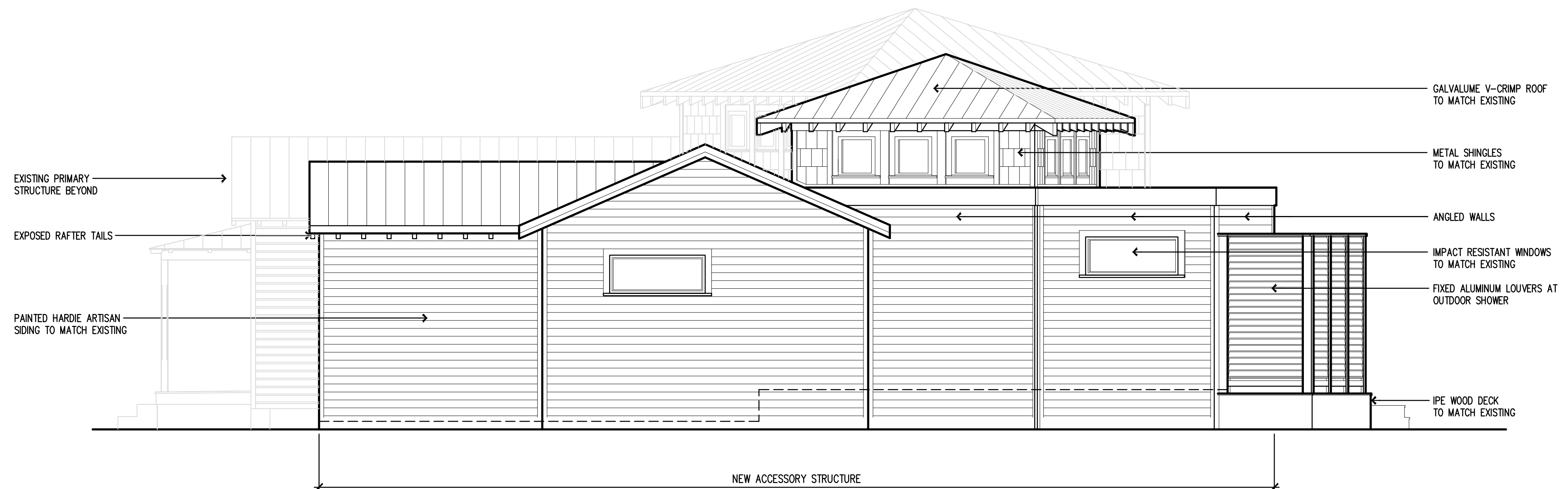
NORTH SIDE ELEVATION 1/4"=1'-0"
