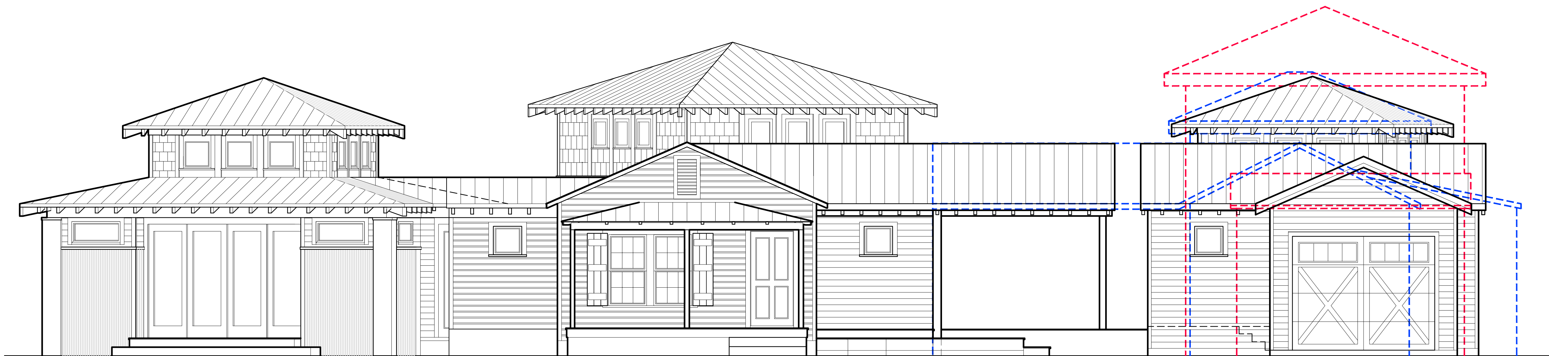
FRONT ELEVATION 1/4"=1'-0"
