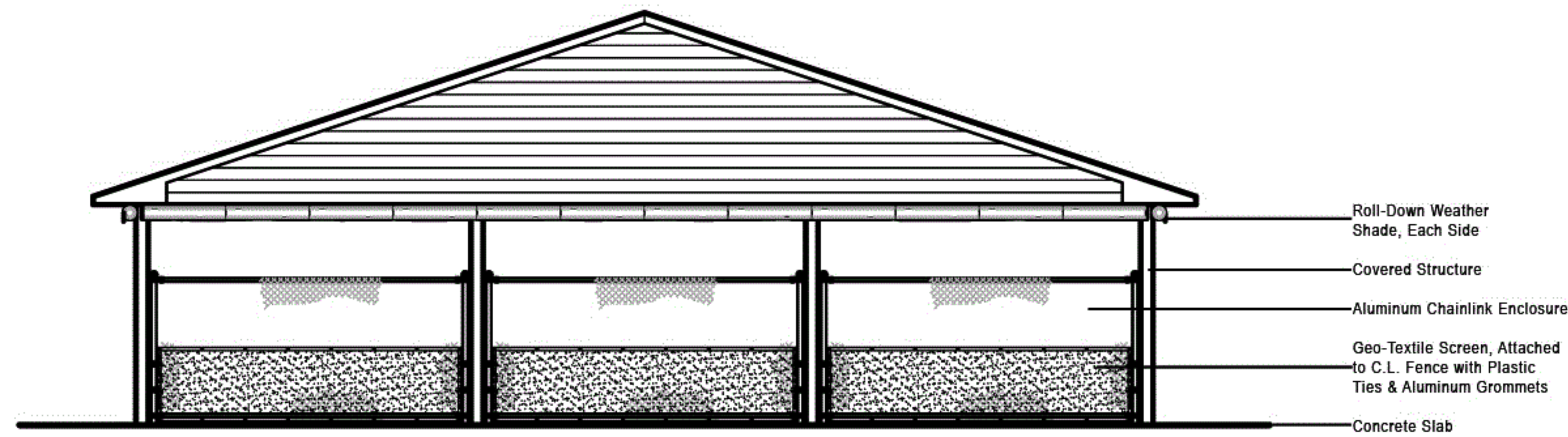
Men's Shelter- East / West Elevation
