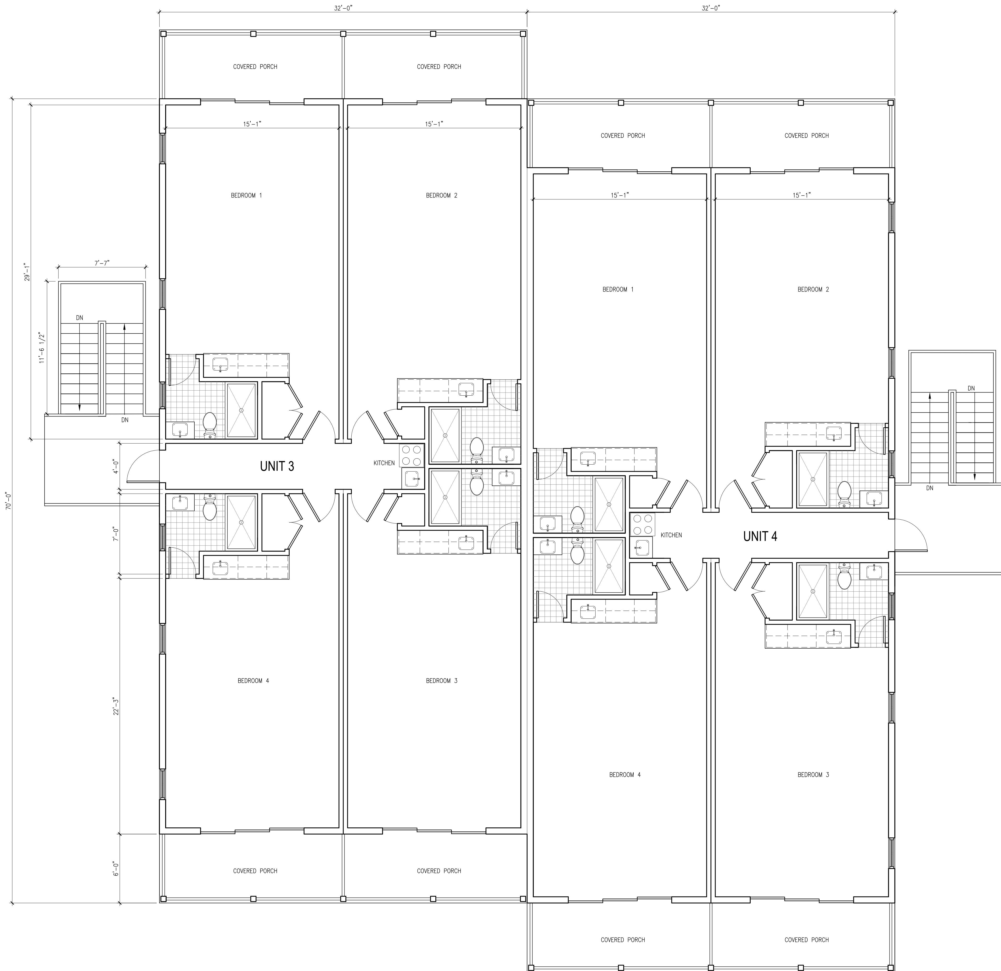
1 A2.2 TYPICAL SECOND FLOOR PLAN SCALE: 1/4"=1'-0"
