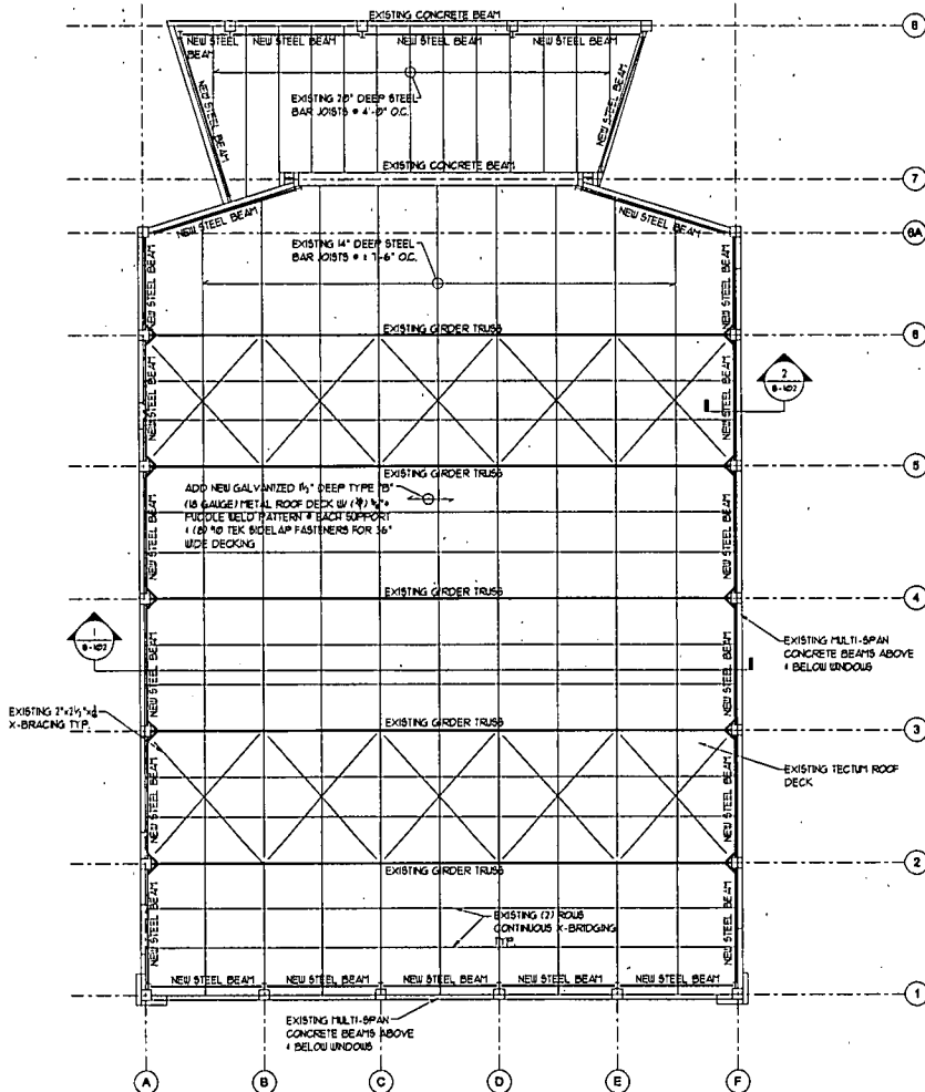
EXISTING ROOF FRAMING PLAN SCALE 1/8\"/>
