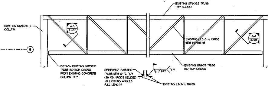
ADDITIONAL WEB REINFORCING EXISTING GIRDER TRUSS
