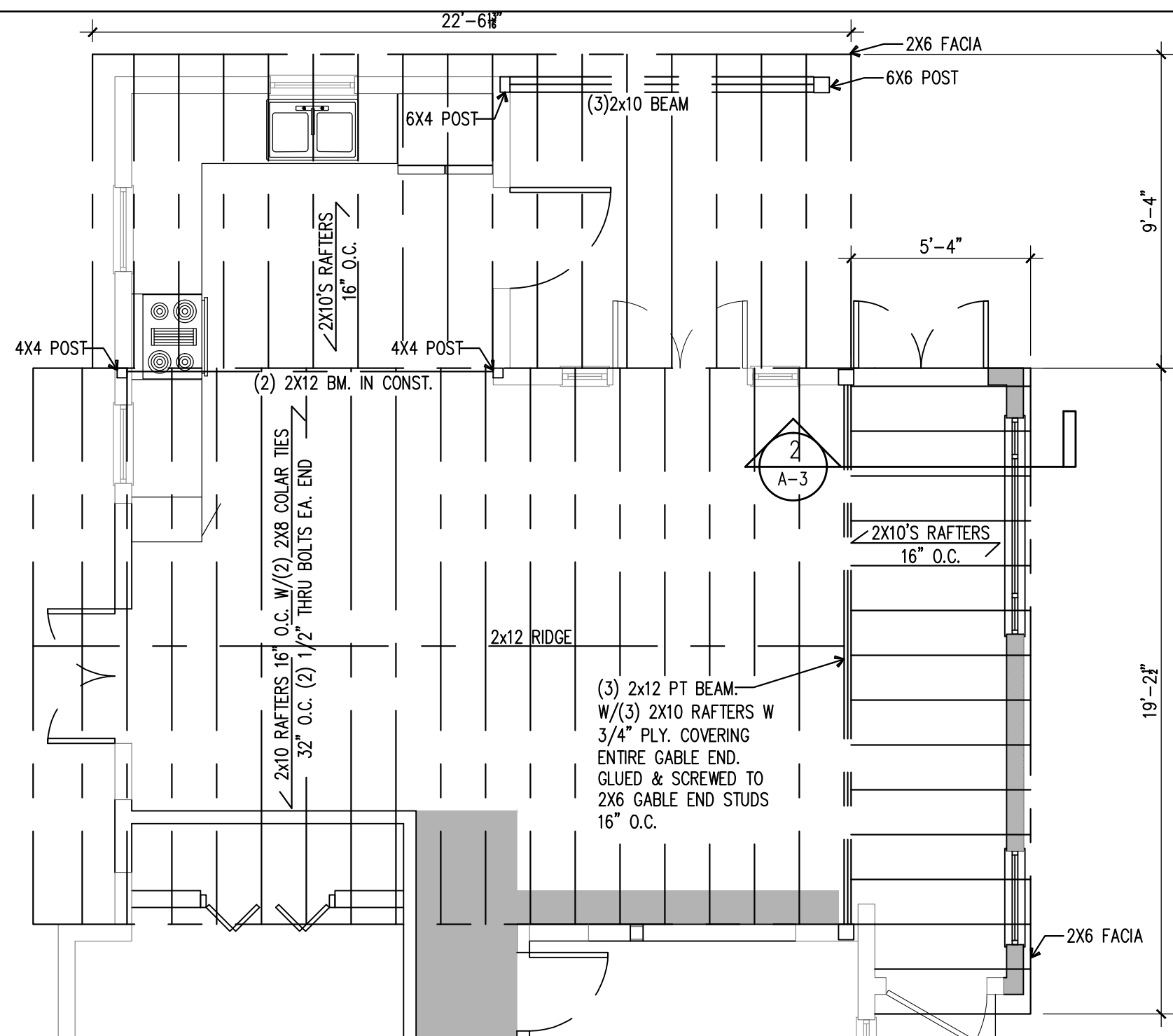
5 ROOF FRAMING PLAN SCALE: 1/4" = 1'-0"
