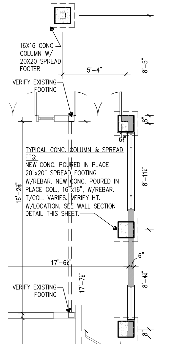
4 FOUNDATION PLAN SCALE: 1/4" = 1'-0"
