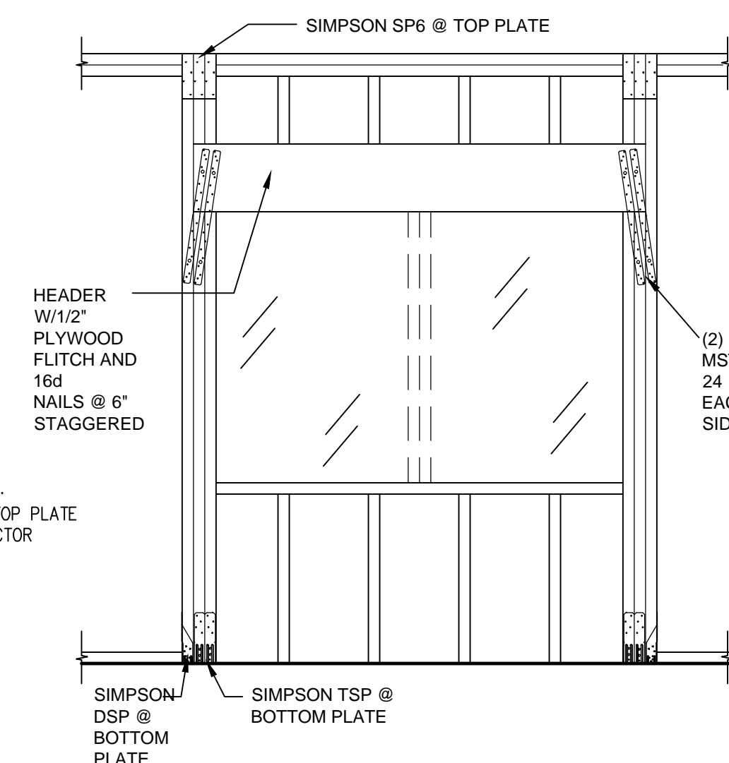
HEADER STRAP DETAIL
