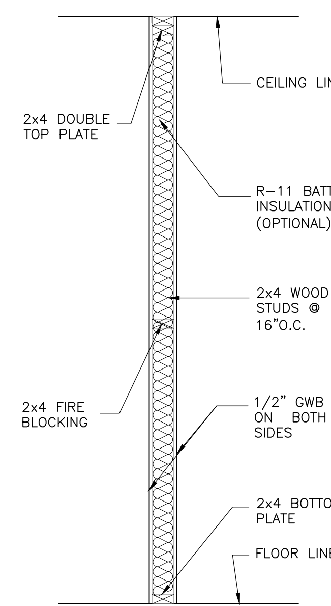
1 2X4 WALL DETAIL SCALE: 3/4" = 1'-0"
