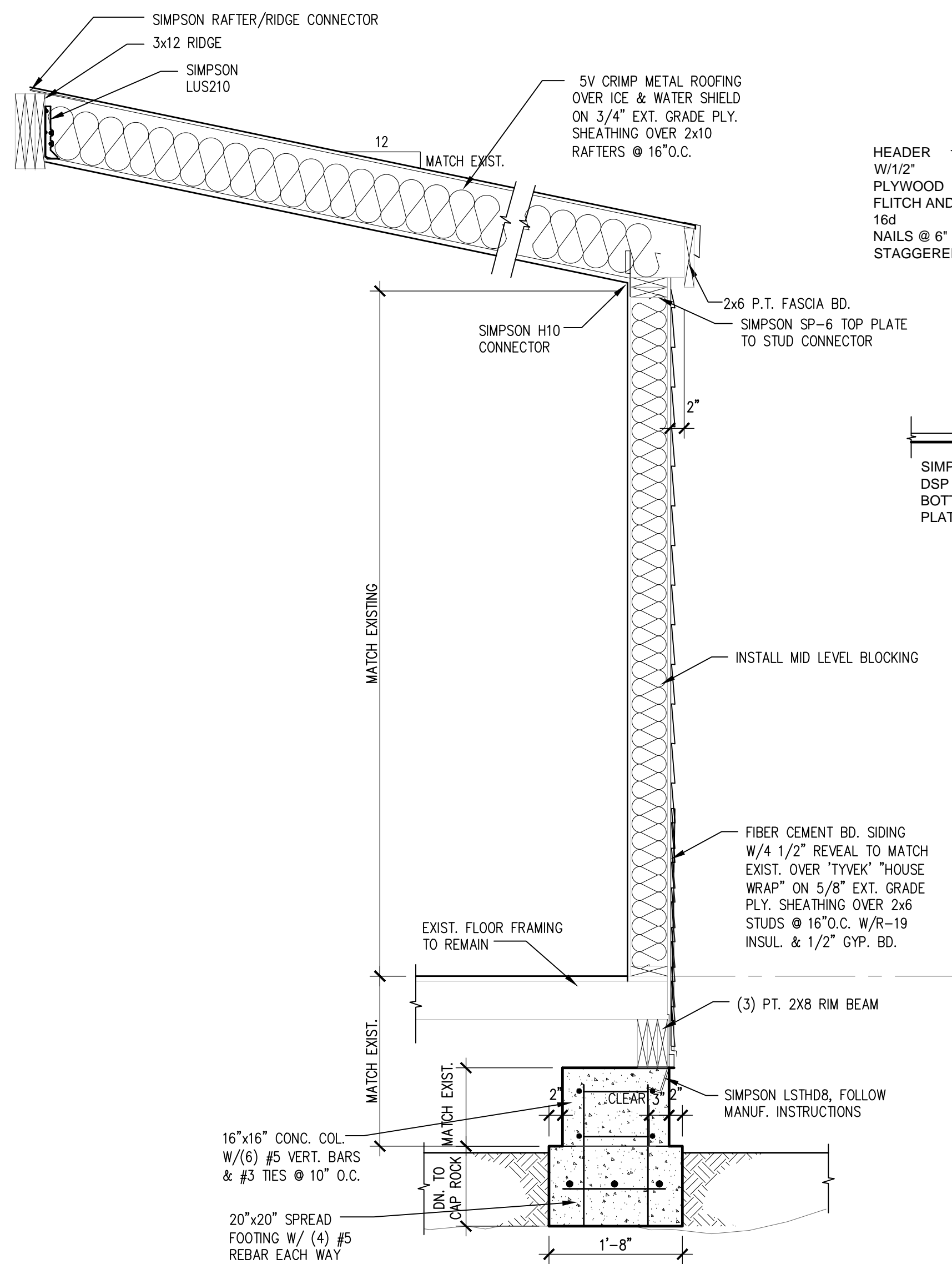
2 2X6 WALL DETAIL SCALE: 3/4" = 1'-0"
