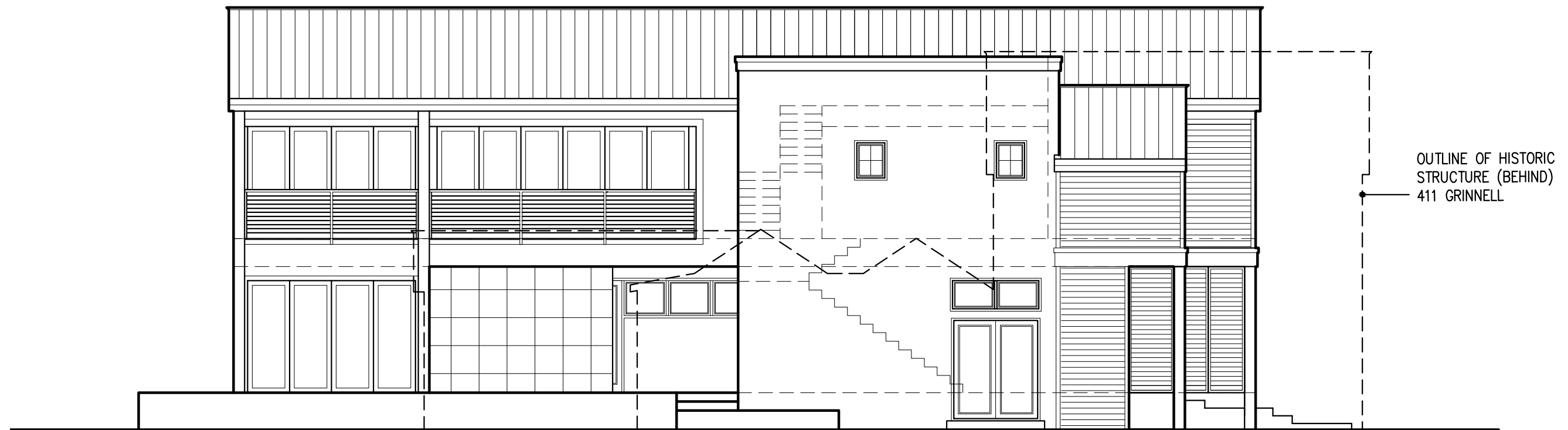
SIDE ELEVATION (NORTH) 1/8"=1'-0"
