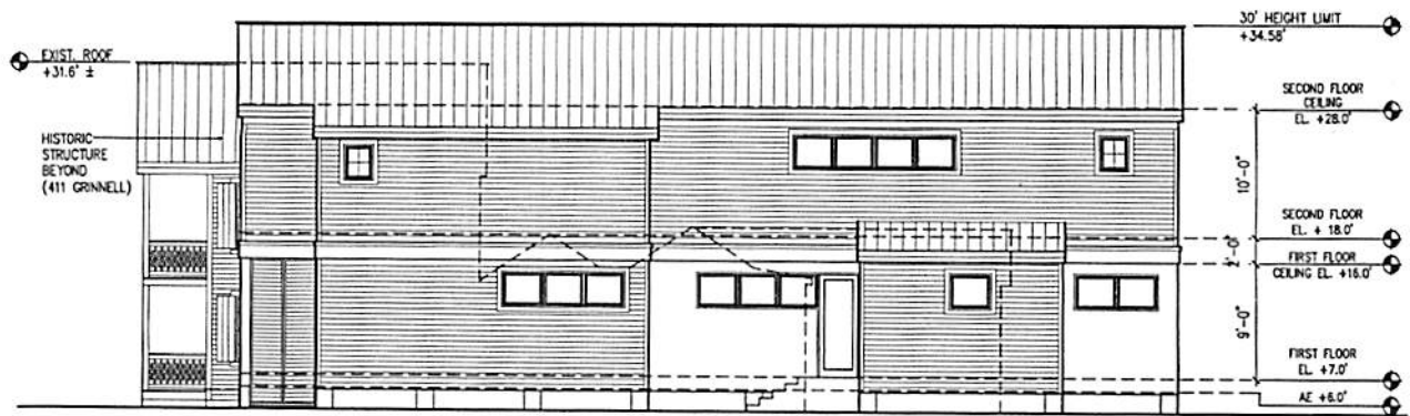
SIDE ELEVATION (SOUTH) 1/8"=1'-0"
