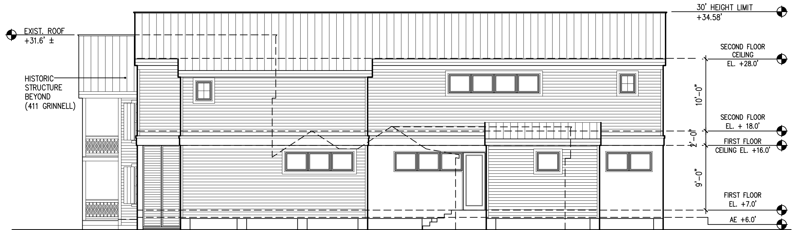
SIDE ELEVATION (SOUTH) 1/8"=1'-0"
