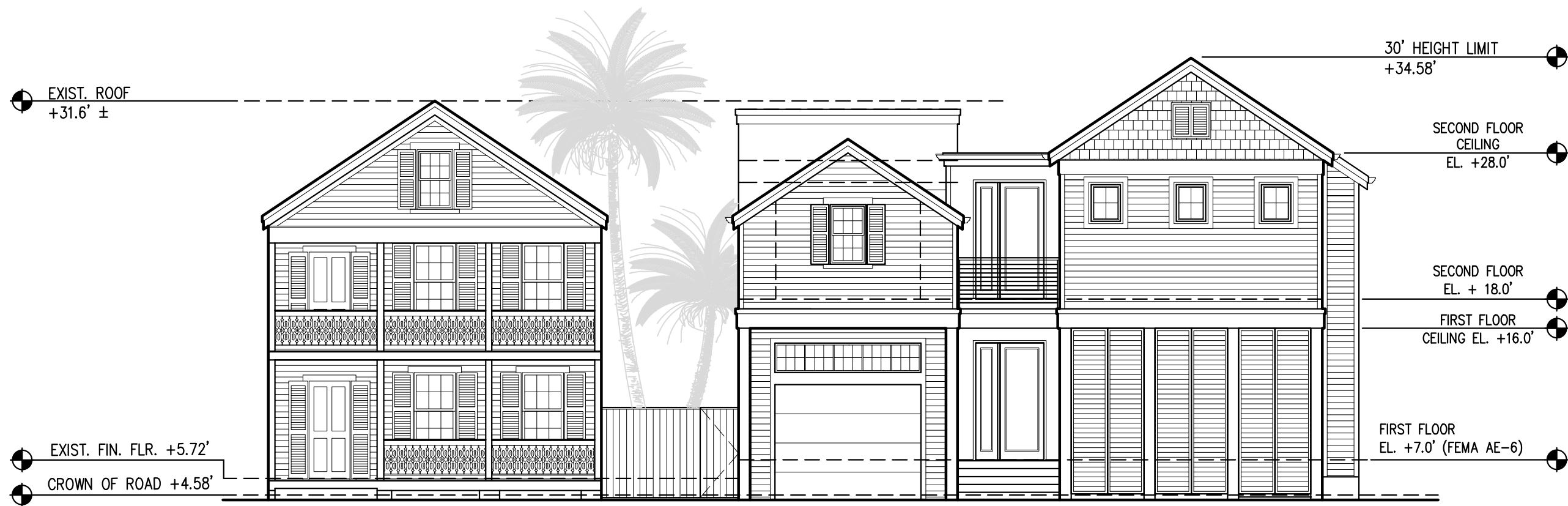
FRONT ELEVATION 1/8"=1'-0"
