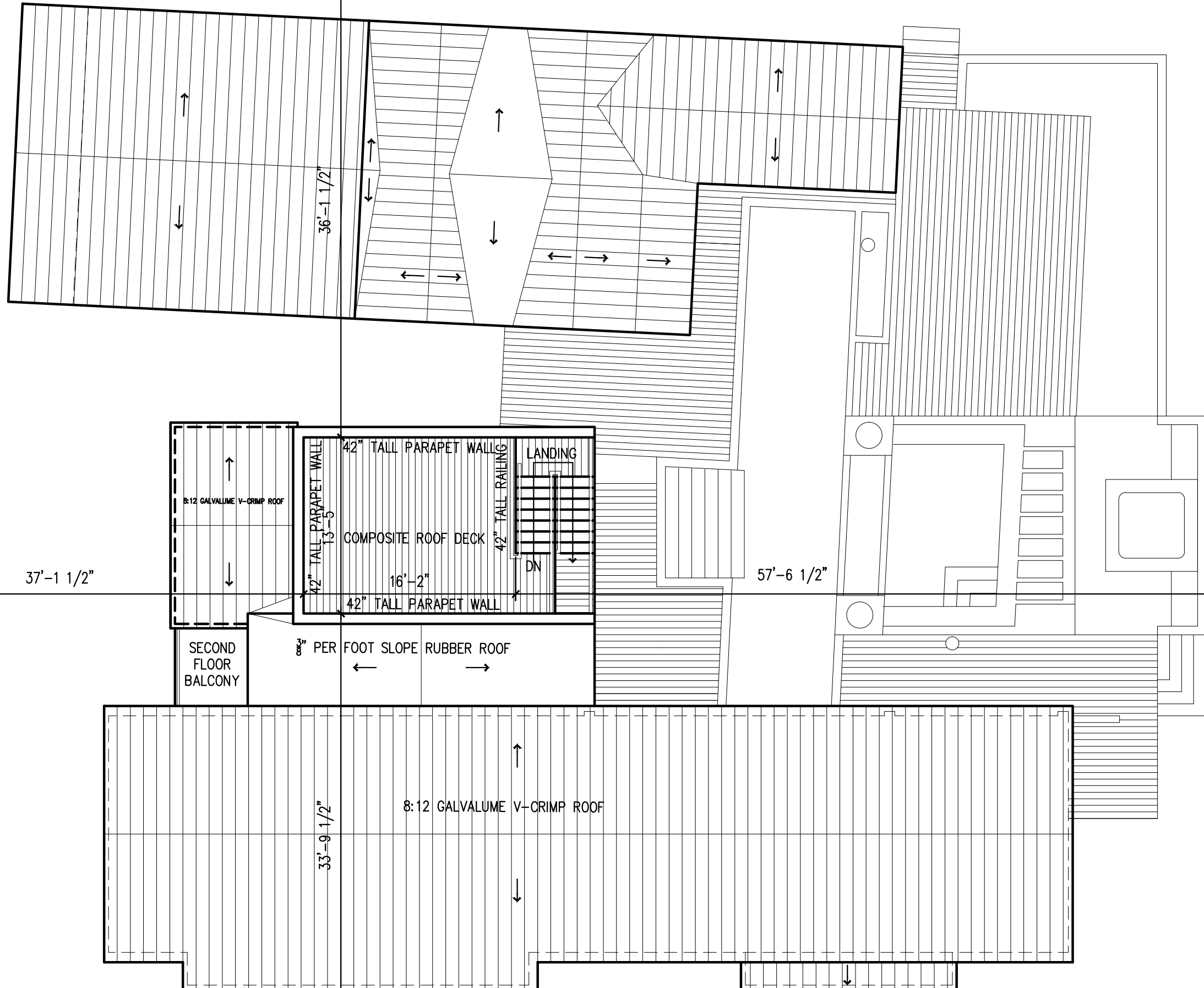
ROOF PLAN 1/8"=1'-0"
