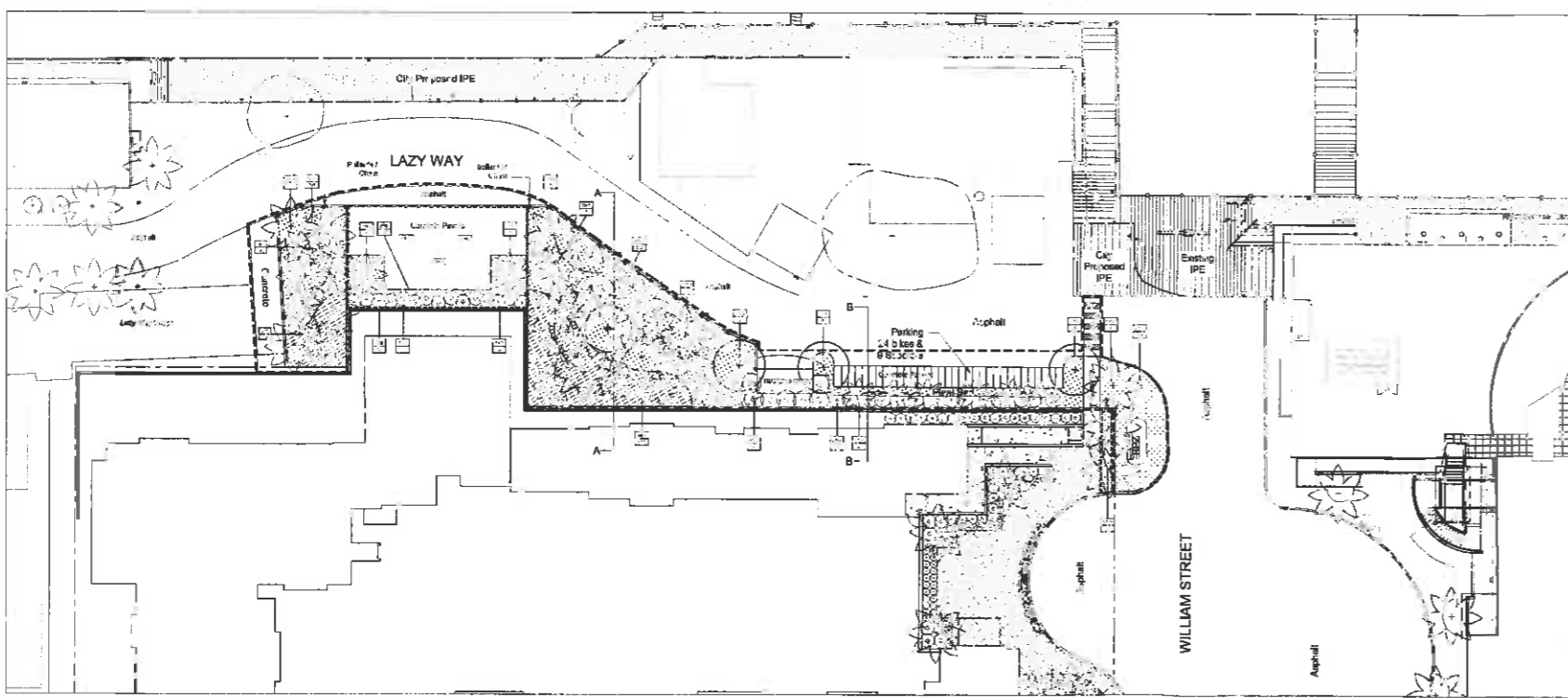
7 LANDSCAPE PLAN SCALE 1"=20'-0"
