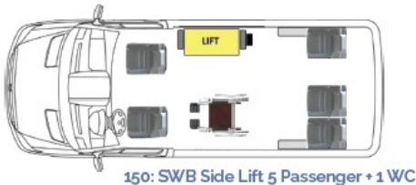
150: SWB Side Lift 5 Passenger + 1 WC
