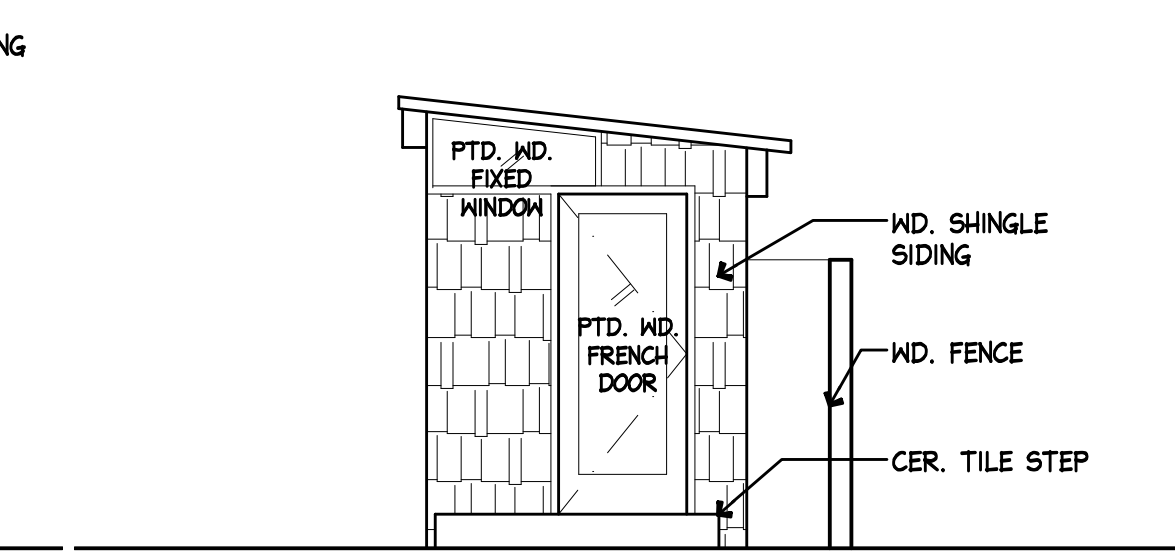
5 SHED WEST EXTERIOR ELEVATION EX2 SCALE: 1/4"=1'-0"
