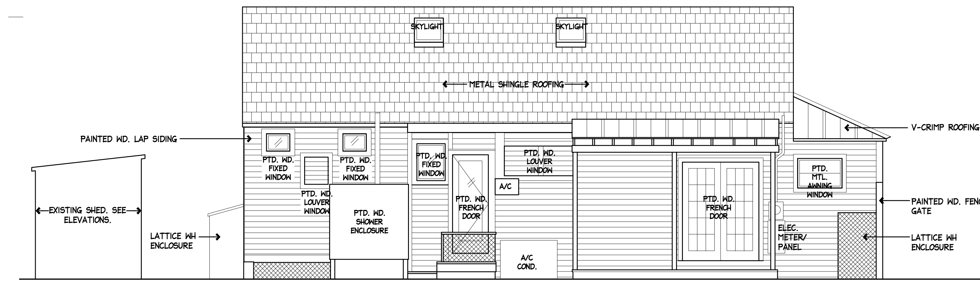
2 EXISTING SIDE (EAST) EXTERIOR ELEVATION EX2 SCALE: 1/4"=1'-0"
