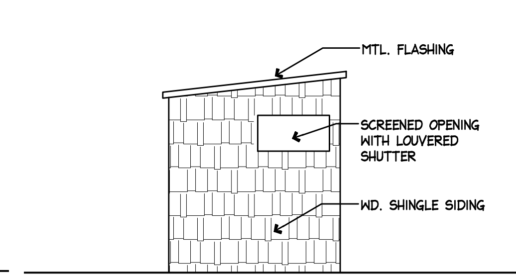
7 SHED EAST EXTERIOR ELEVATION EX2 SCALE: 1/4"=1'-0"
