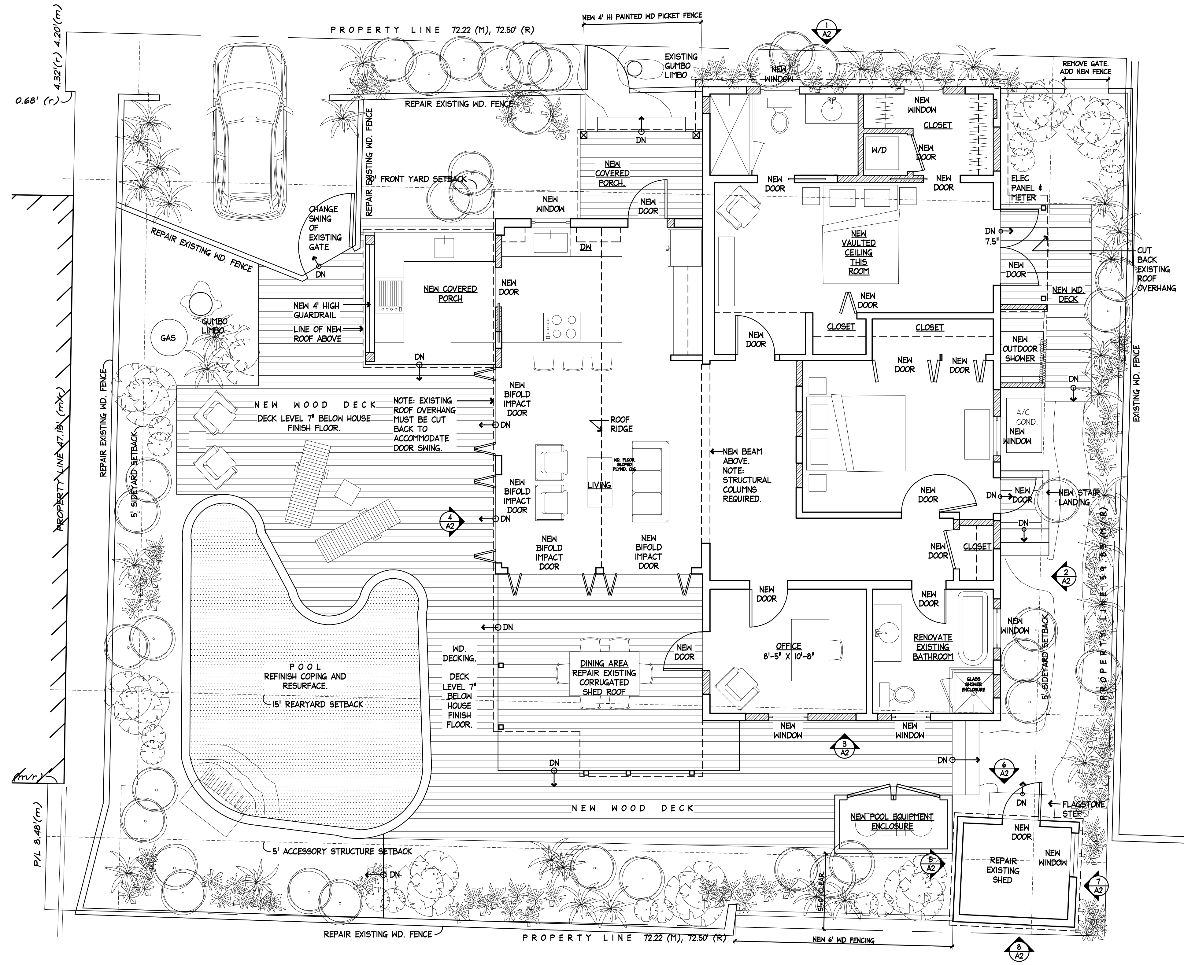
1 PROPOSED FIRST FLOOR PLAN A1 SCALE: 1/4"=1'-0"
