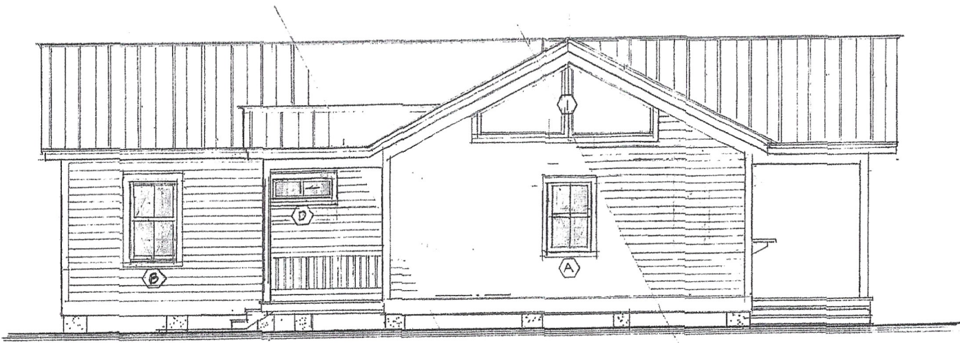
SOUTH ELEVATION
