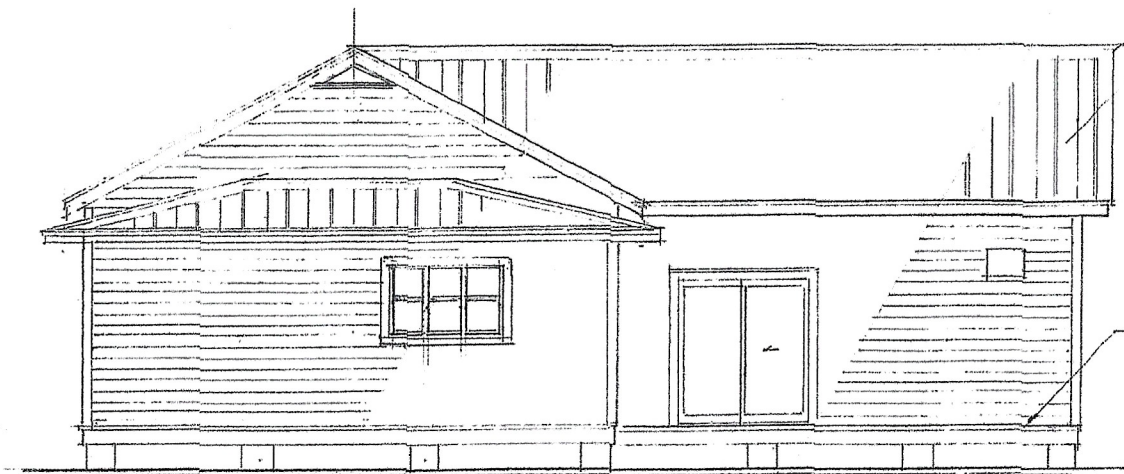
NORTH ELEVATION
