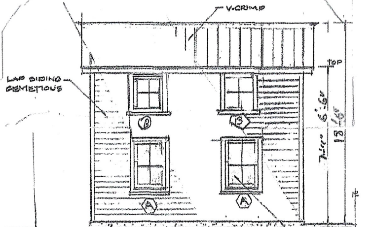
SOUTH ELEVATION SCALE 3/16" = 1'-0"
