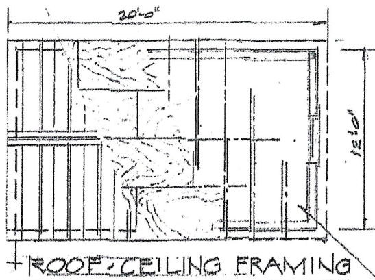
ROOF/CEILING FRAMING SCALE 3/16" = 1'-0"
