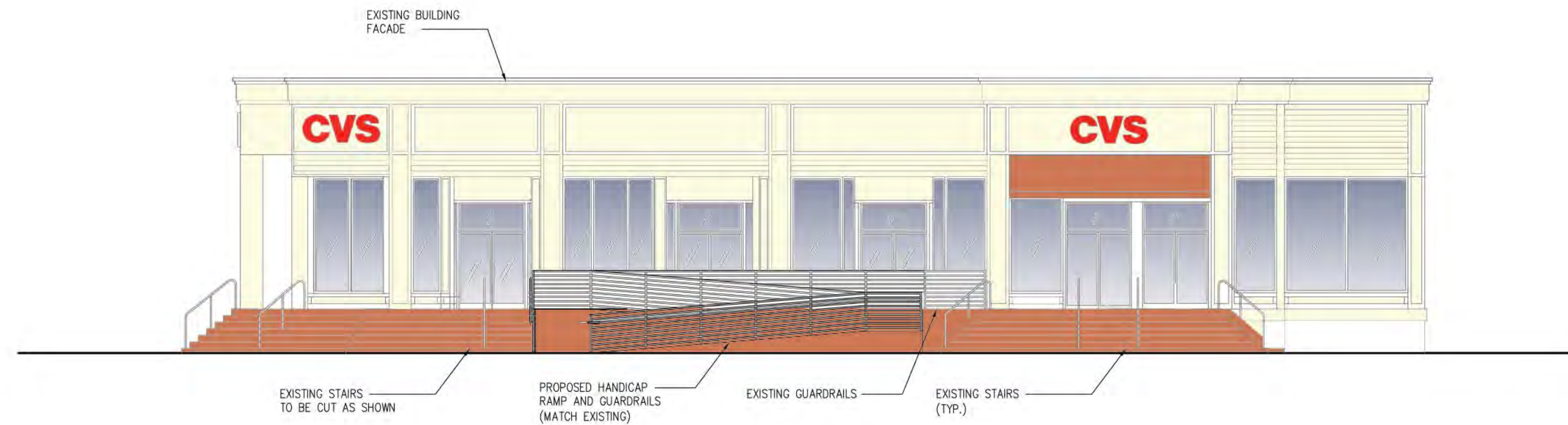
1 SOUTH ELEVATION A-4.0 SCALE: 3/32" = 1'-0"
