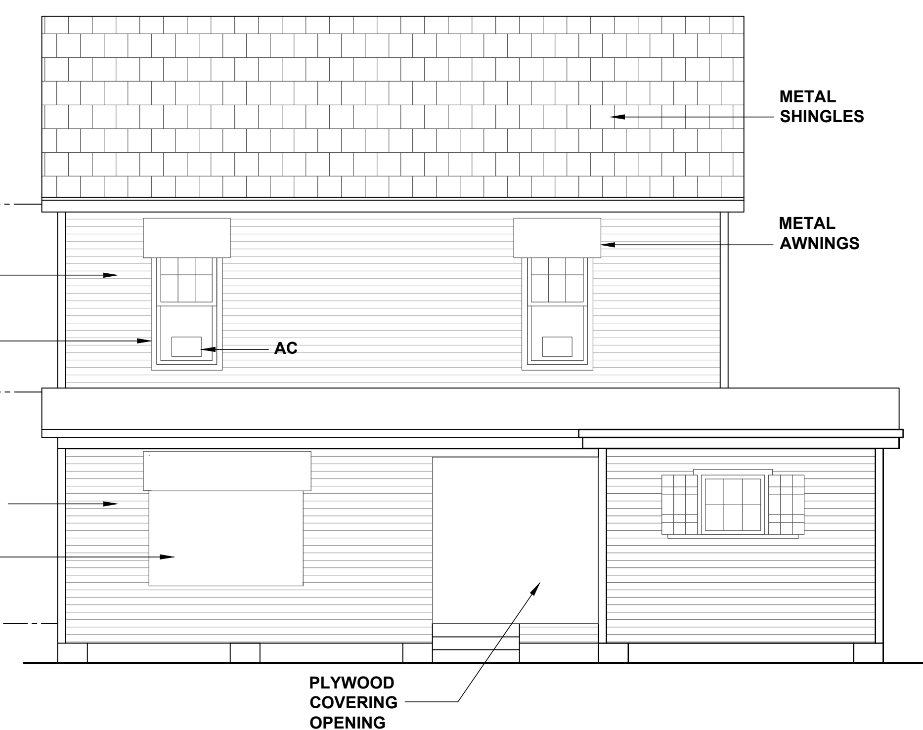
4 EXISTING REAR (WEST) ELEVATION A5 SCALE 1/4" = 1'-0"
