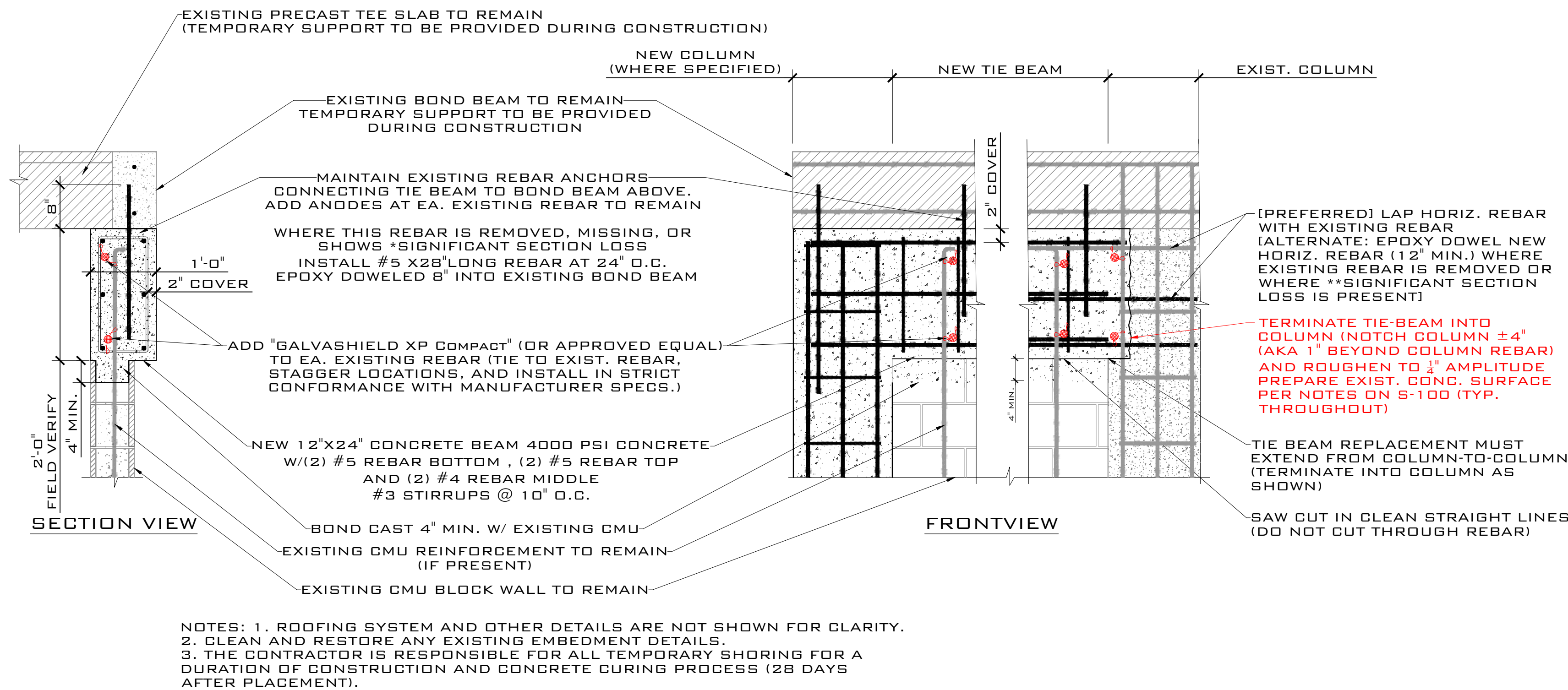
TYP. DETAIL 3/S-104 FULL SECTION - TIE BEAM REPAIR AT ROOF SCALE: N.T.S.
