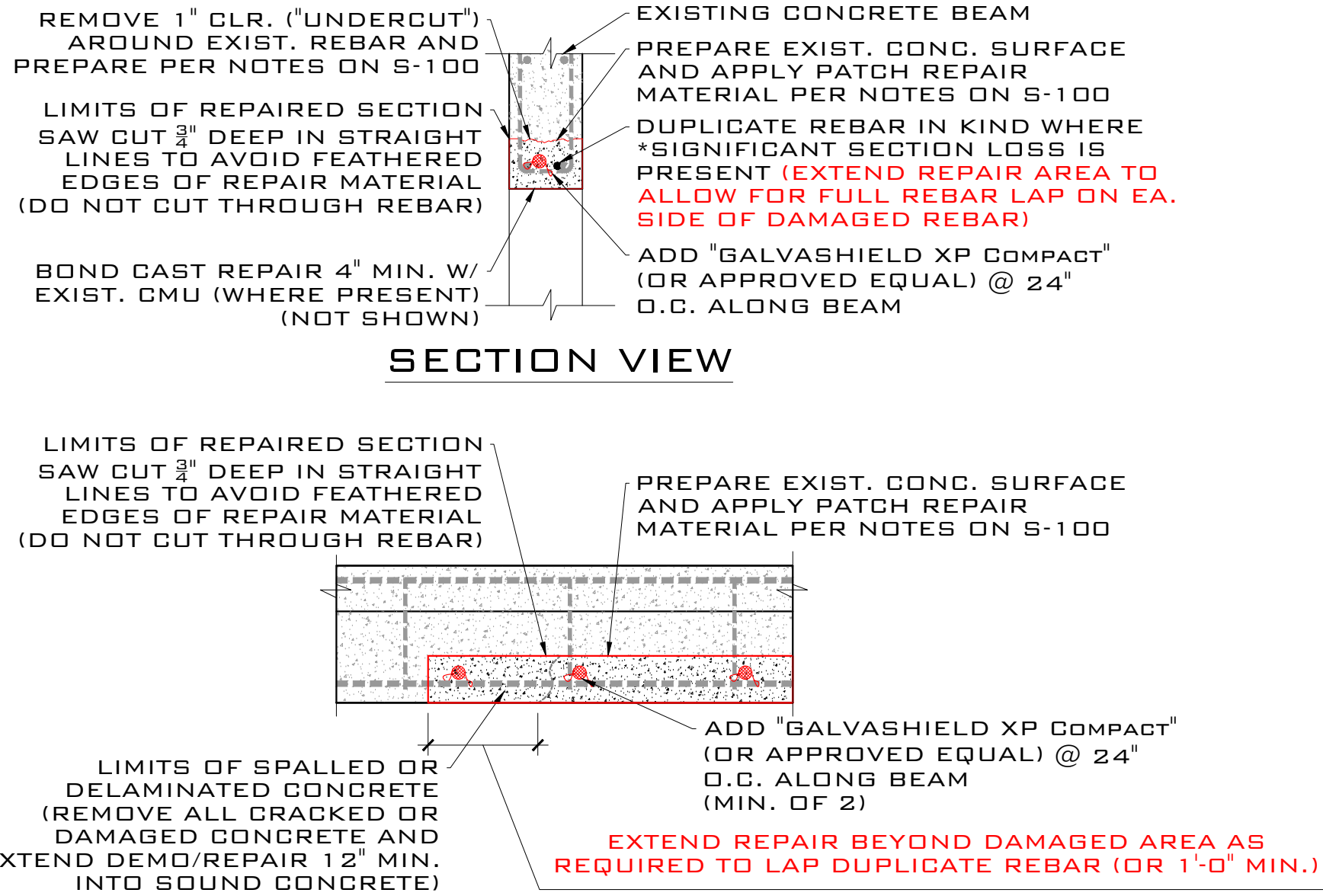
TYP. DETAIL 2/S-105 PARTIAL SECTION - BEAM/HEADER REPAIR SCALE: N.T.S.
