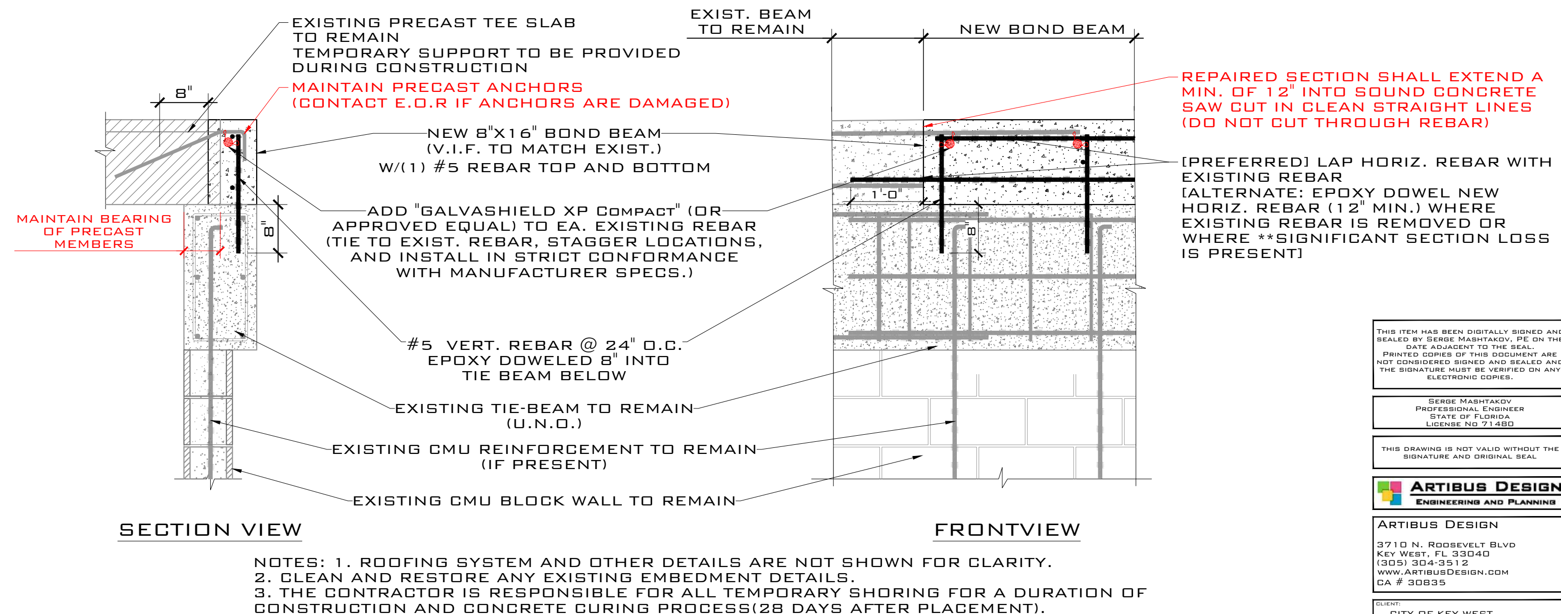
TYP. DETAIL 4/S-104 FULL SECTION - BOND BEAM REPAIR AT ROOF SCALE: N.T.S.
