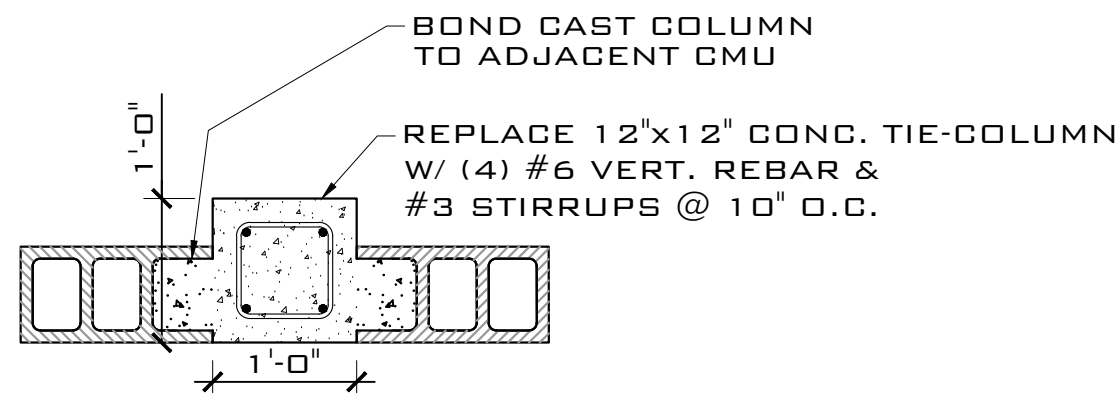
PLAN VIEW 12X12 TIE-COLUMN SCALE: NTS
