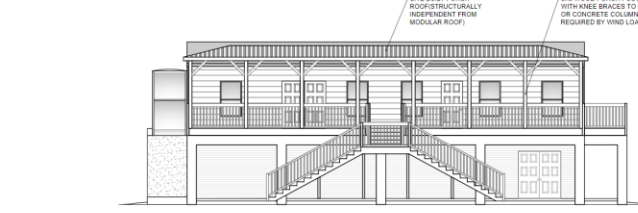
WEST ELEVATION - PROPOSED SCALE: 3/16"=1'-0"
