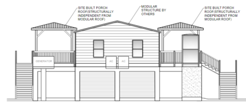
NORTH ELEVATION - PROPOSED SCALE: 3/16"=1'-0"
