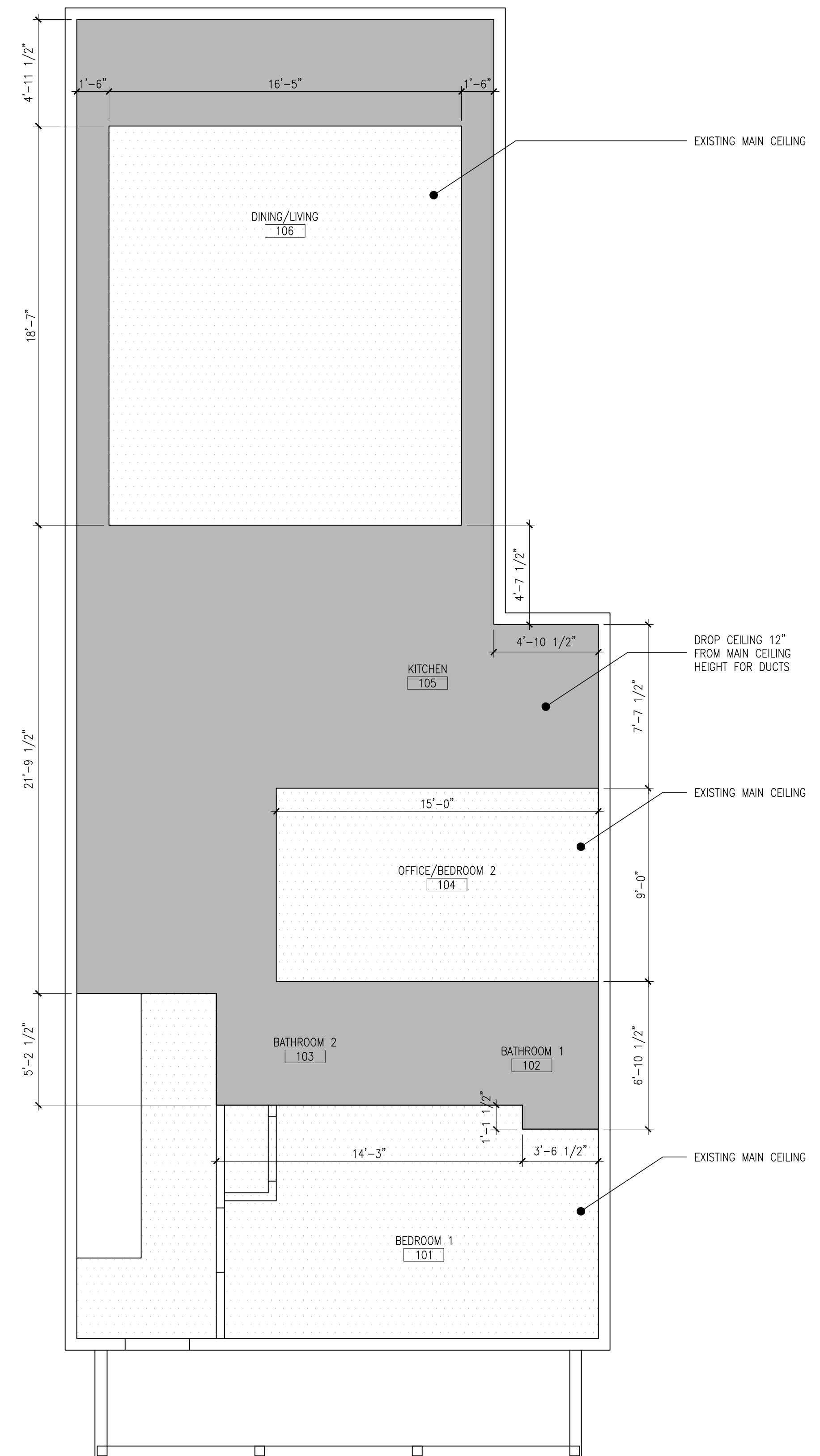
1 PROPOSED FIRST FLOOR RCP A4.1 SCALE: 1/4"=1'-0"
