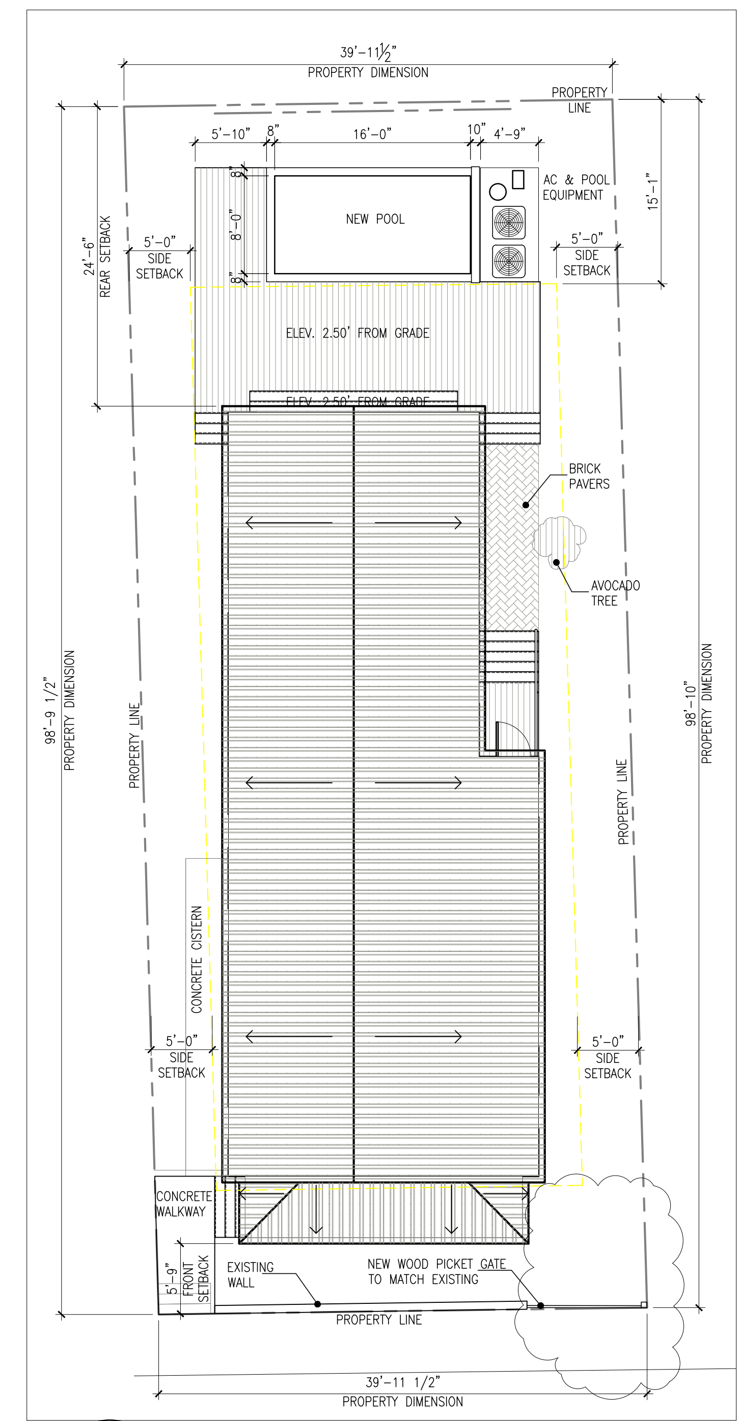
1 PROPOSED SITE PLAN SCALE: 1/8"=1'-0"
