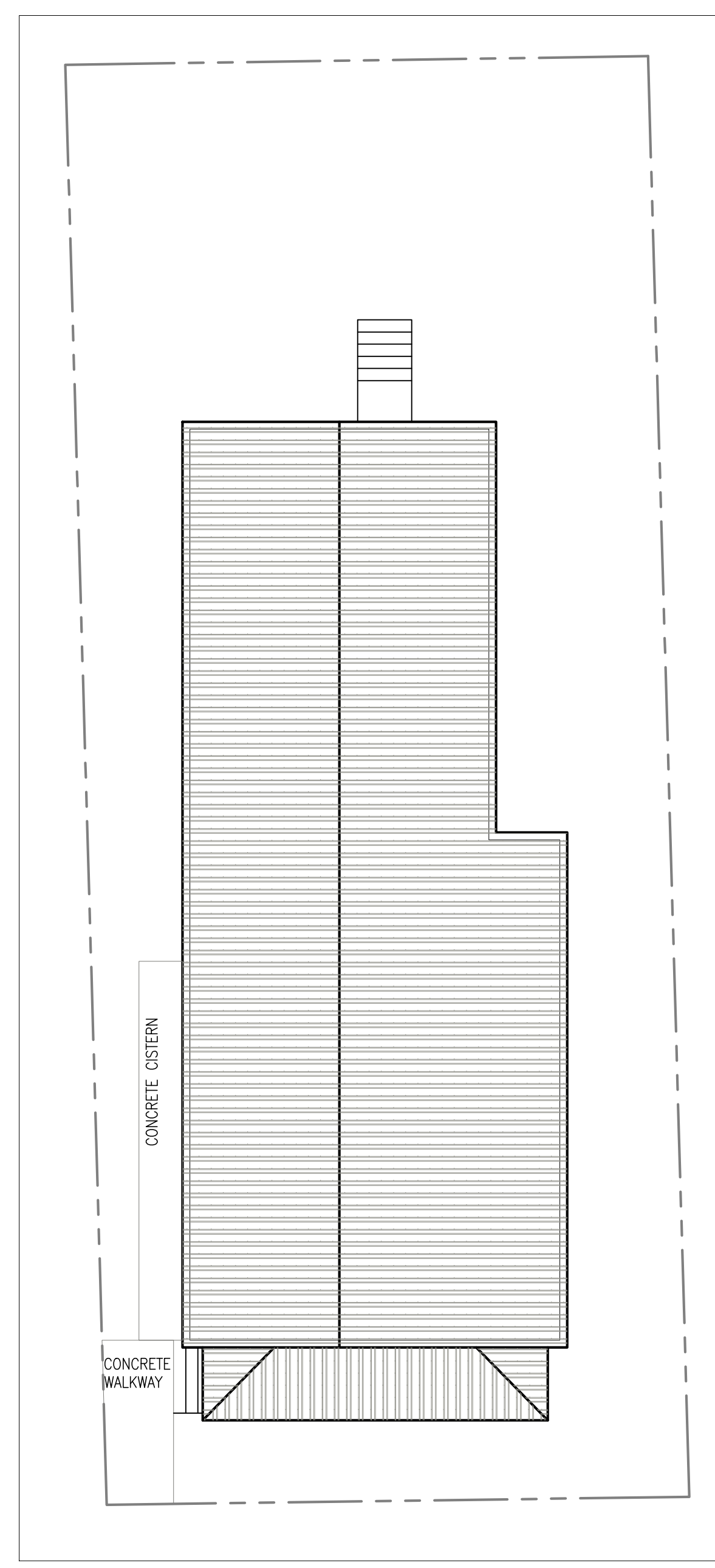
2 EXISTING SITE PLAN SCALE: 1/8"=1'-0"
