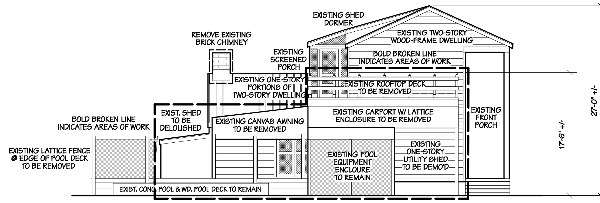
EXISTING SOUTH ELEVATION scale: 1/8"=1'-0"
