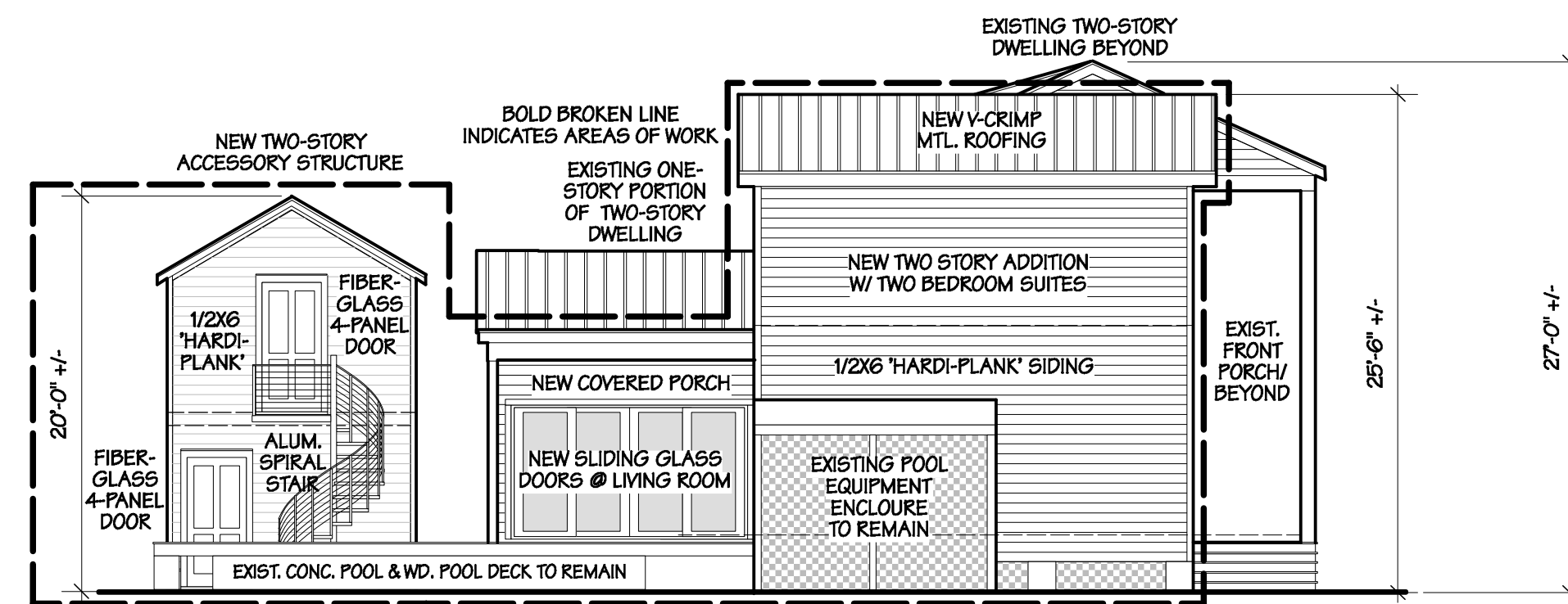
PROPOSED SOUTH ELEVATION scale: 1/8"=1'-0"
