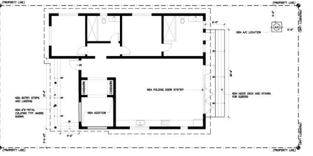
4 PROPOSED FLOOR PLAN Scale: 1/4" = 1'-0"
