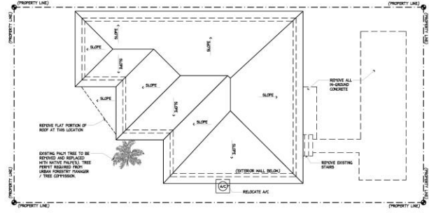
3 EXISTING SITE PLAN Scale: 1/4" = 1'-0"
