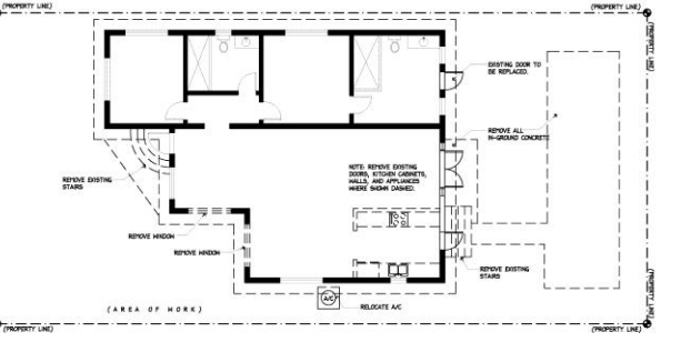
5 EXISTING FLOOR PLAN Scale: 1/4" = 1'-0"
