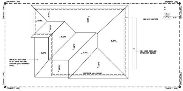
2 PROPOSED SITE PLAN Scale: 1/4" = 1'-0"
