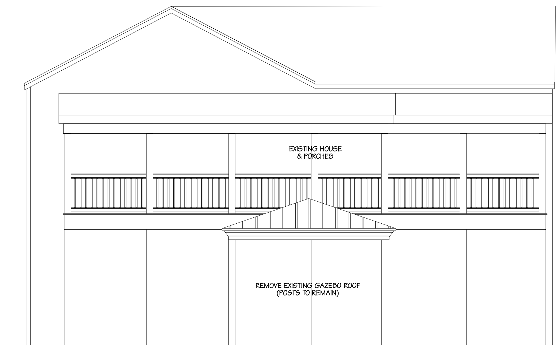
GAZEBO EXISTING SOUTH ELEVATION scale: 1/4"=1'-0"
