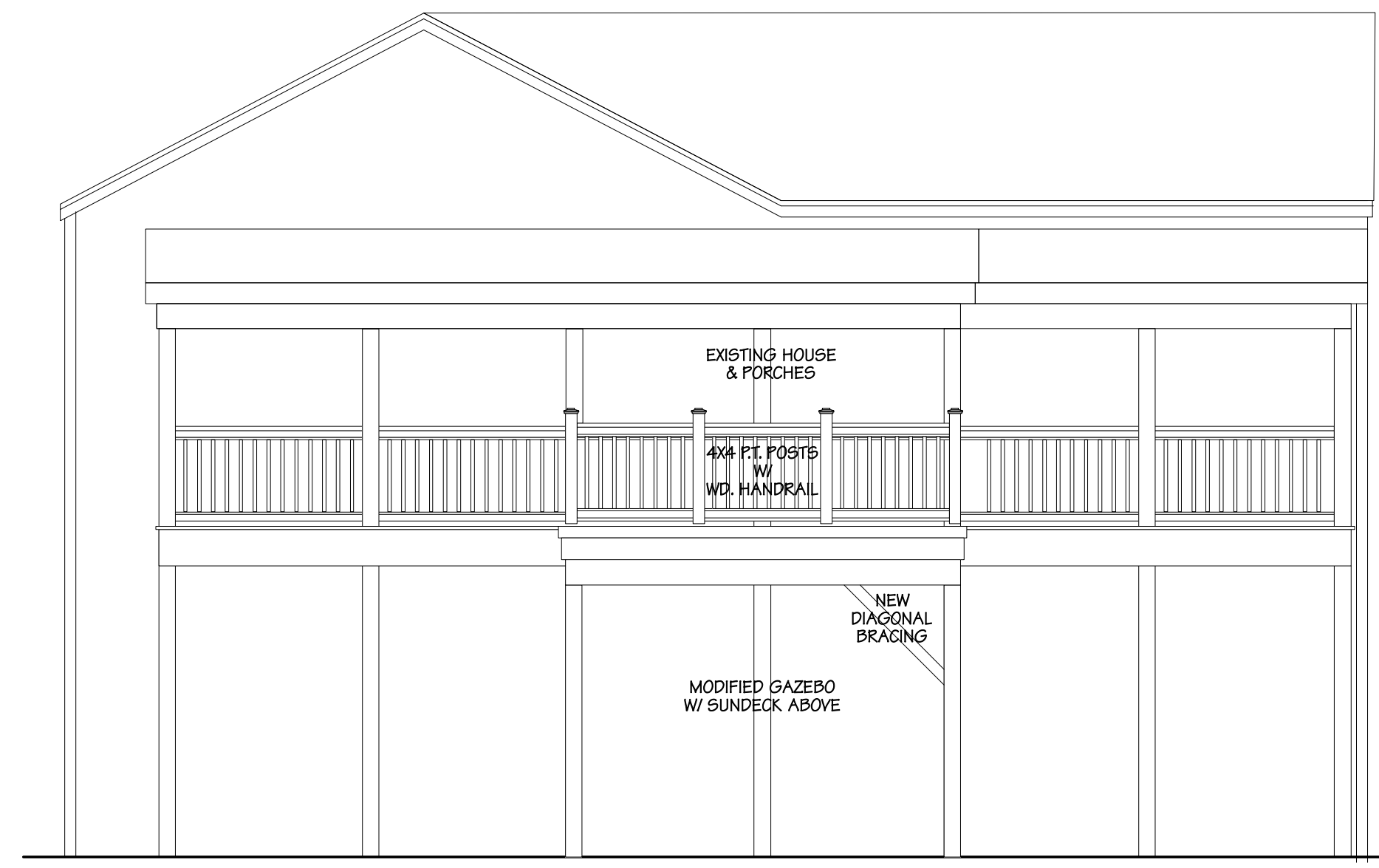
GAZEBO PROPOSED SOUTH ELEVATION scale: 1/4"=1'-0"
