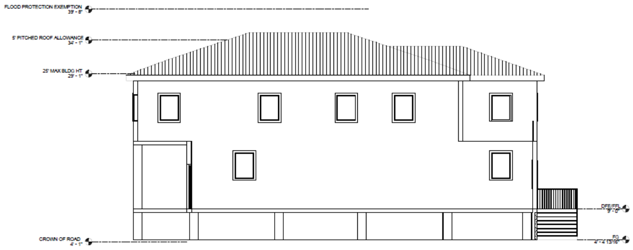
2 SOUTH ELEVATION (SIDE) SCALE: 1/4" = 1'
