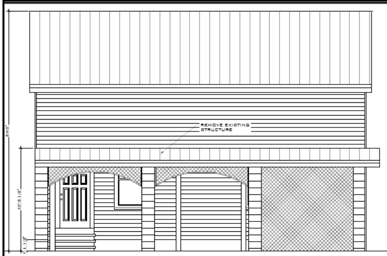
EXISTING RIGHT SIDE ELEVATION SCALE: 3/16" = 1'-0"
