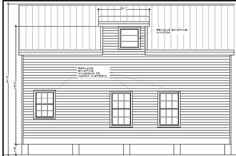
EXISTING LEFT SIDE ELEVATION SCALE: 3/16" = 1'-0"
