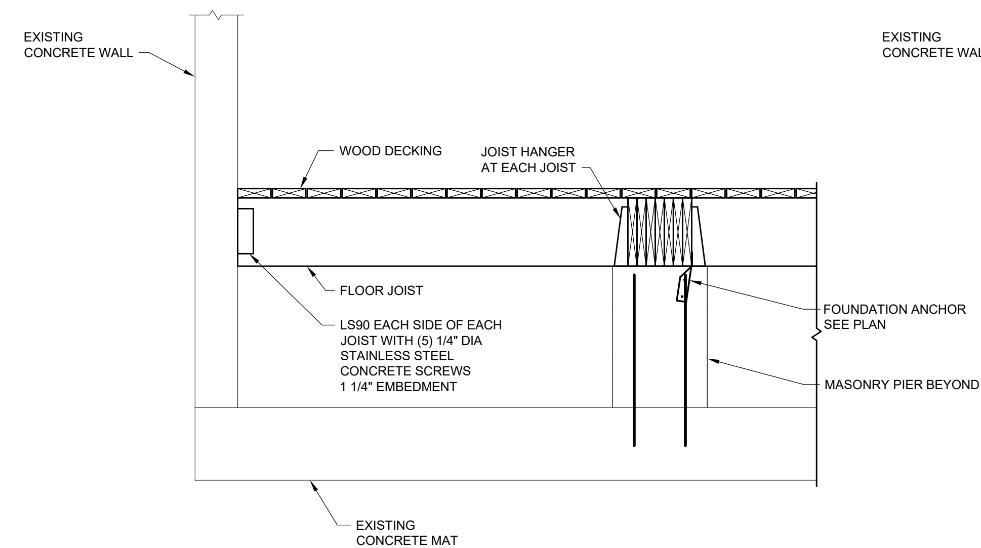
SECTION 3 SCALE: 3/4" = 1'-0" S2.1
