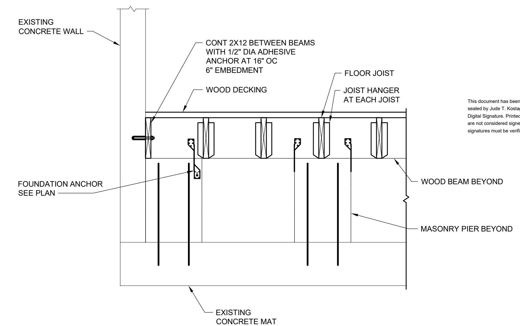
SECTION 5 SCALE: 3/4" = 1'-0" S2.1
