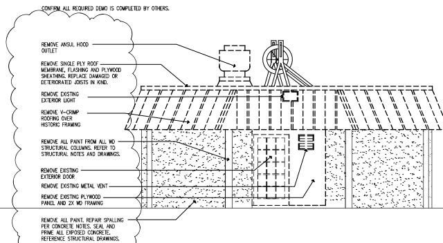
2 SOUTH ELEVATION: DEMO SCALE: 1/4" = 1'
