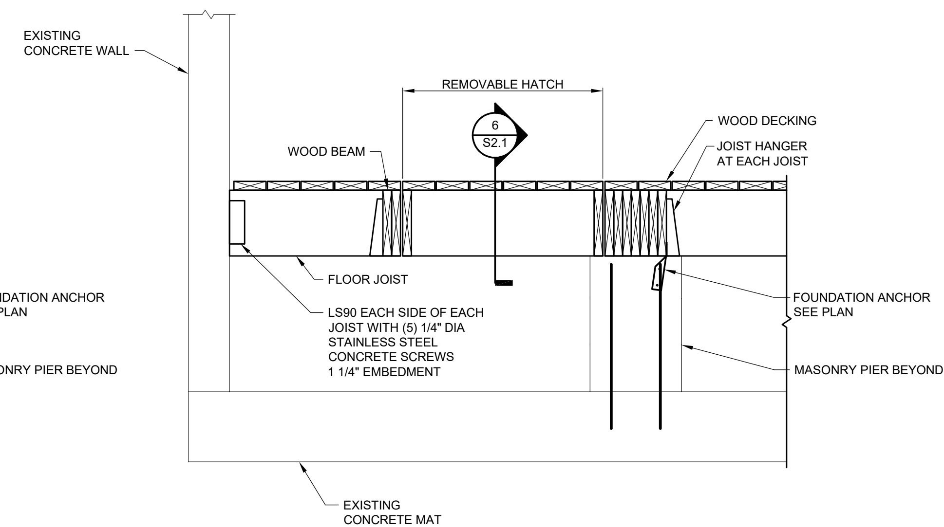
SECTION 4 SCALE: 3/4" = 1'-0" S2.1
