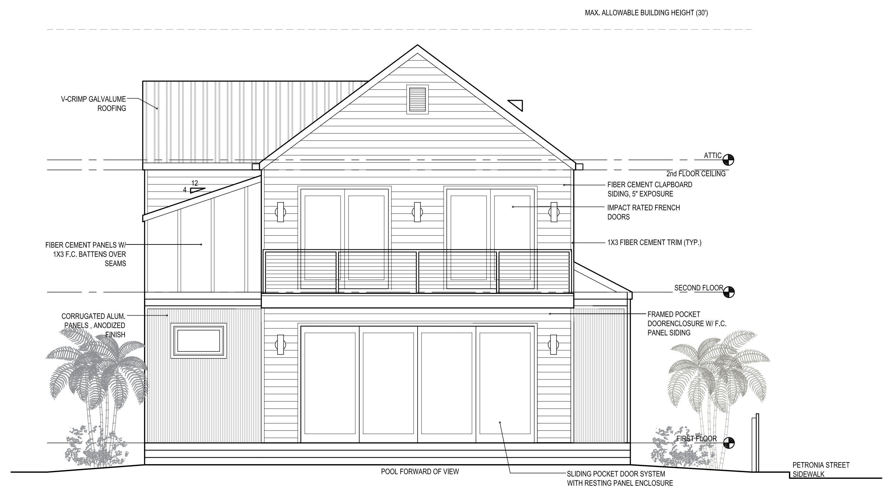
1 A3.2 EAST ELEVATION SCALE: 1/4"=1'-0"
