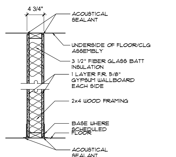
PARTITION TYPE - NON RATED 1 FIRE: N/A U.L. N/A SOUND: N/A TYPICAL APPLICATION: TYPICAL WALL
