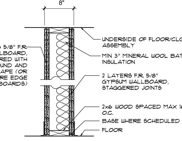
PARTITION TYPE - ONE HOUR 3 FIRE: 2 HR3 U.L. U200 SOUND: STC54 TYPICAL APPLICATION: FIRE RATED PLUMBING WALL
