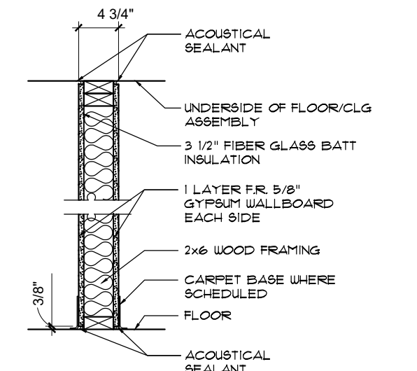
PARTITION TYPE - ONE HOUR 4 FIRE: 1 HR U.L. U200 SOUND: STC50 TYPICAL APPLICATION: PARTITION WALL
