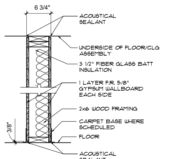
PARTITION TYPE - NON RATED 2 FIRE: 1 HR U.L. U200 SOUND: STC50 TYPICAL APPLICATION: PLUMBING WALL
