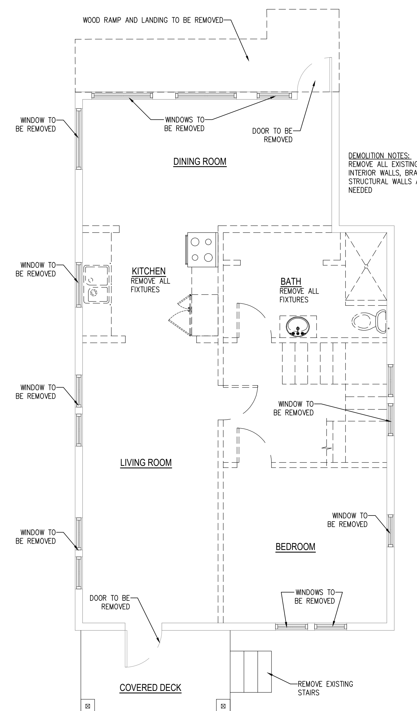
(PRE CONSTRUCTION) EXISTING 1ST FLOOR PLAN
