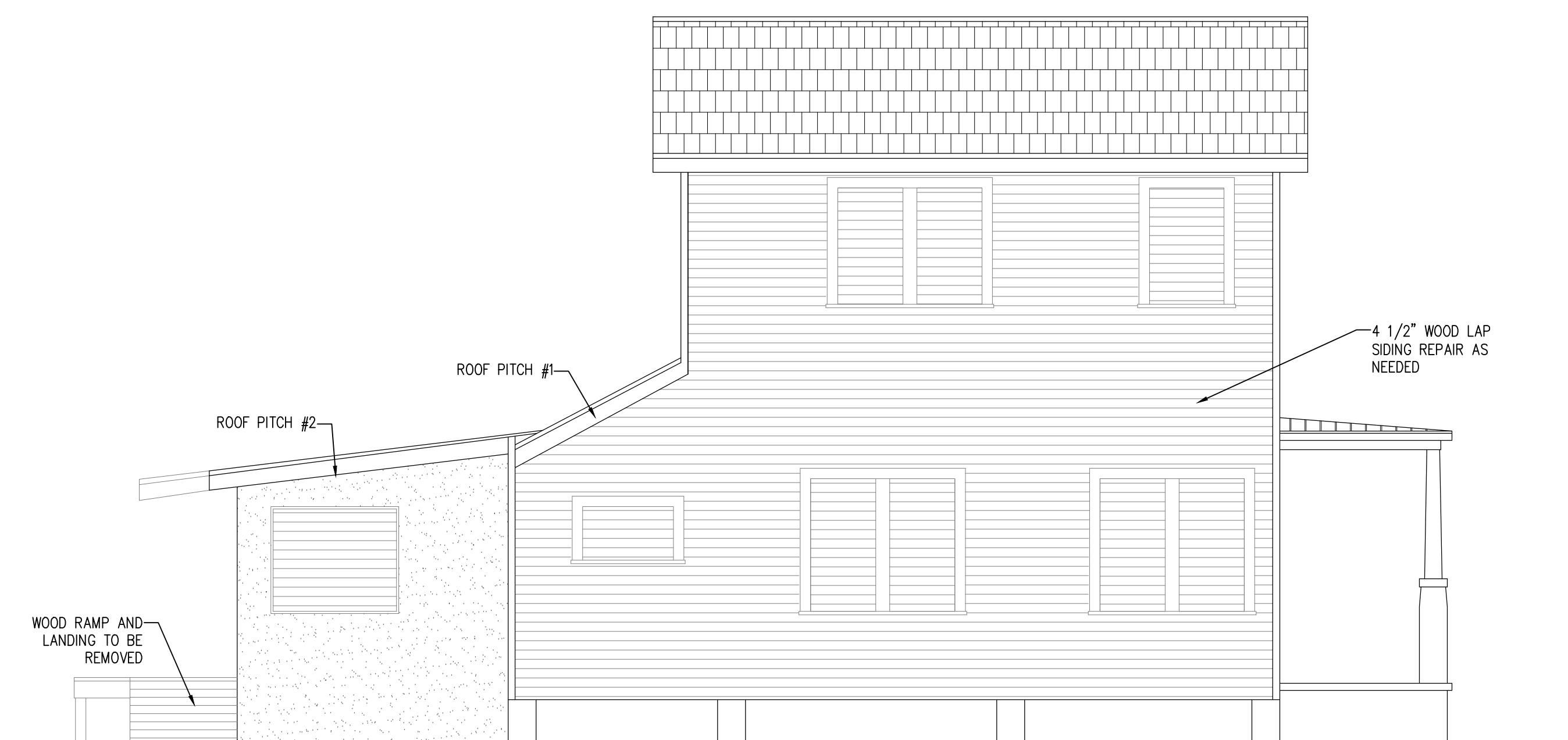
(PRE CONSTRUCTION) EXISTING SIDE ELEVATION
