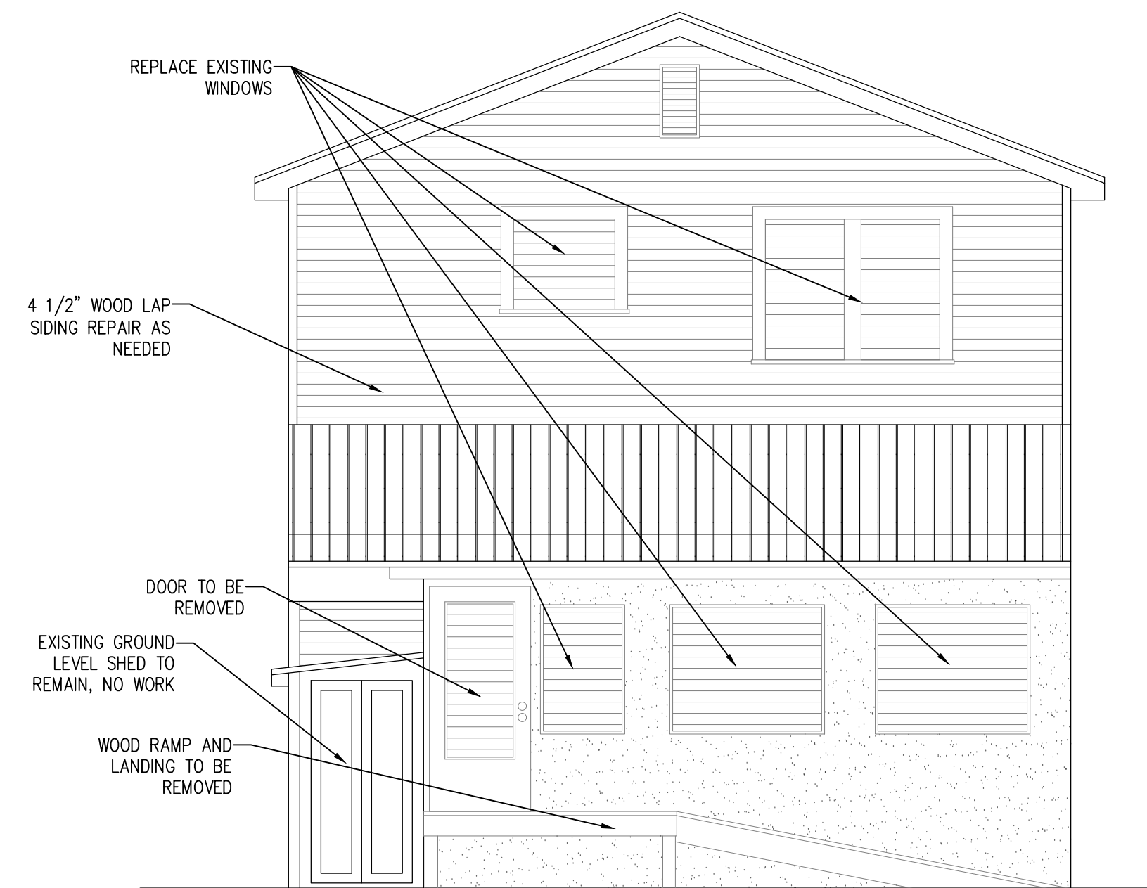
(PRE CONSTRUCTION) EXISTING REAR ELEVATION
