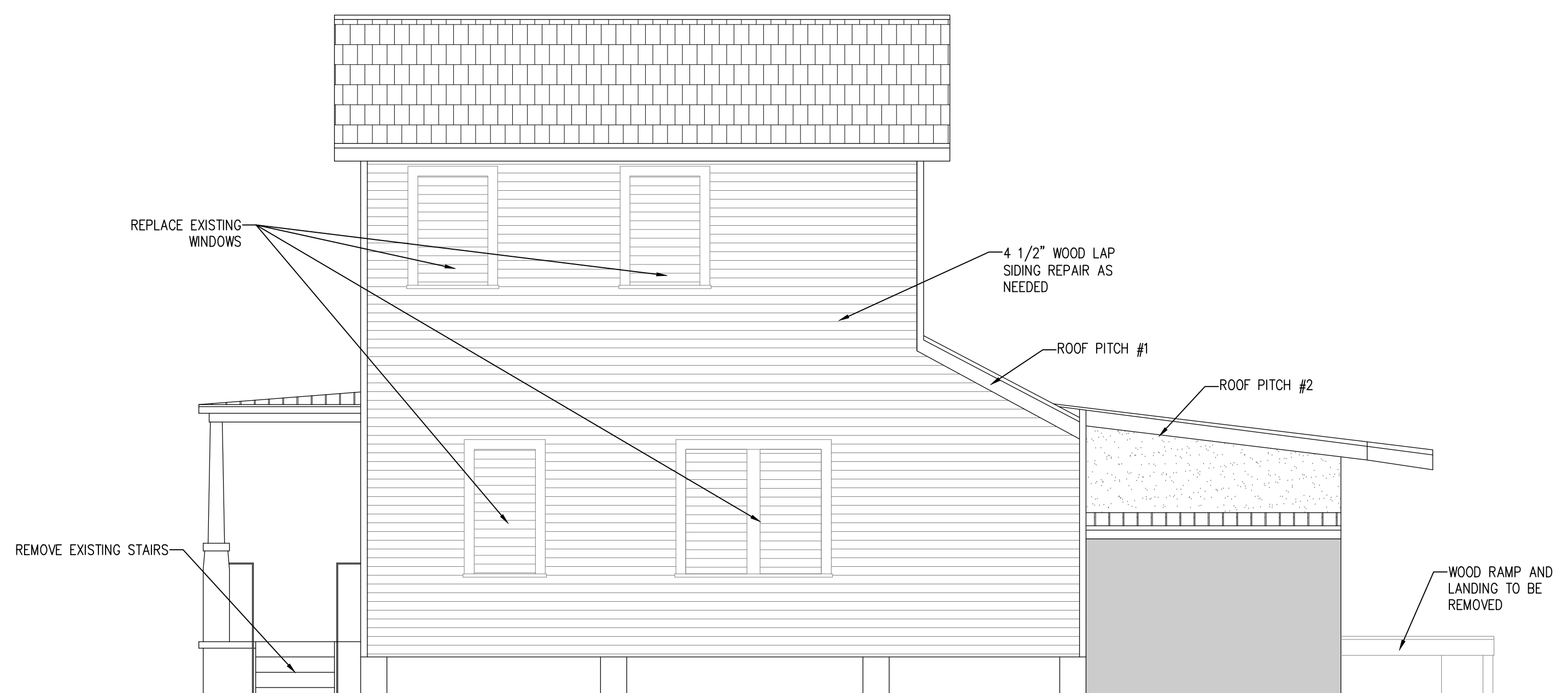
(PRE CONSTRUCTION) EXISTING SIDE ELEVATION
