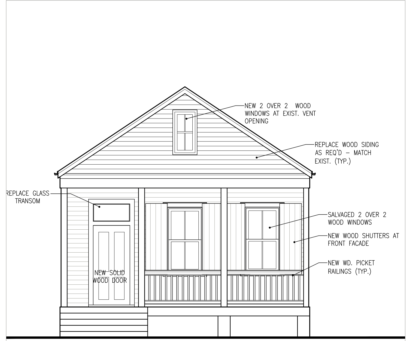
1 WEST ELEVATION SCALE: 1/4"=1'-0"
