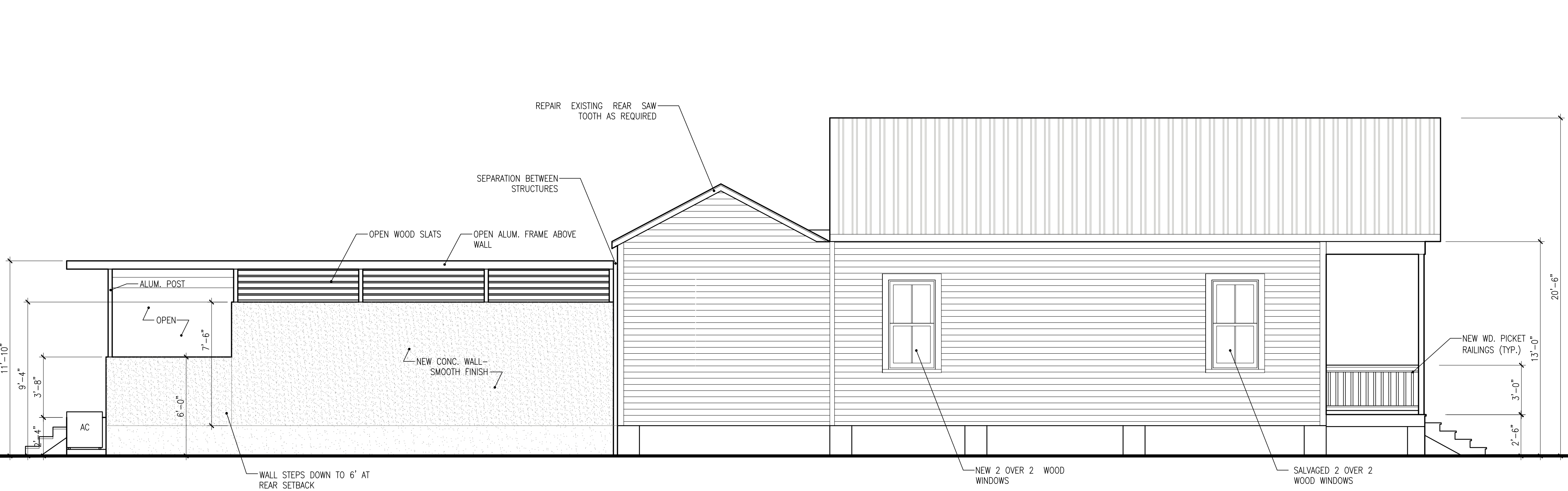
4 NORTH ELEVATION SCALE: 1/4"=1'-0"
