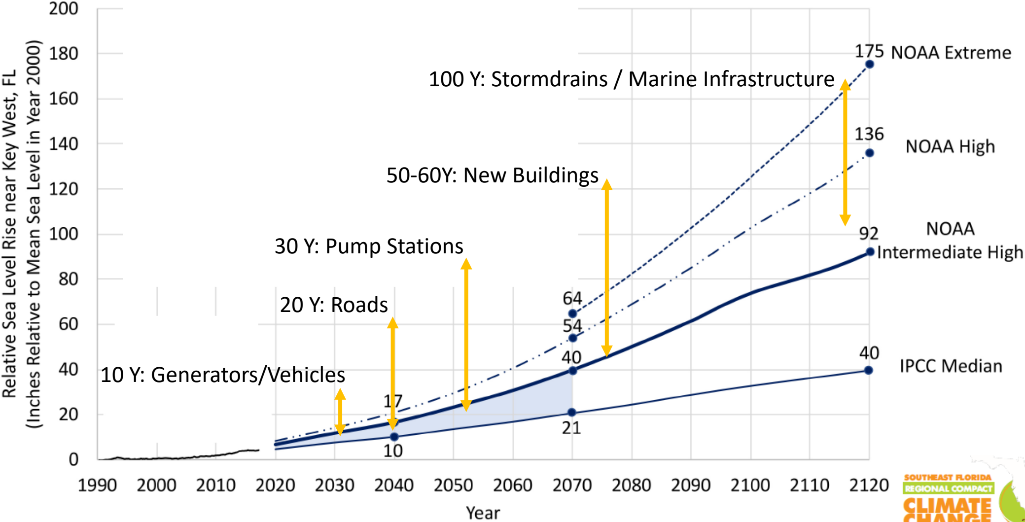
FIGURE 1: Unified Sea Level Rise Projection
