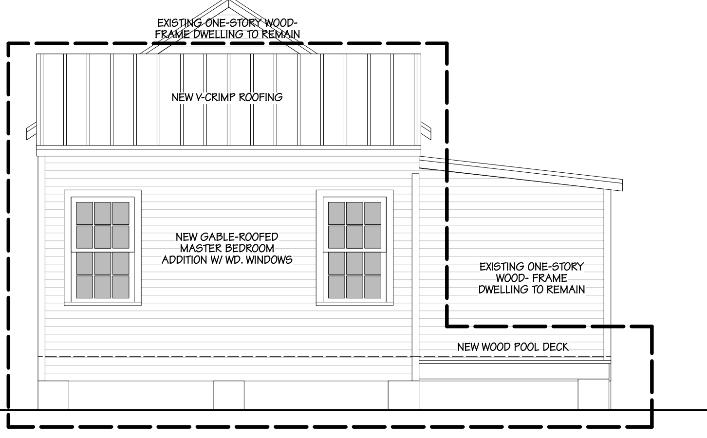
PROPOSED WEST ELEVATION scale: 1/4"=1'-0"
