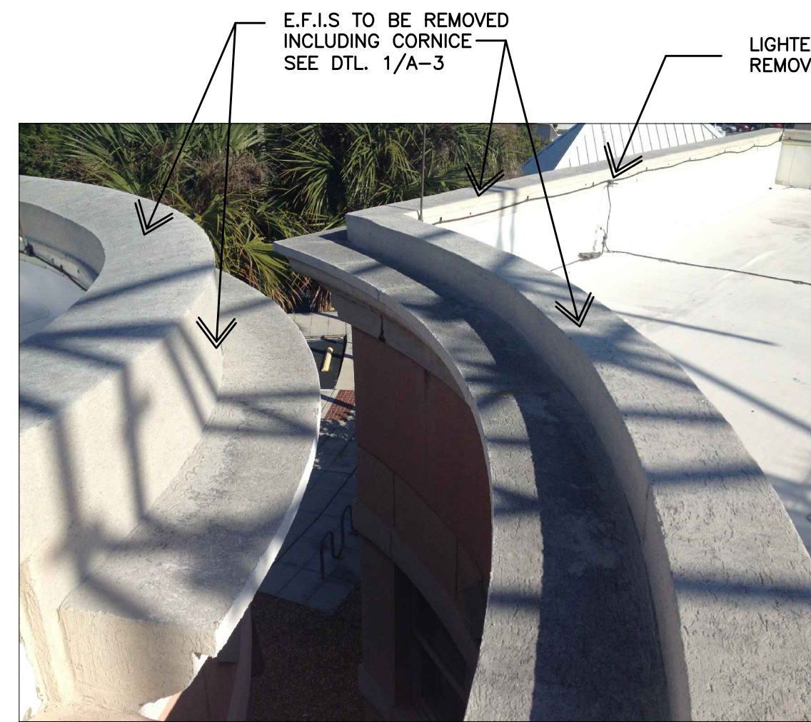
1 ENTRY 'TOWER' CORNICE DETAILS A-2
