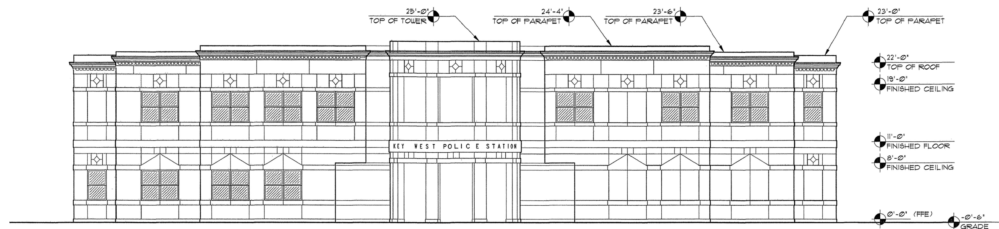
10 EXISTING FRONT ELEVATION - NORTH A-2.1
