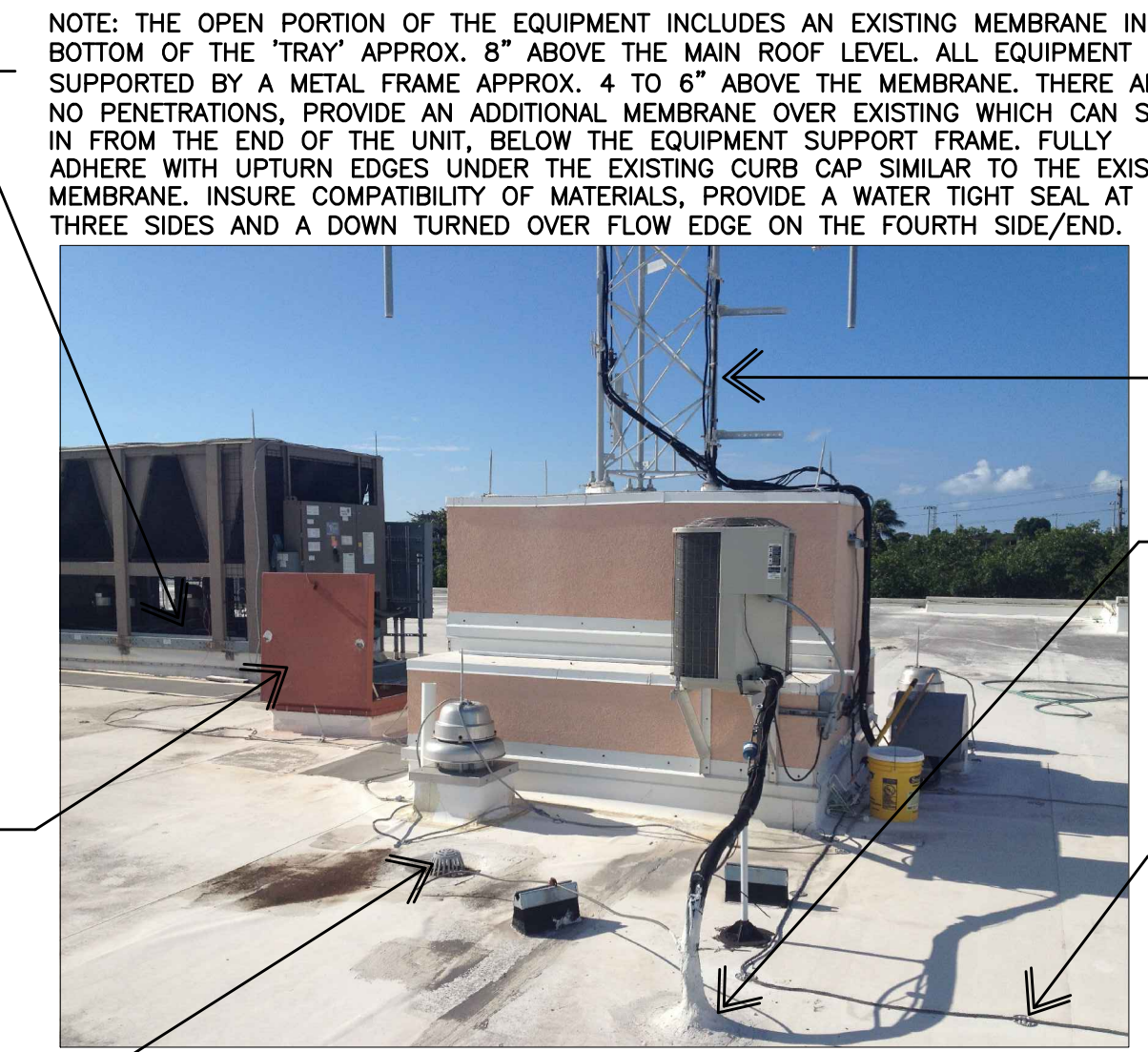
4 STEPPED PENTHOUSE & ANTENNA A-2
