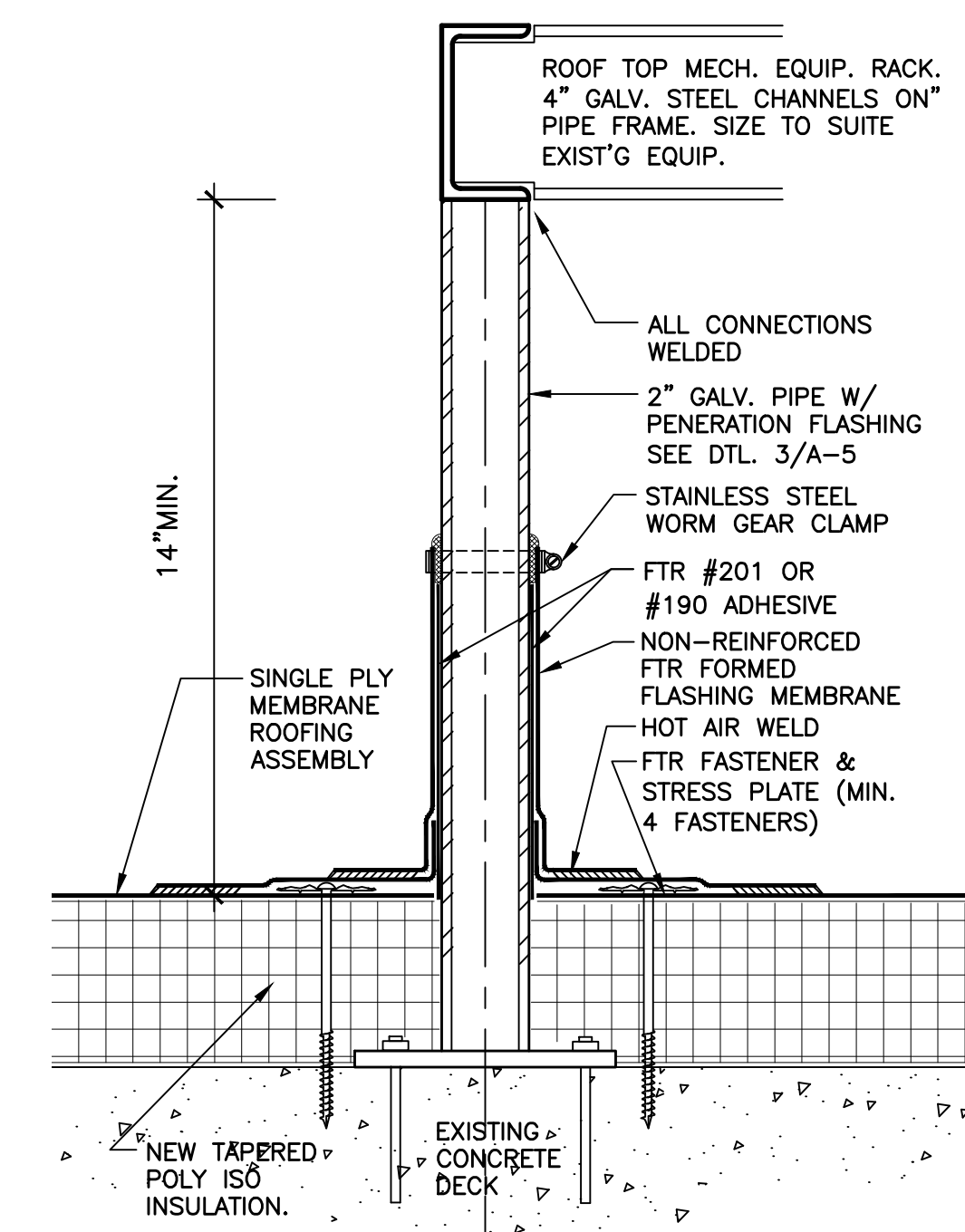
4 EQUIP. RACK-EXISTING SCALE : 3" = 1'-0"
