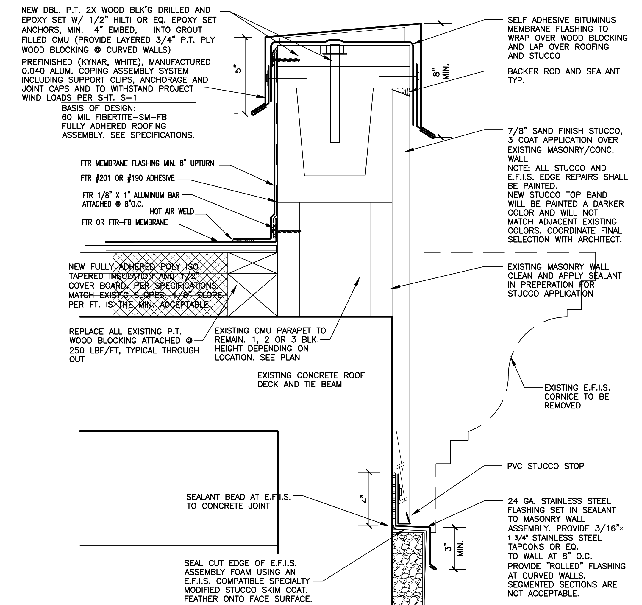
1 NEW PARAPET DTL. - BASE BID
