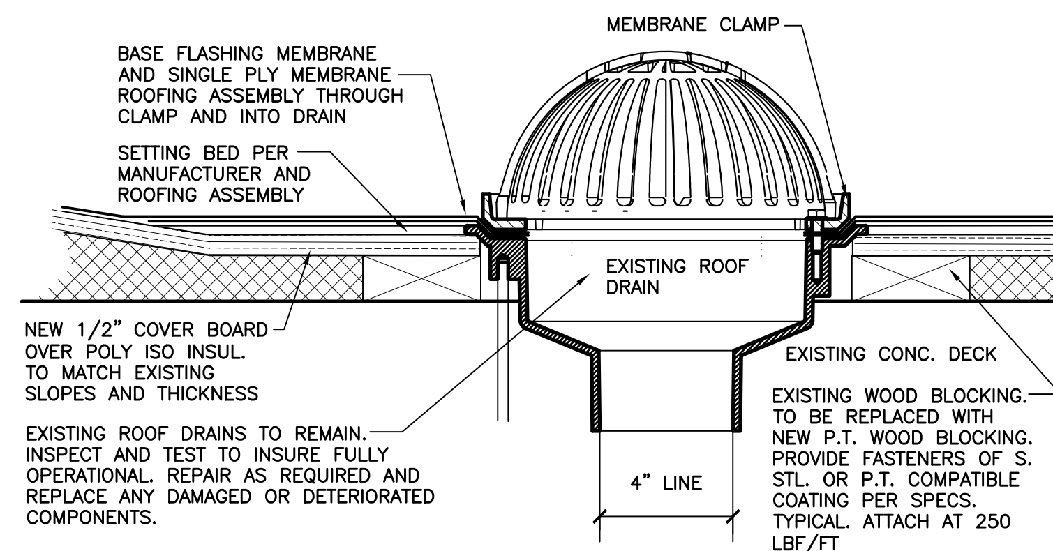
5 ROOF DRAIN DTL. SCALE : 3" = 1'-0"
