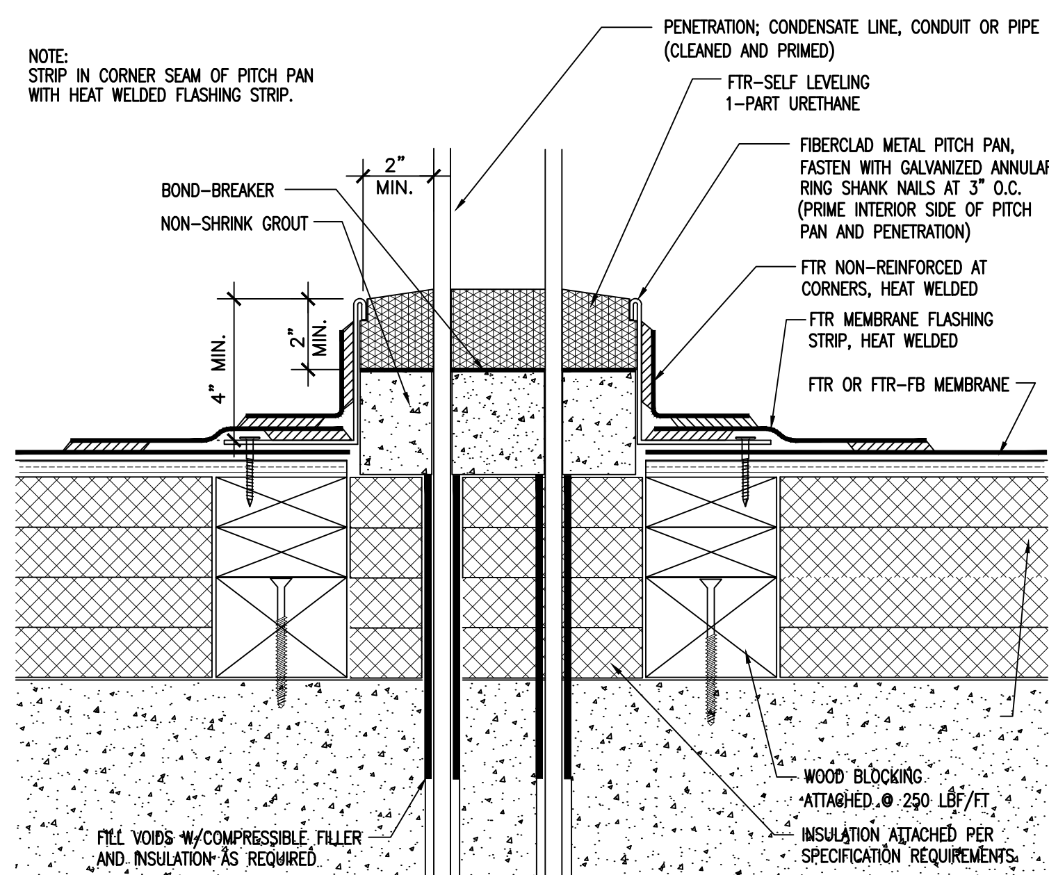
1 MULTIPLE PENETRATION PITCH POCKET SCALE : 3" = 1'-0"
