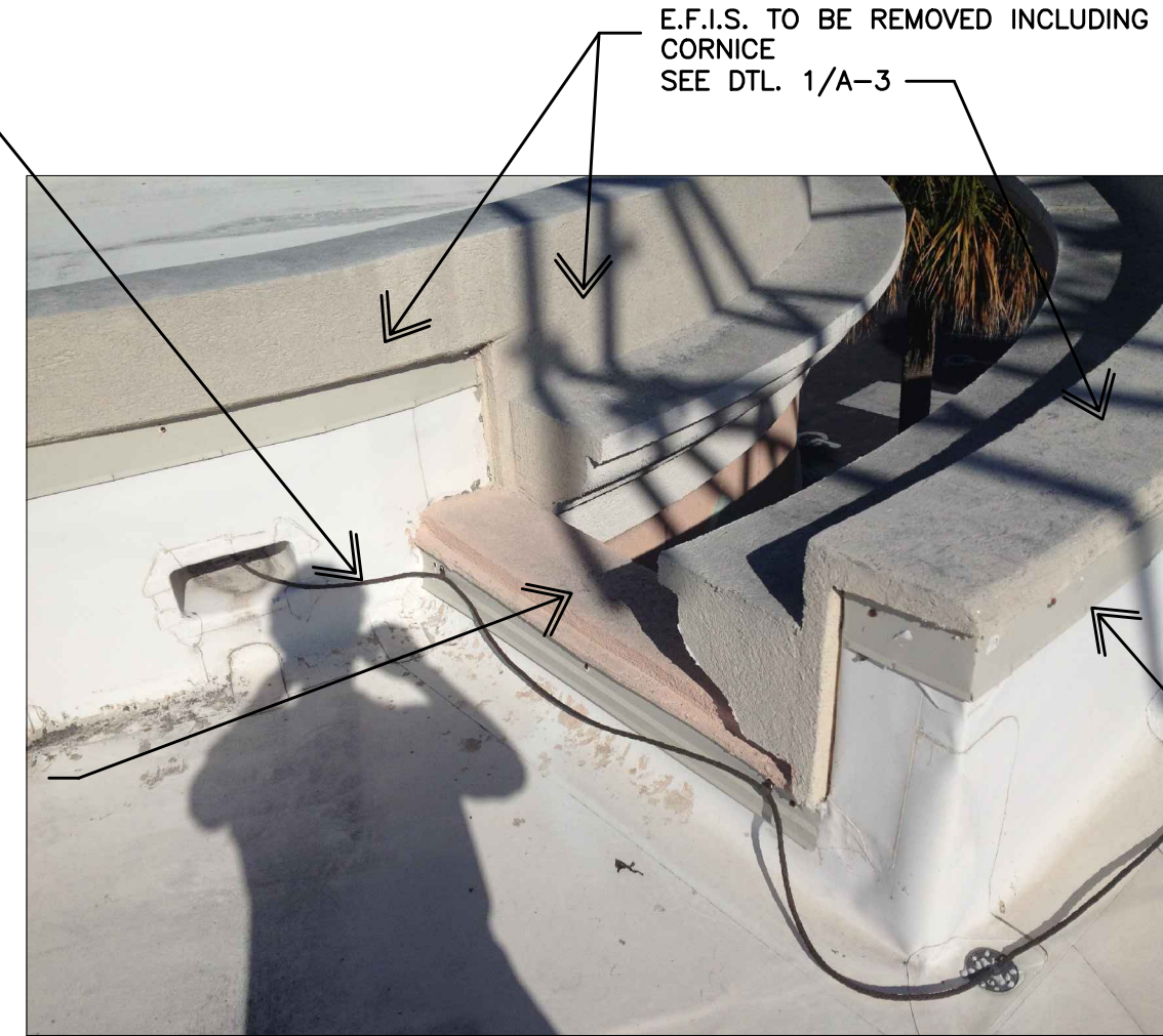
2 ENTRY 'TOWER' CORNICE DETAILS A-2
