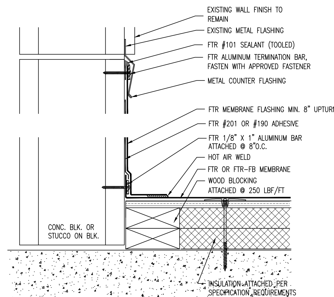
6 WALL FLASHING DTL. SCALE : 3" = 1'-0"
