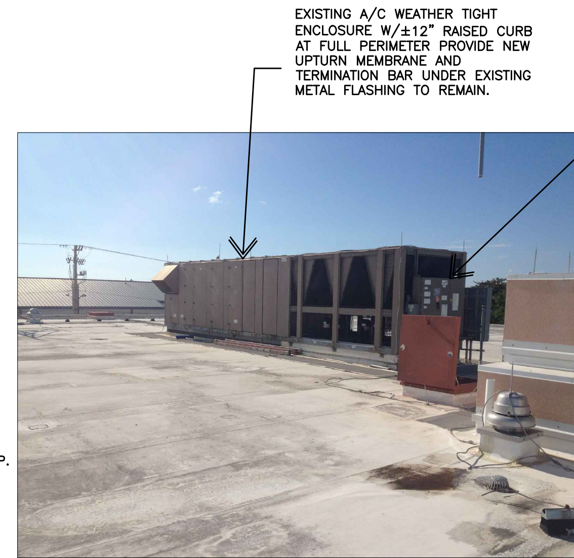
3 A/C EQUIPMENT A-2
