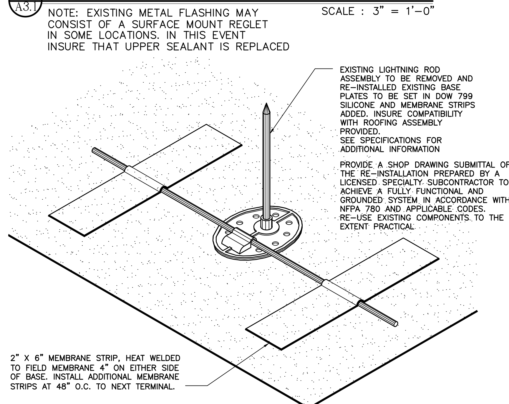
2 LIGHTNING PROTECTION SCALE : 3" = 1'-0"
