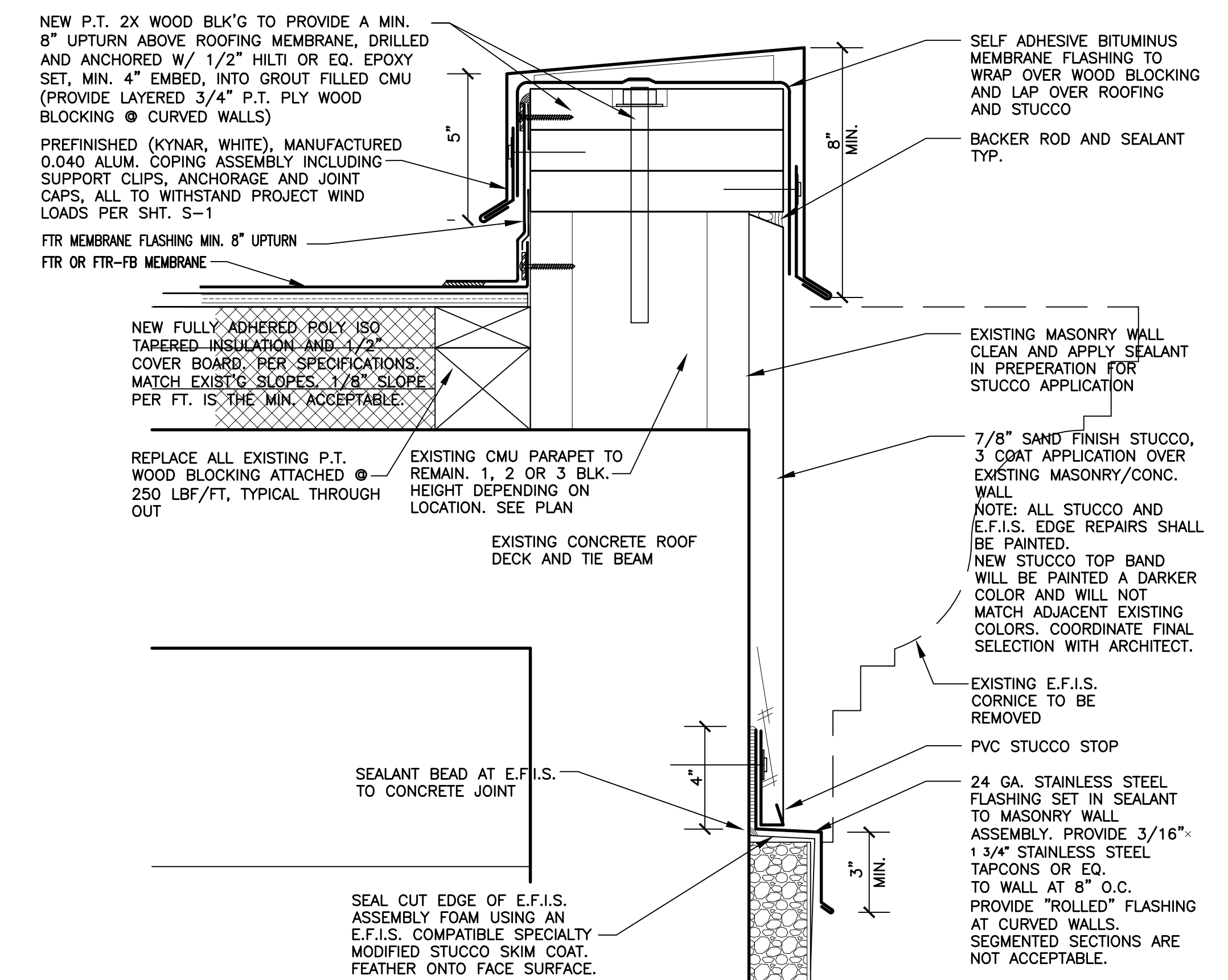
2 NEW CURB DTL. - BASE BID
