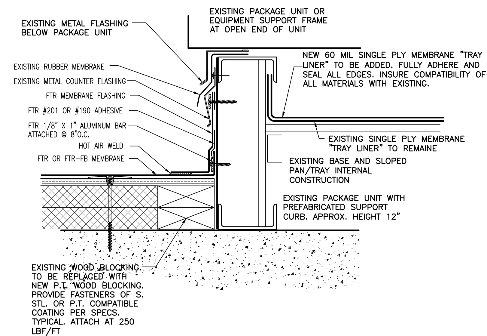
6 PACKAGE AC EQUIP. CURB FLASHING DTL. SCALE : 3" = 1'-0"
