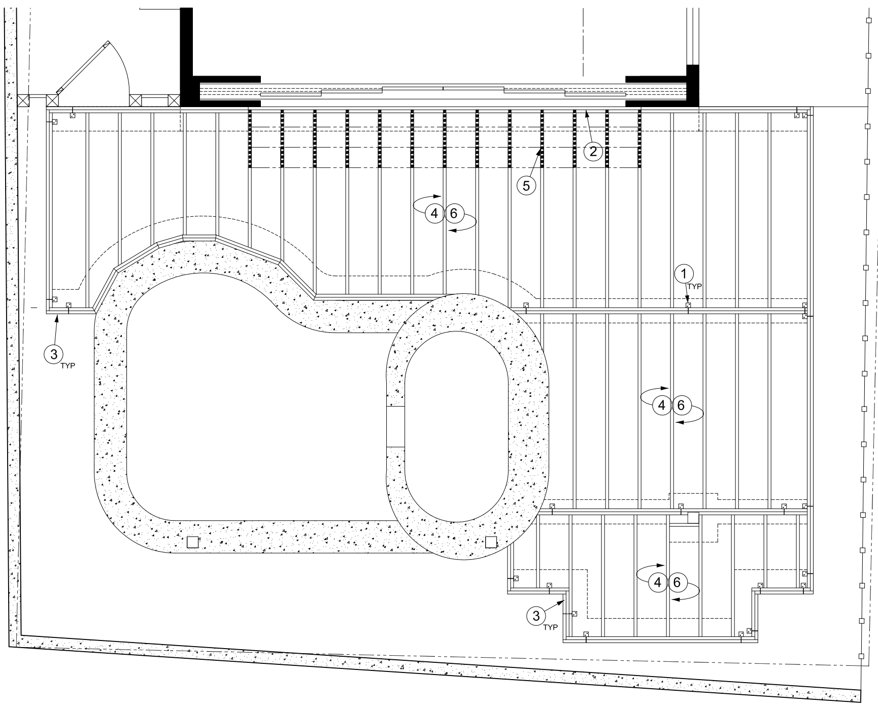
1 Proposed Deck Framing Plan A-3.3
