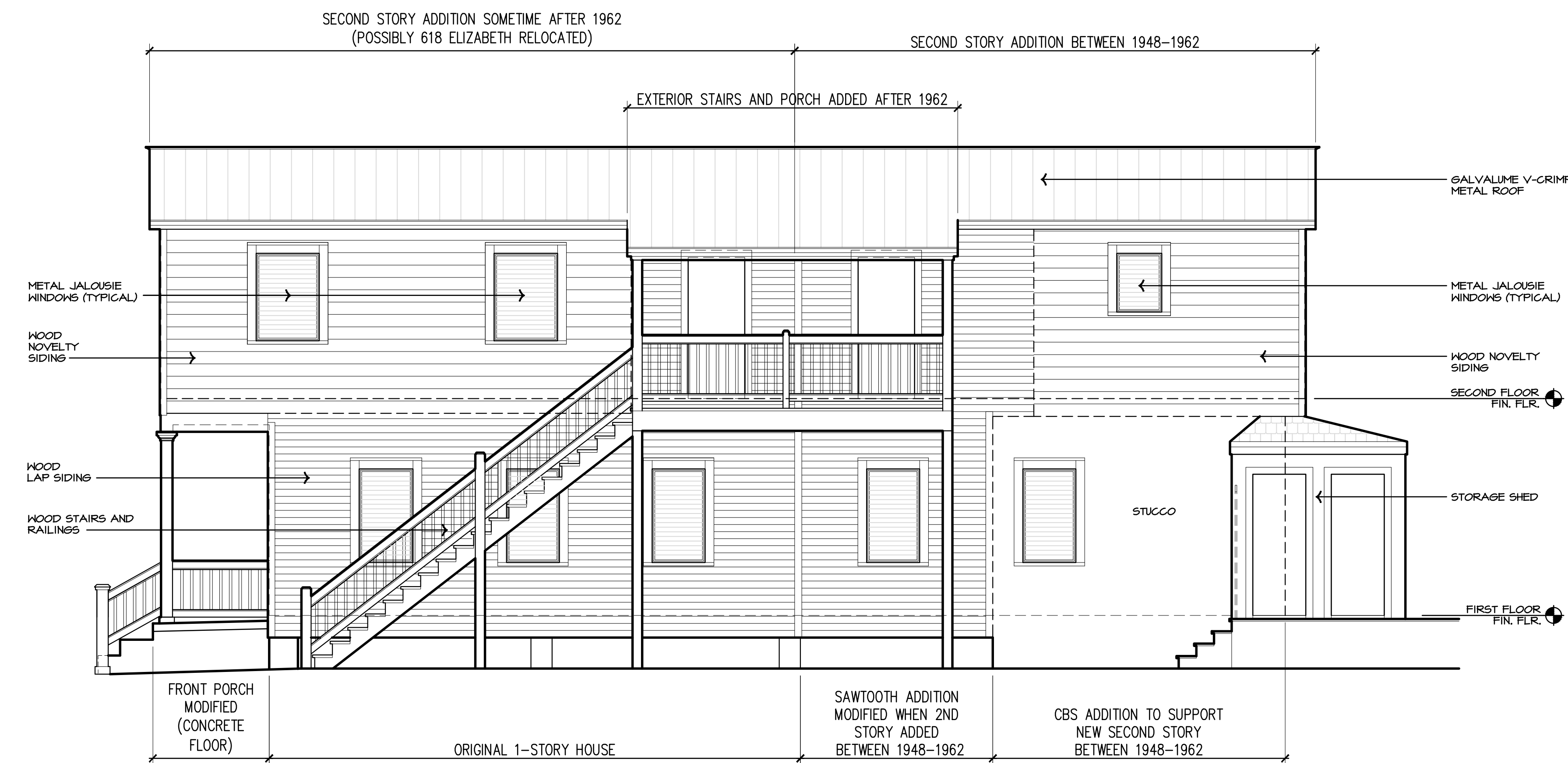
EXISTING NORTH SIDE ELEVATION
