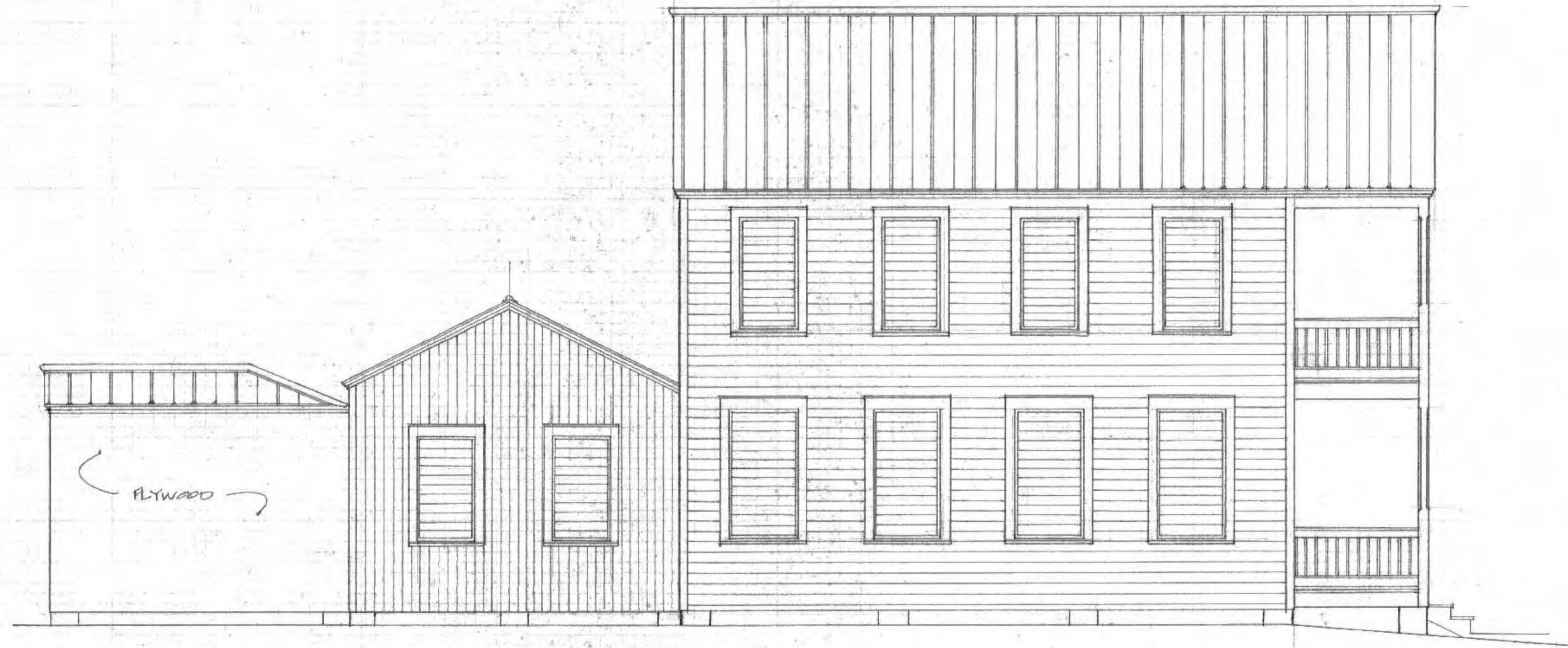
NORTHEAST ELEVATION 1/4"=1'-0"
