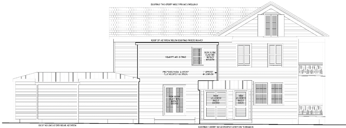
PROPOSED LEFT SIDE (EAST) ELEVATION scale: 1/4"=1'-0"
