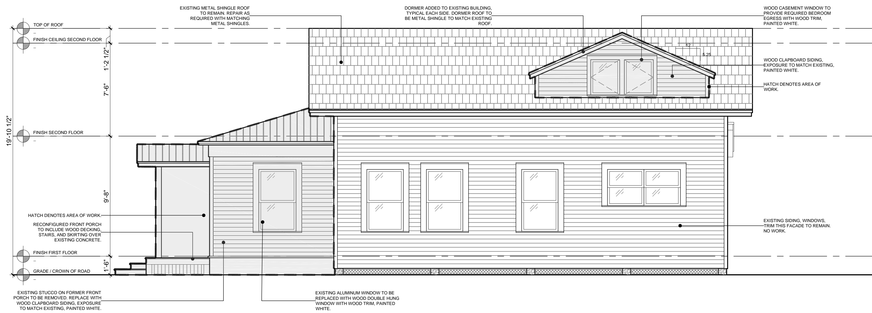
02 North Elevation 1/4" = 1'-0"
