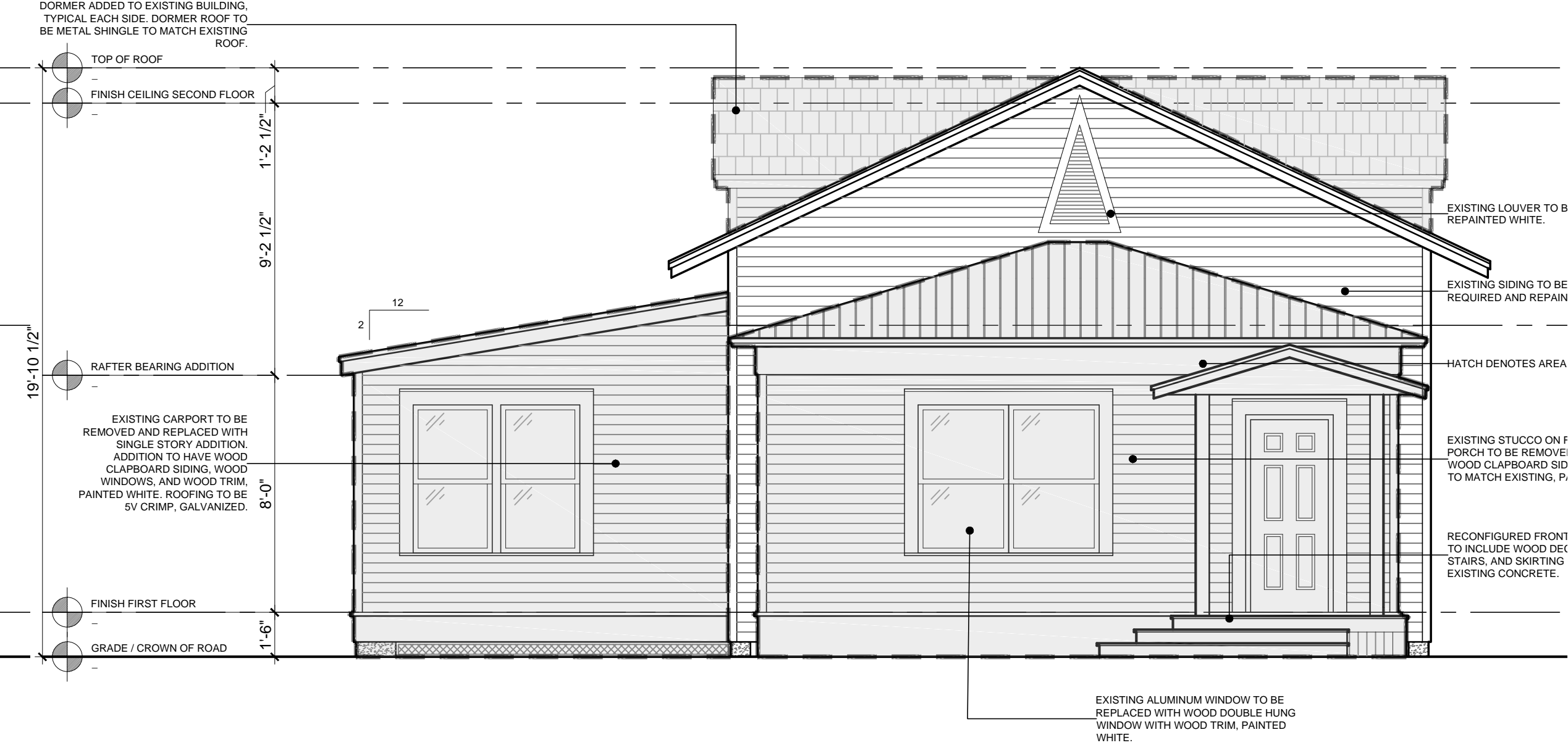
01 East Elevation - Margaret Street 1/4" = 1'-0"
