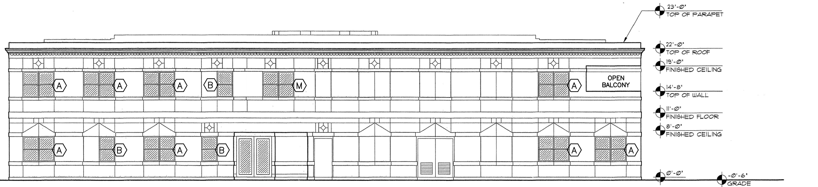
3 REAR ELEVATION (SOUTH EAST) A-3 SCALE : 1/8" = 1'-0"
