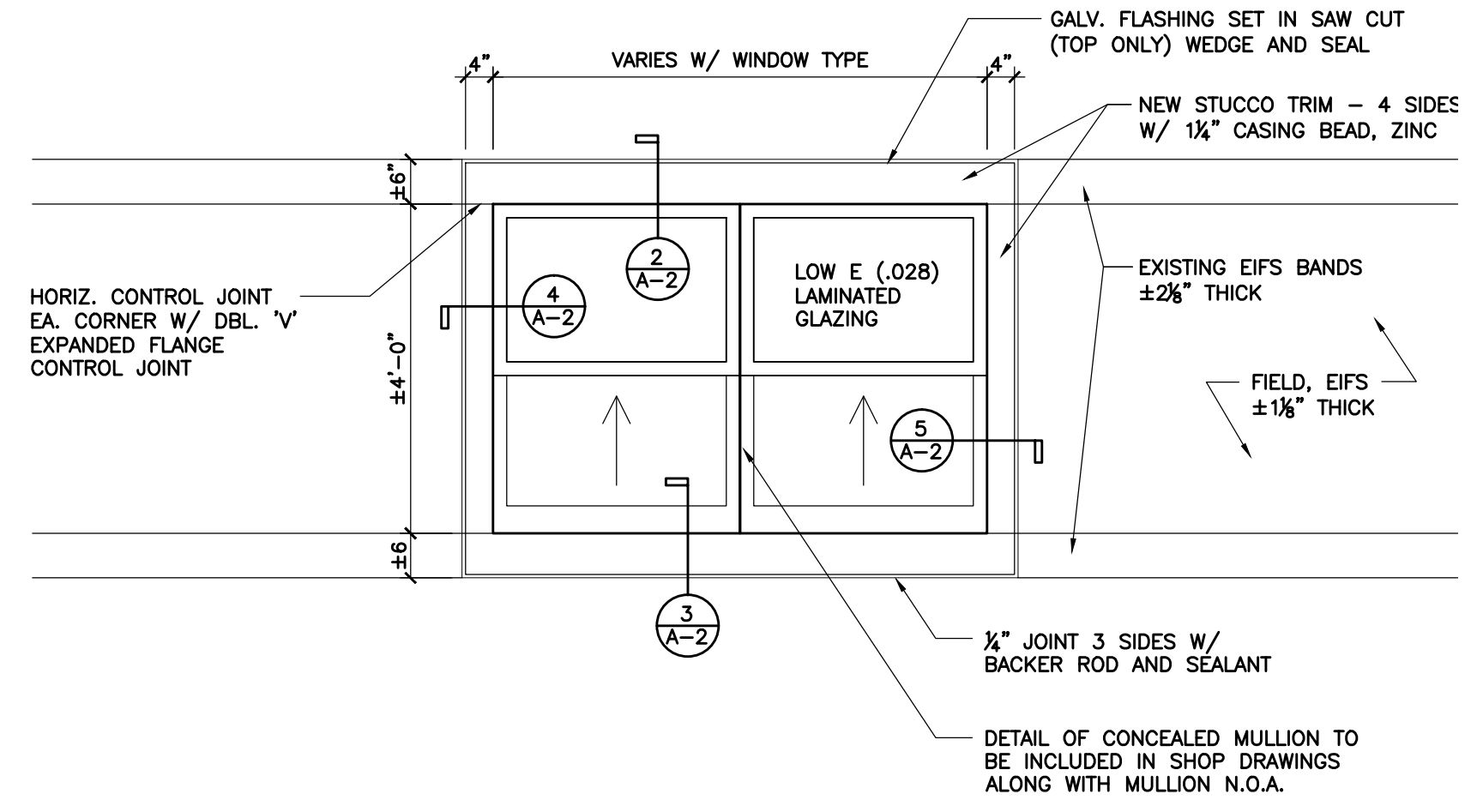
5 WINDOW ELEVATION A-3 SCALE : 1/2" = 1'-0"
