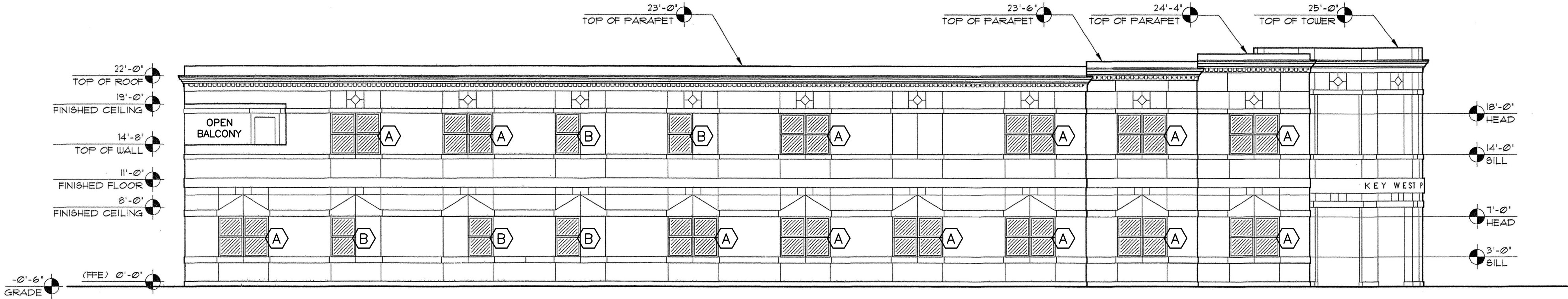
2 SIDE ELEVATION (NORTH EAST) A-3 SCALE : 1/8" = 1'-0"
