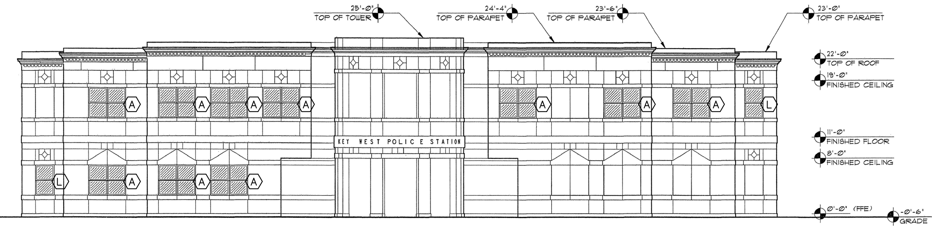
1 FRONT ELEVATION (NORTH WEST) A-3 SCALE : 1/8" = 1'-0"
