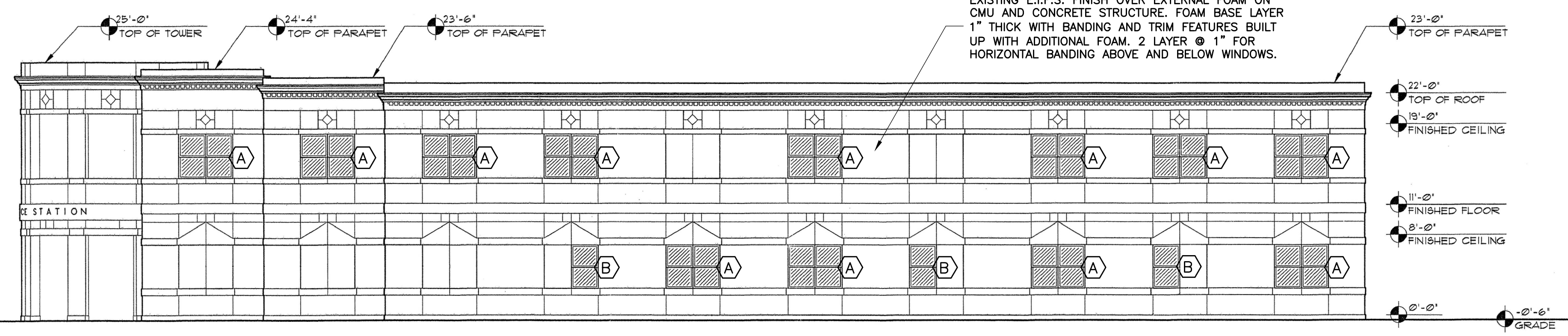
4 SIDE ELEVATION (NORTH EAST) A-3 SCALE : 1/8" = 1'-0"
