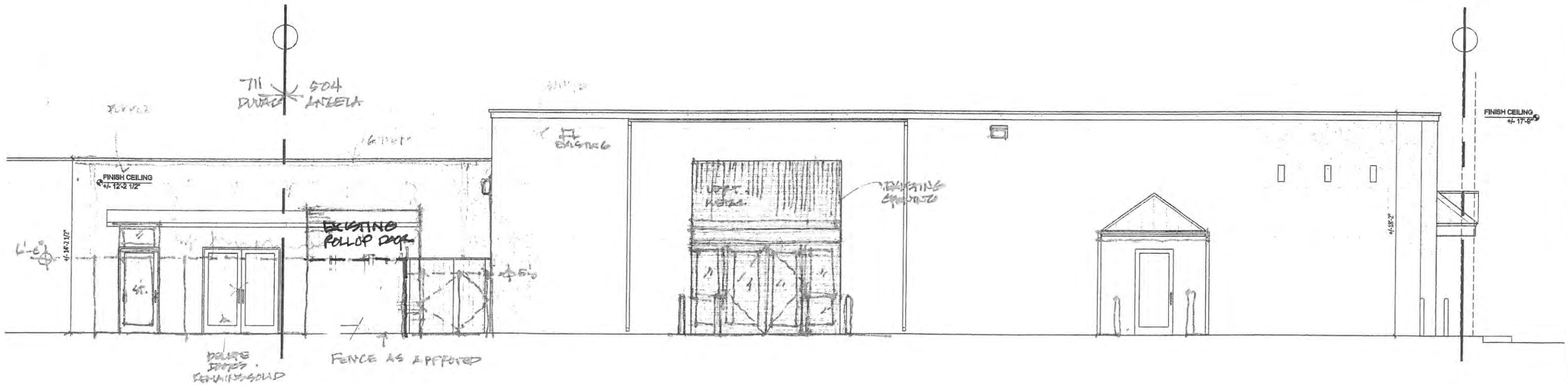
2 PROPOSED ELEVATION AT PARKING SCALE: 1/4" = 1'-0" GRAPHIC SCALE: 1/4" = 1'-0"
