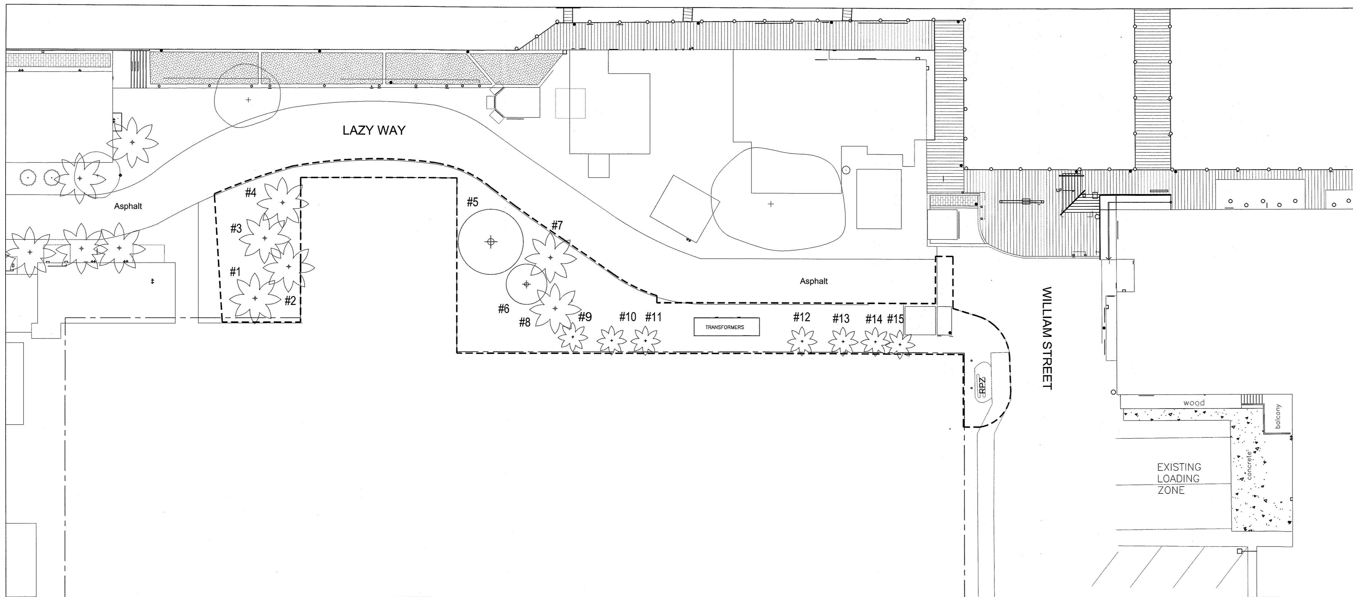
1 TREE DISPOSITION PLAN SCALE: 1" = 20'-0"
