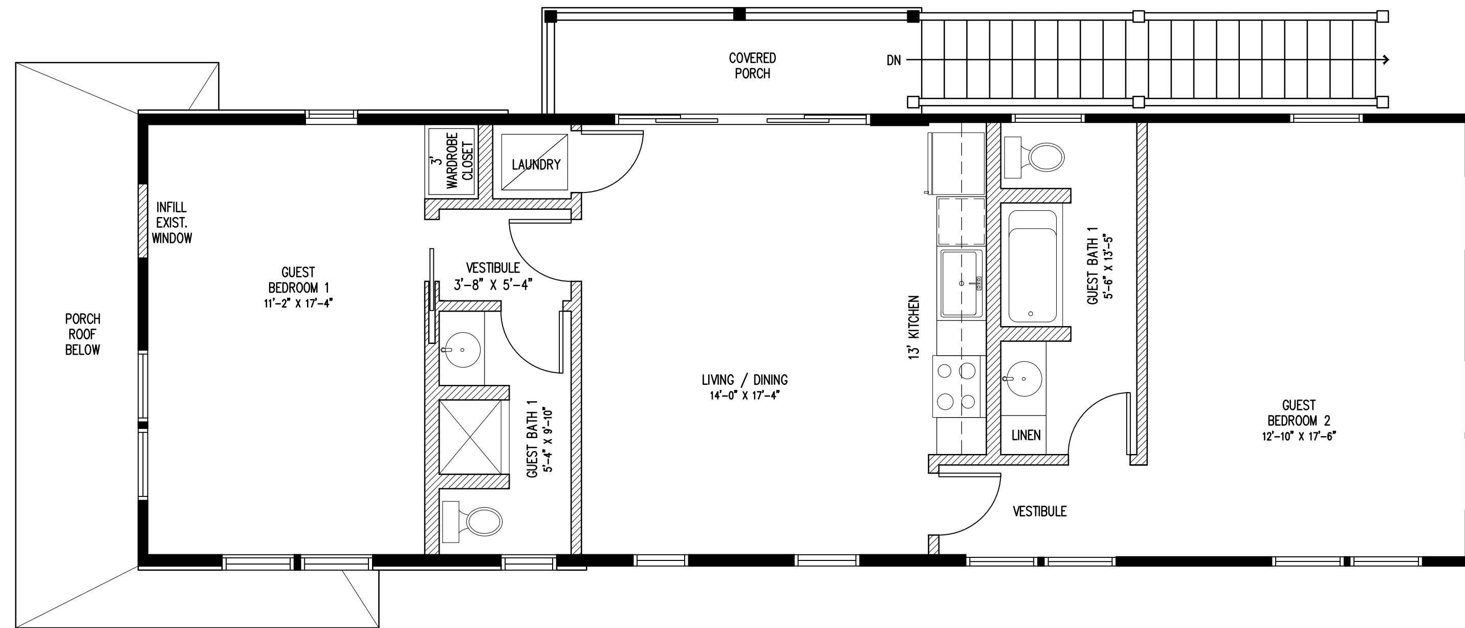
PROPOSED SECOND FLOOR PLAN 1/4" = 1'-0"
