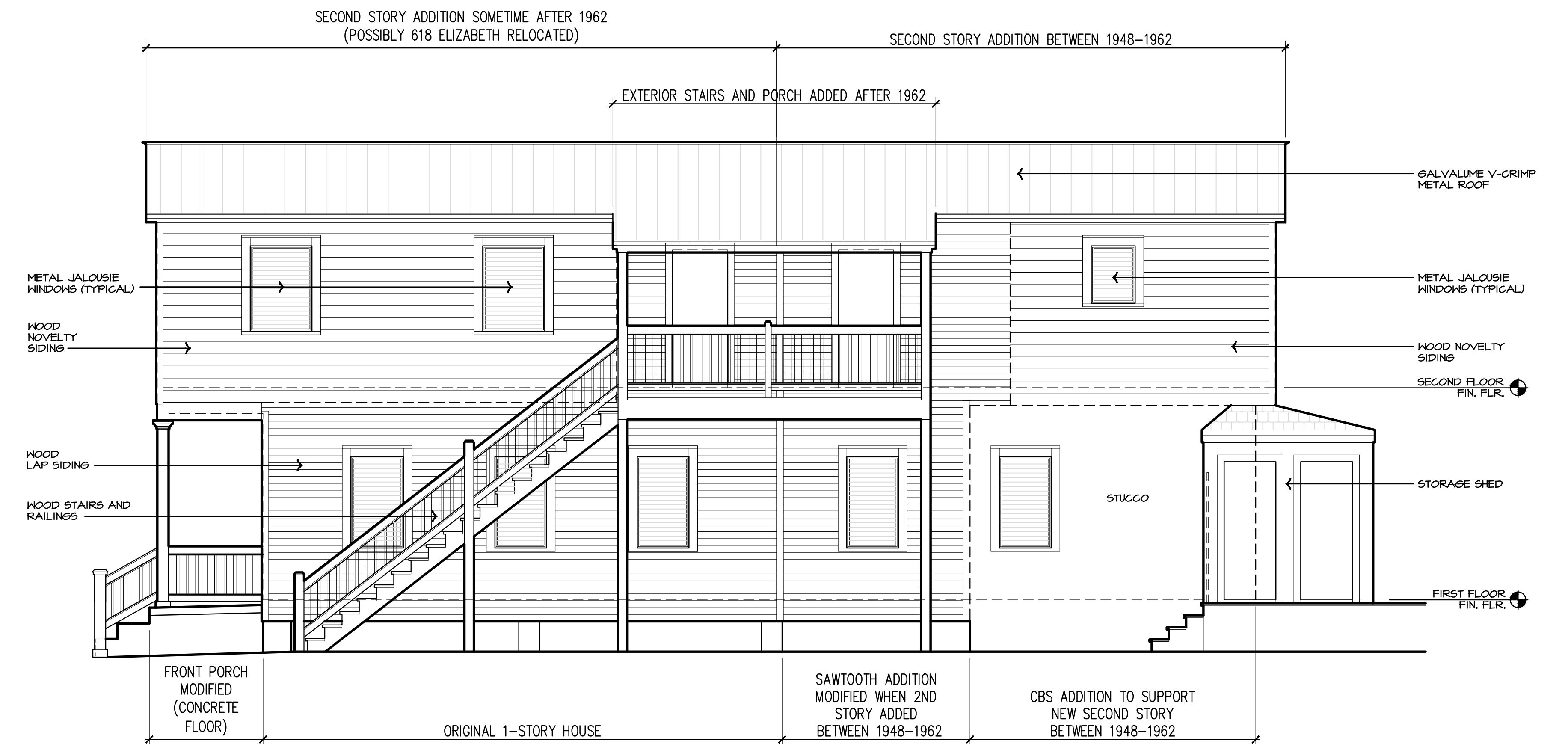
EXISTING NORTH SIDE ELEVATION 1/4" = 1'-0"
