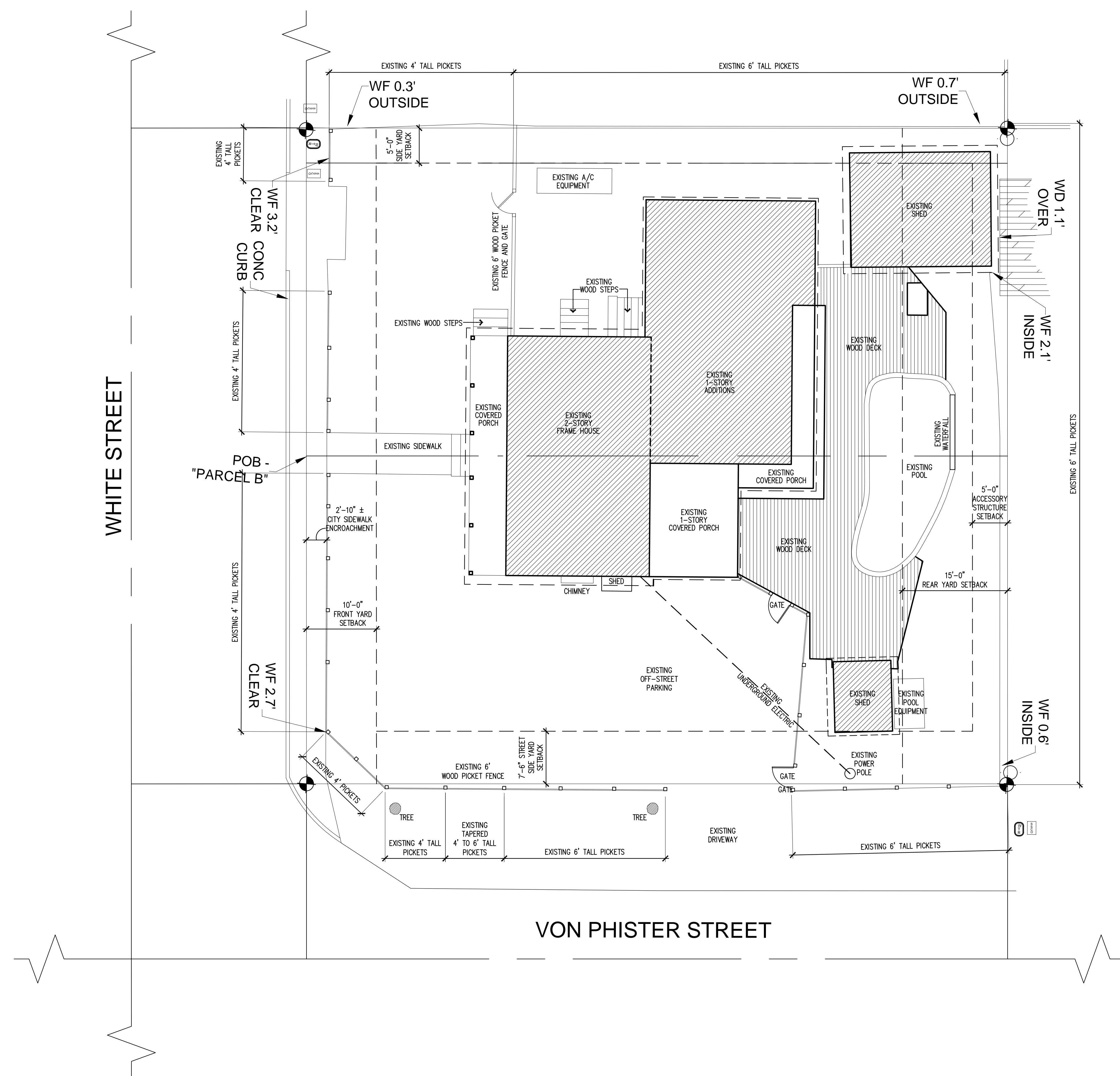
EXISTING SITE PLAN 1/8"=1'-0"
