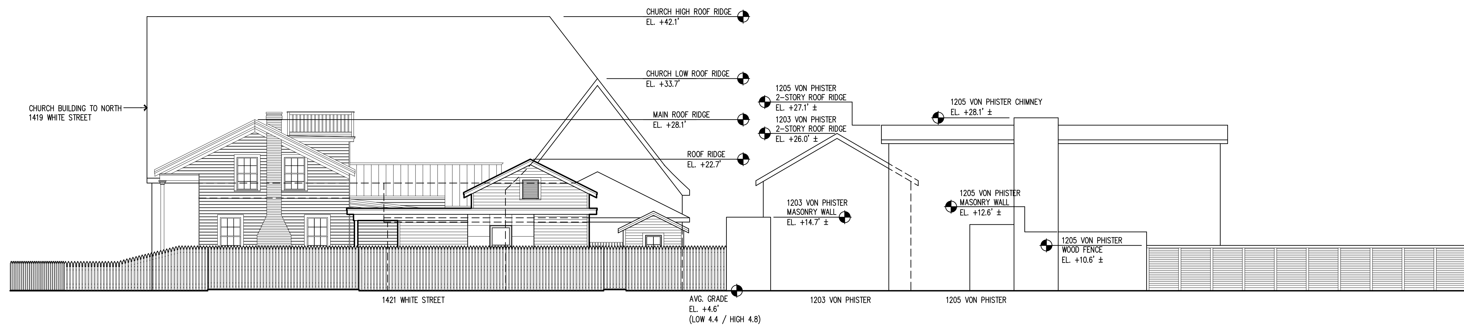
STREETSCAPE ELEVATION – VON PHISTER STREET 1/8"=1'-0"
