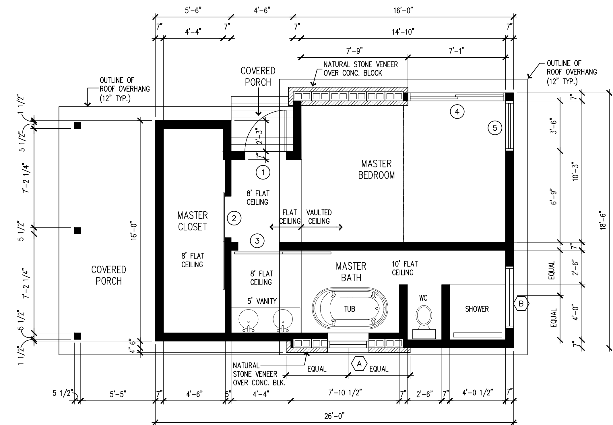
FLOOR PLAN 1/4"=1'-0"
