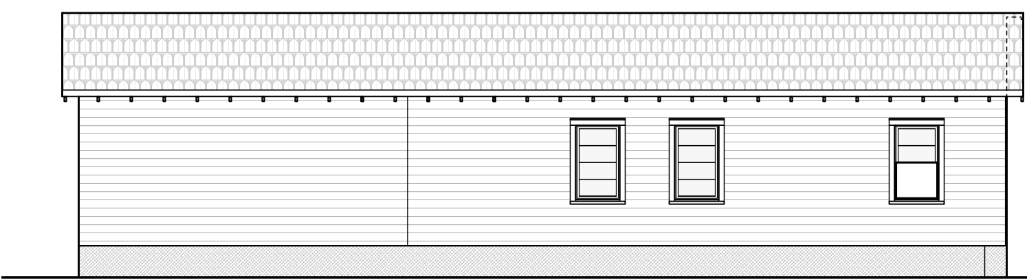
6 EX. ELEVATION - SIDE (EAST) D1.1 SCALE: 1/8" = 1'-0"
