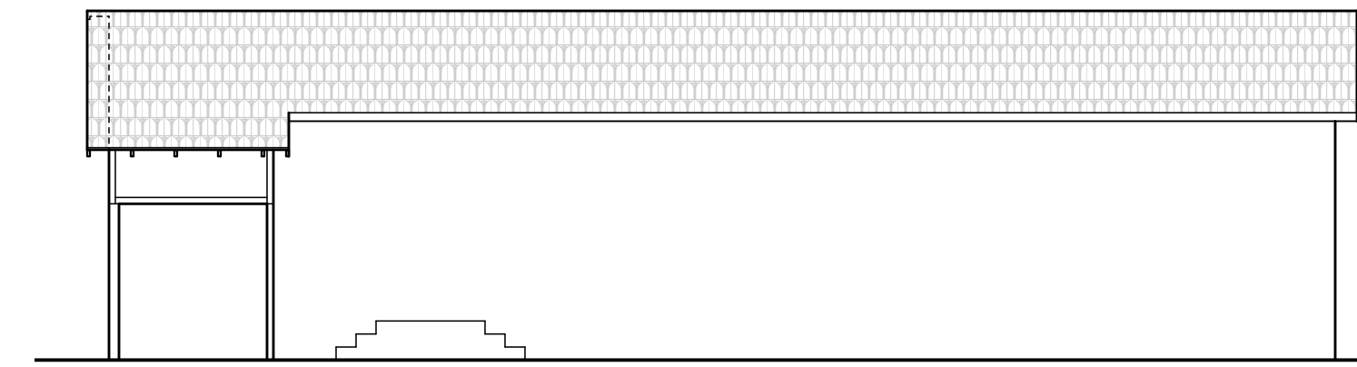
4 EX. ELEVATION - SIDE (WEST) D1.1 SCALE: 1/8" = 1'-0"
