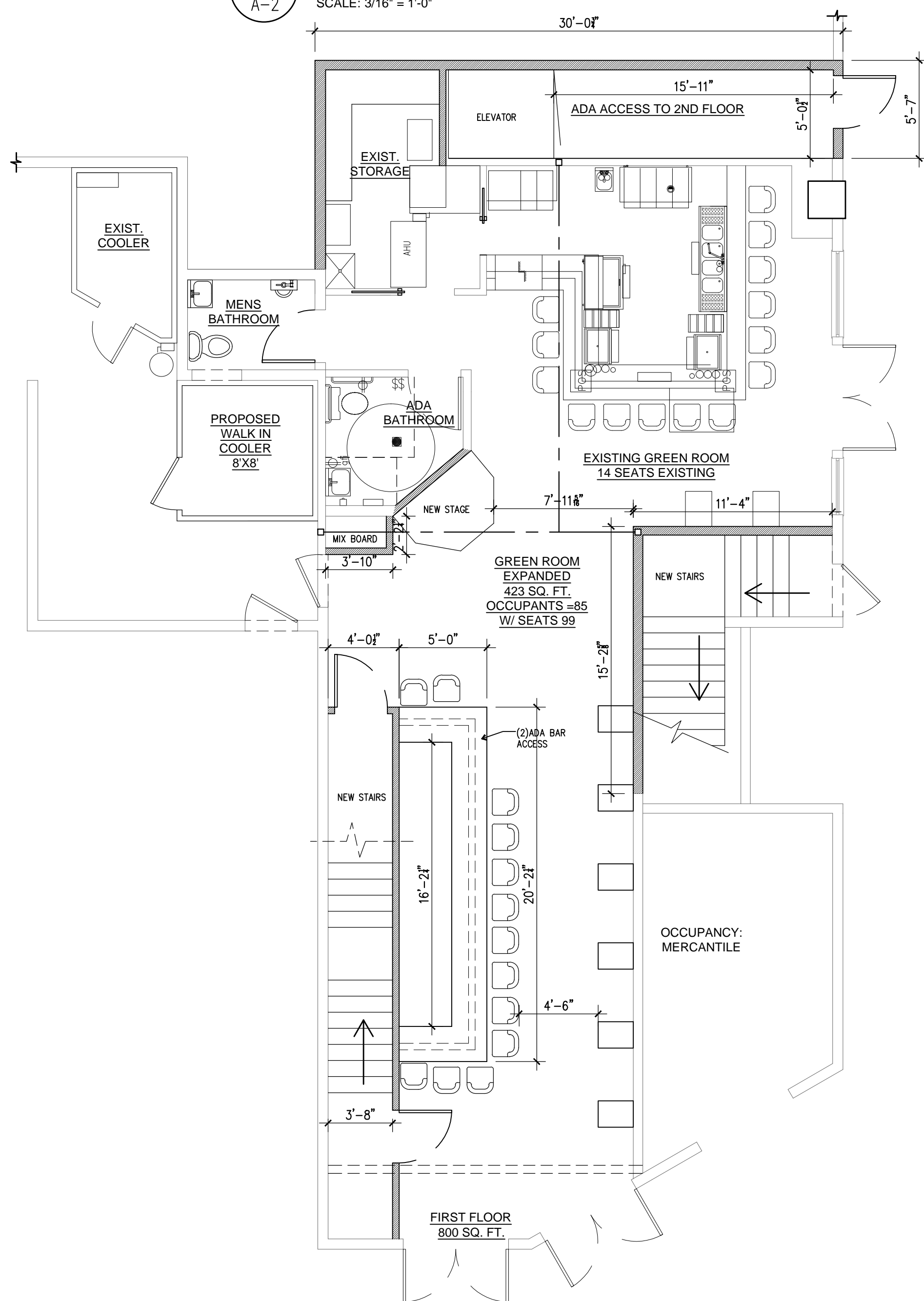
2 PROPOSED FIRST FLOOR PLAN SCALE: 3/16" = 1'-0"
