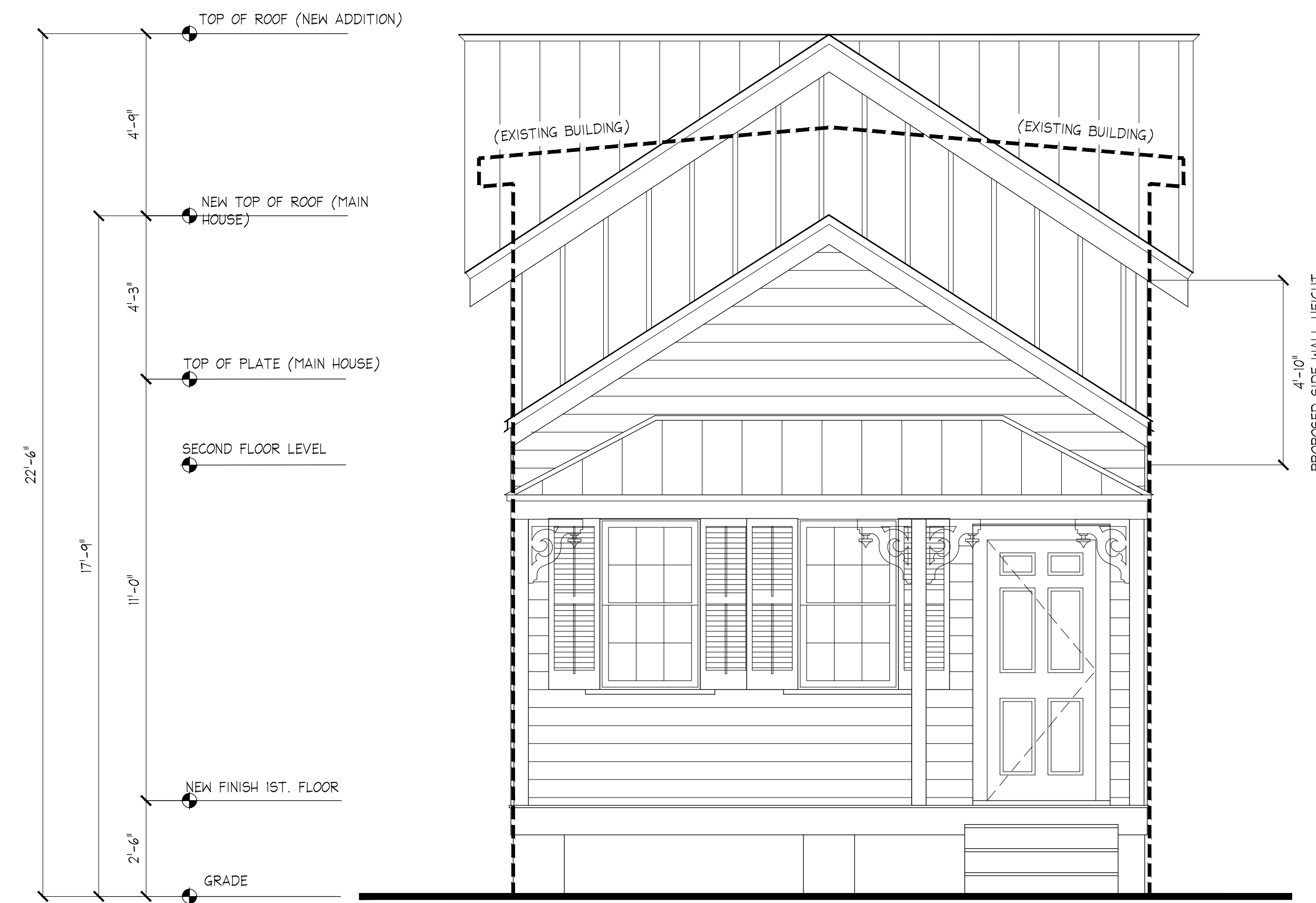
1 A6 PROPOSED EAST ELEVATION SCALE: 3/8" = 1'-0"
