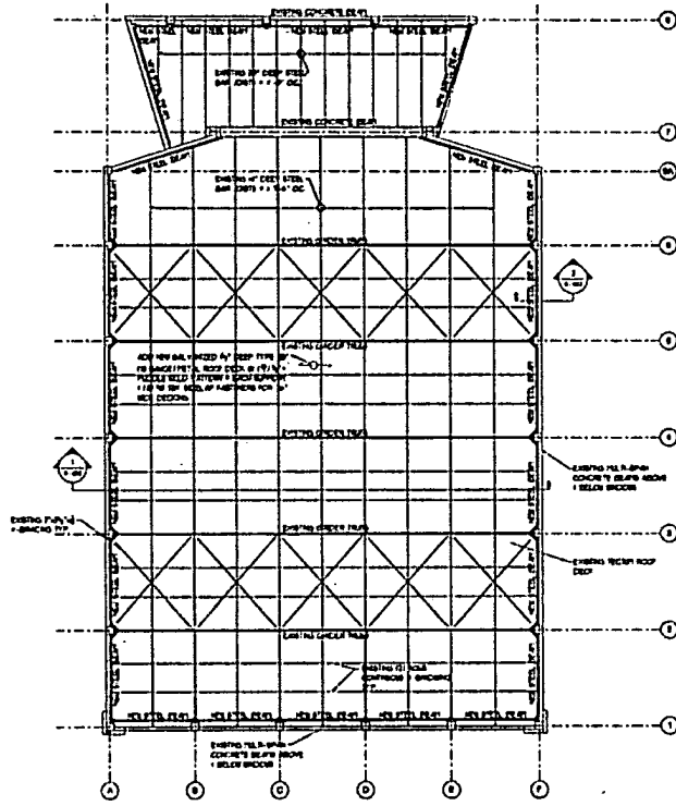
EXISTING ROOF FRAMING PLAN 1.1.1.12
