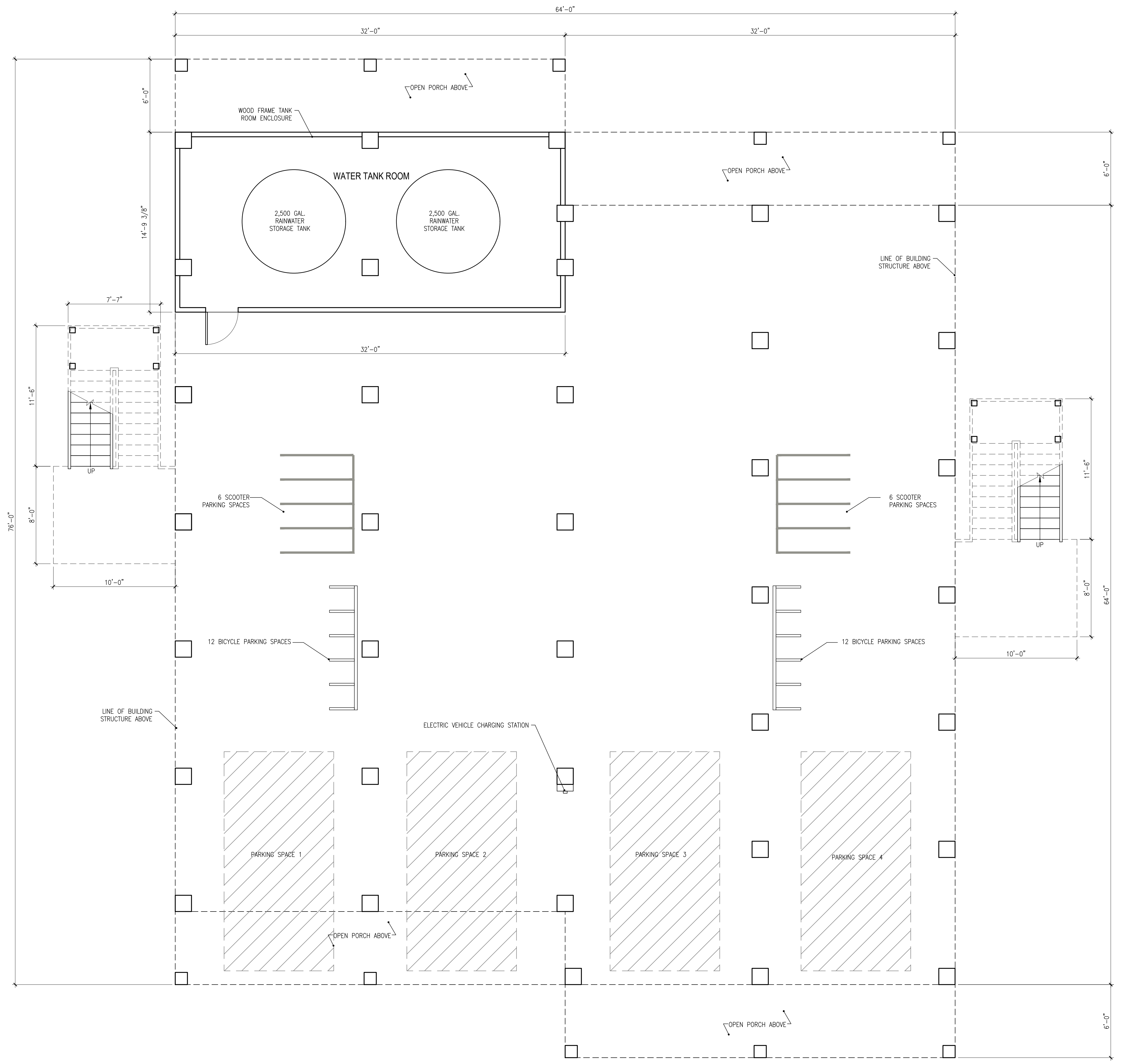
1 A2.0 TYPICAL GROUND FLOOR PLAN SCALE: 1/4"=1'-0"
