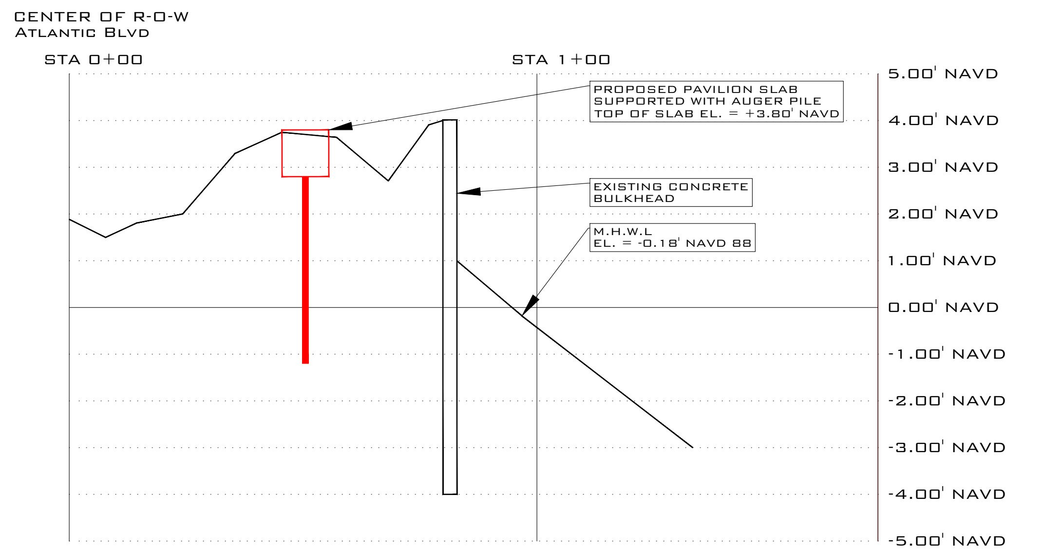
CUT/FILL PROFILE PAVILION "C" SCALE HORIZONTAL: 1" = 20'-0" SCALE VERTICAL: 1" = 2'-0"
