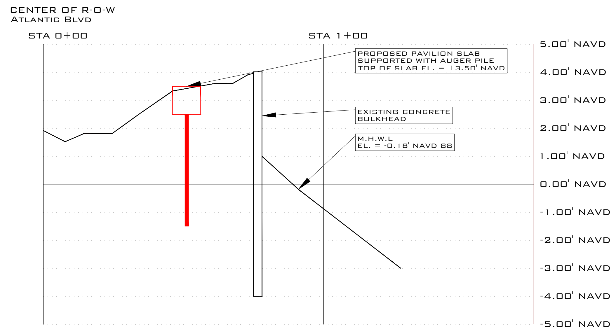
CUT/FILL PROFILE PAVILION "B" SCALE HORIZONTAL: 1" = 20'-0" SCALE VERTICAL: 1" = 2'-0"
