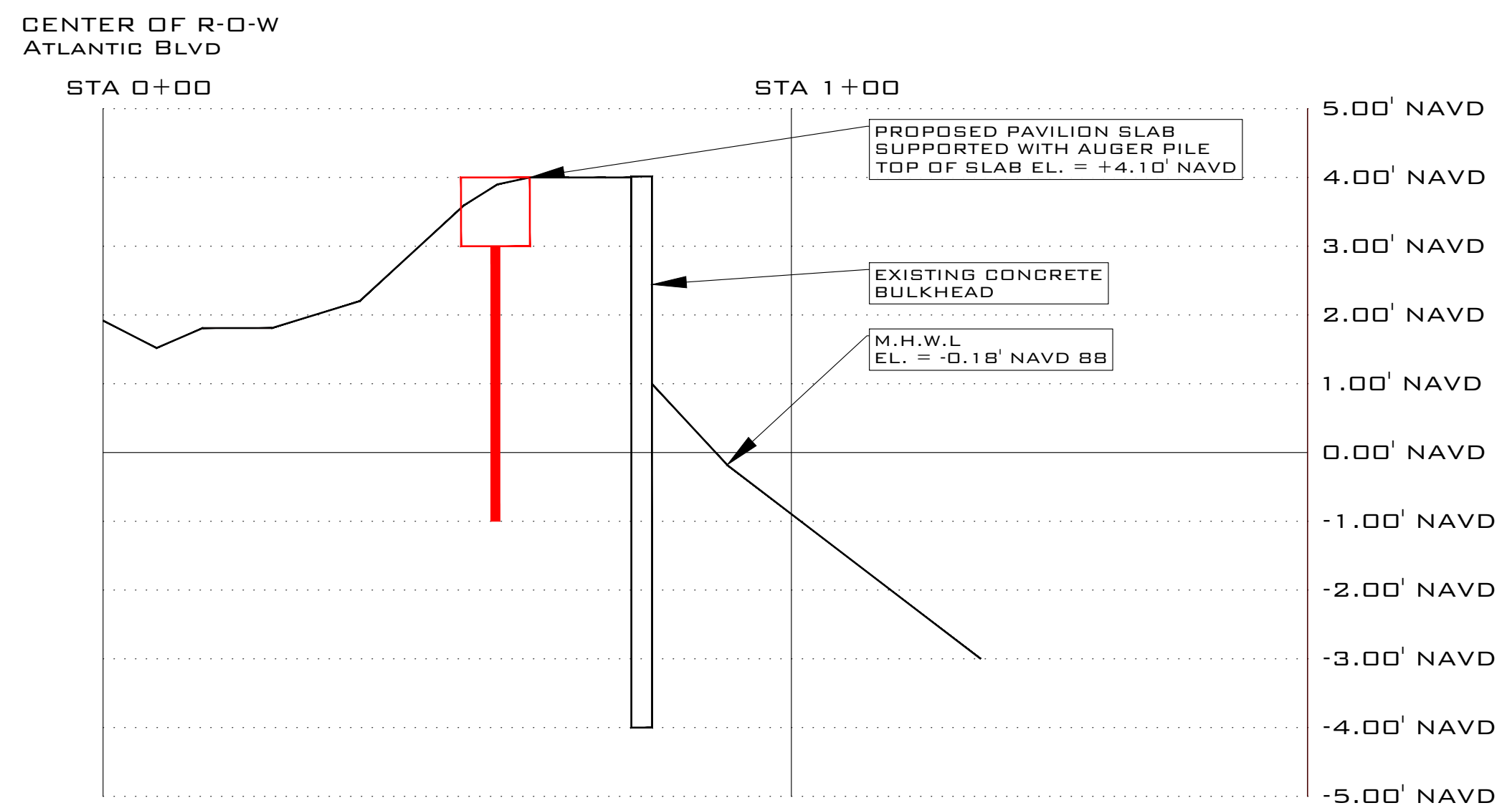
CUT/FILL PROFILE PAVILION "A" SCALE HORIZONTAL: 1" = 20'-0" SCALE VERTICAL: 1" = 2'-0"
