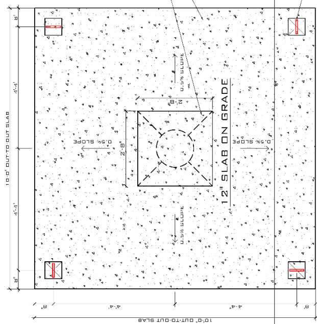
FOUNDATION PLAN SCALE: 1/2" = 1'-0"
